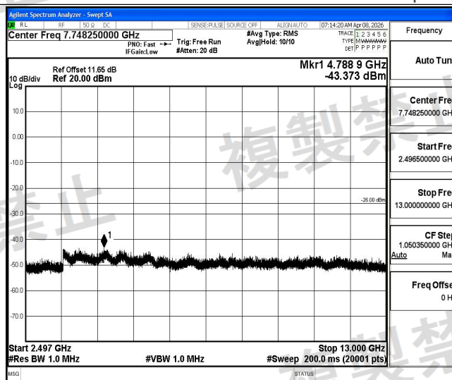
NTNV-3DH5-Ant1-2441-2496.5~13000-PASS
