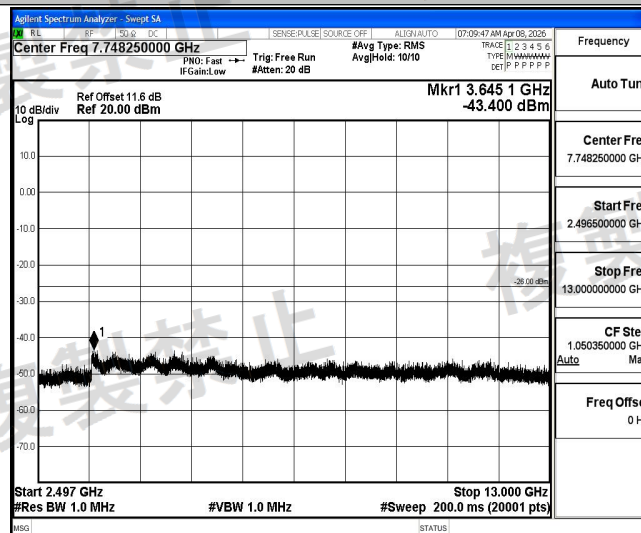
NTHV-2DH5-Ant1-2480-2496.5~13000-PASS
