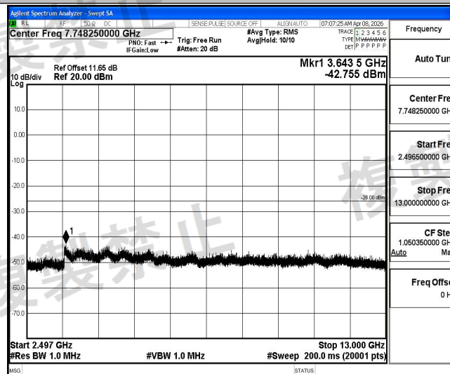
NTHV-2DH5-Ant1-2441-2496.5~13000-PASS
