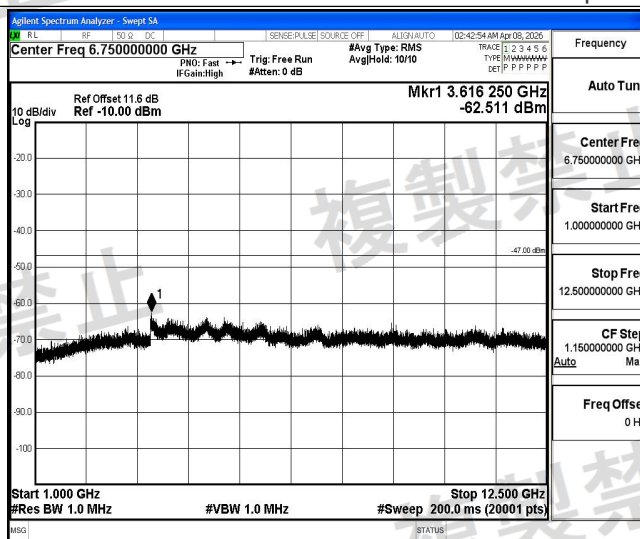
NTNV-DH5-Ant1-2480-1000~12500-PASS
