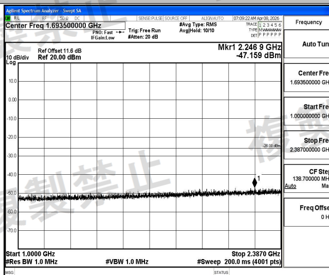
NTHV-2DH5-Ant1-2480-1000~2387-See table below
