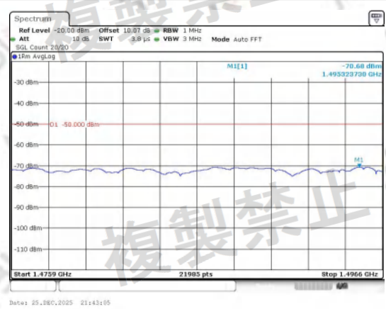
1475.9-1496.6_new Band 3 20MHz/1747.5/Mid QPSK 48@0
