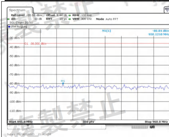
945.0-960.0_new Band 3 20MHz/1747.5/Mid QPSK 48@0
