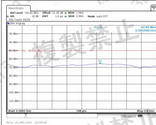
3590.3-3600.0_new Band 3 20MHz/1747.5/Mid QPSK 18@0
