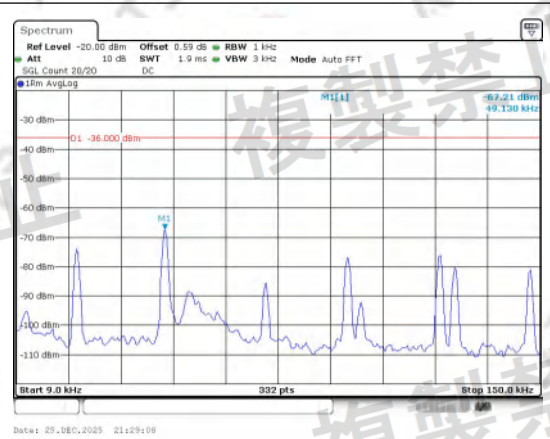
0.009-0.15_new Band 3 20MHz/1747.5/Mid QPSK 18@82
