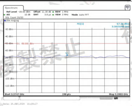
3574.7-3590.3_new Band 3 20MHz/1747.5/Mid QPSK 18@0
