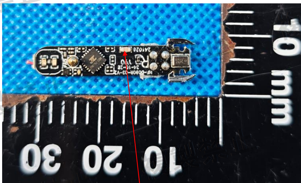
Chip Antenna
