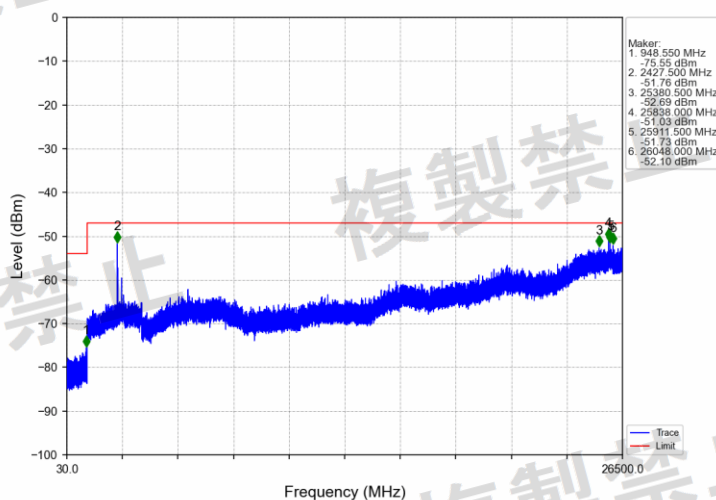
802.11ac(VHT20)_LCH_5180MHz_Ant1_NTNV
