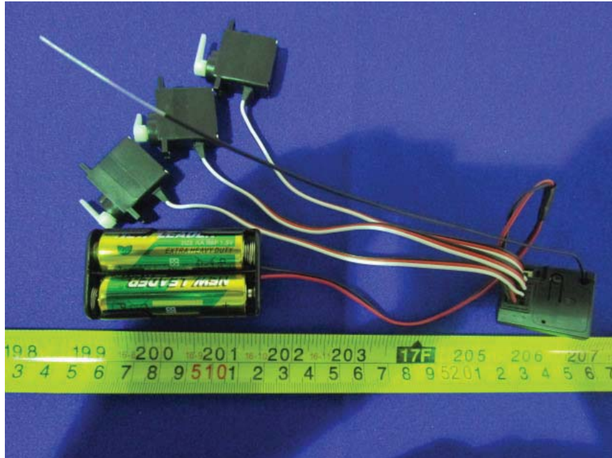
EUT and Servo View
