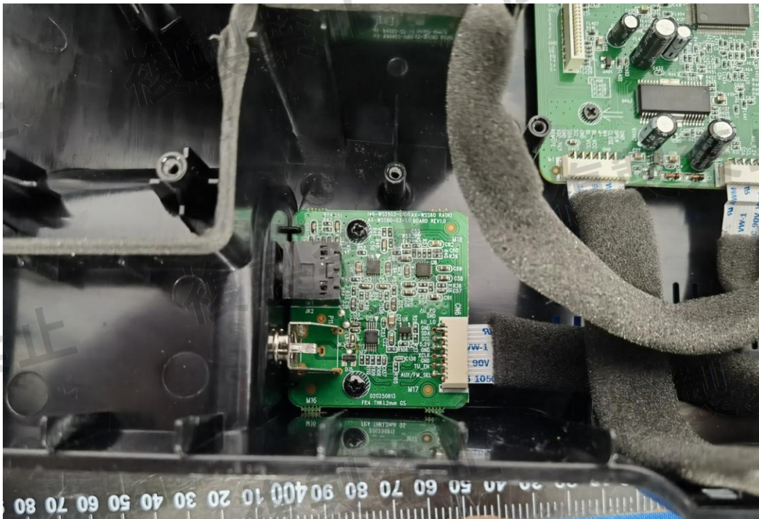
Figure 22 Inside of the EUT
