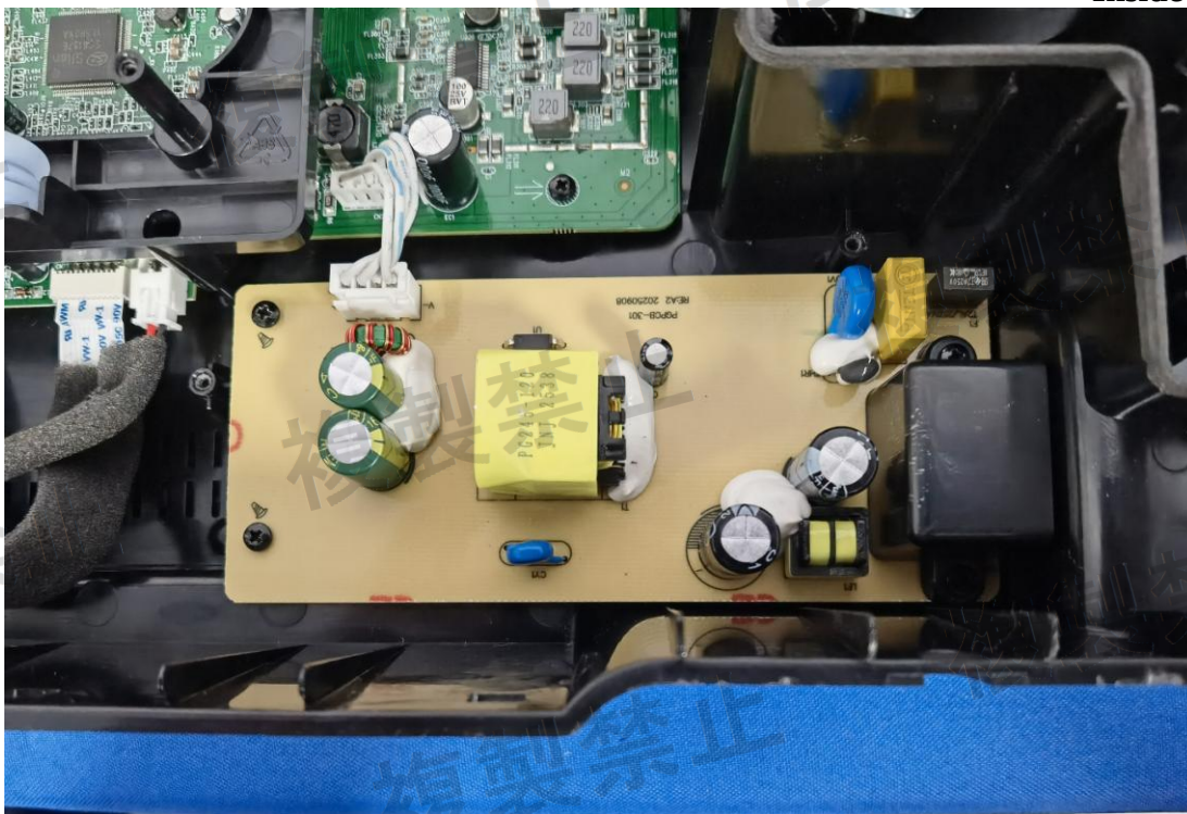
Figure 20 Inside of the EUT
