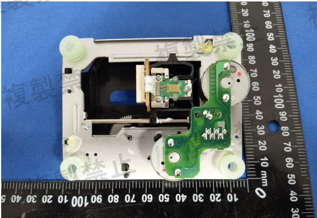
Figure 19 Inside of the EUT
