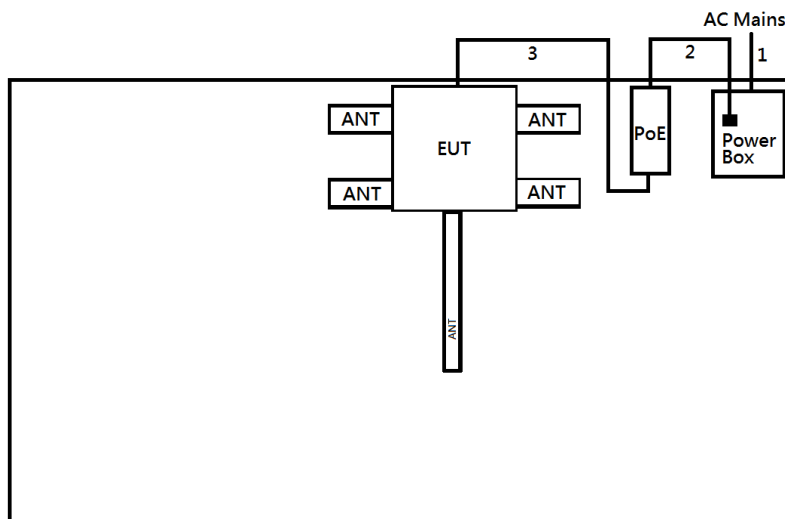
Test Setup Diagram – AC Line Conducted Emission Test (Sample 2) - TX
