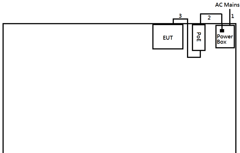
Test Setup Diagram – AC Line Conducted Emission Test (Sample 1) - TX
