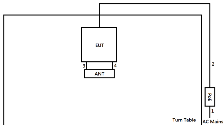
Test Setup Diagram - Radiated Test (Sample 2_Panel 2) - TX
