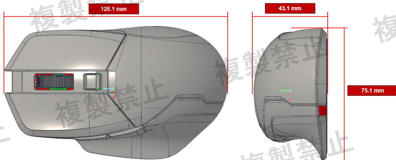
Mouse Dimension
