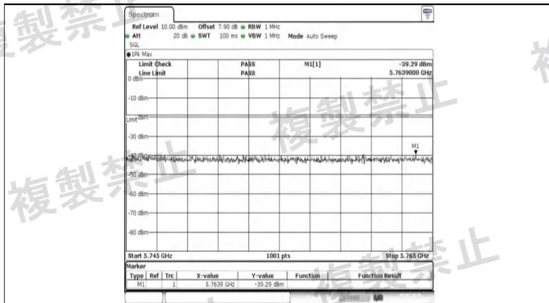
NTNV-11AC20SISO-Ant1-5500-5745~5765-PASS
