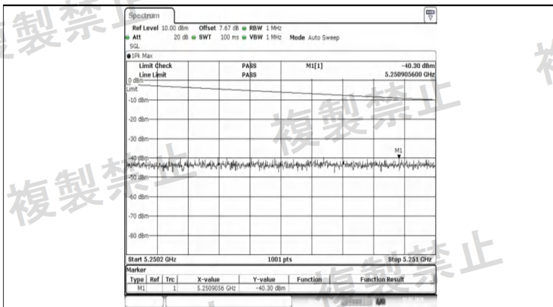
NTNV-11AX20SISO-Ant1-5180-5250.2~5251-PASS
