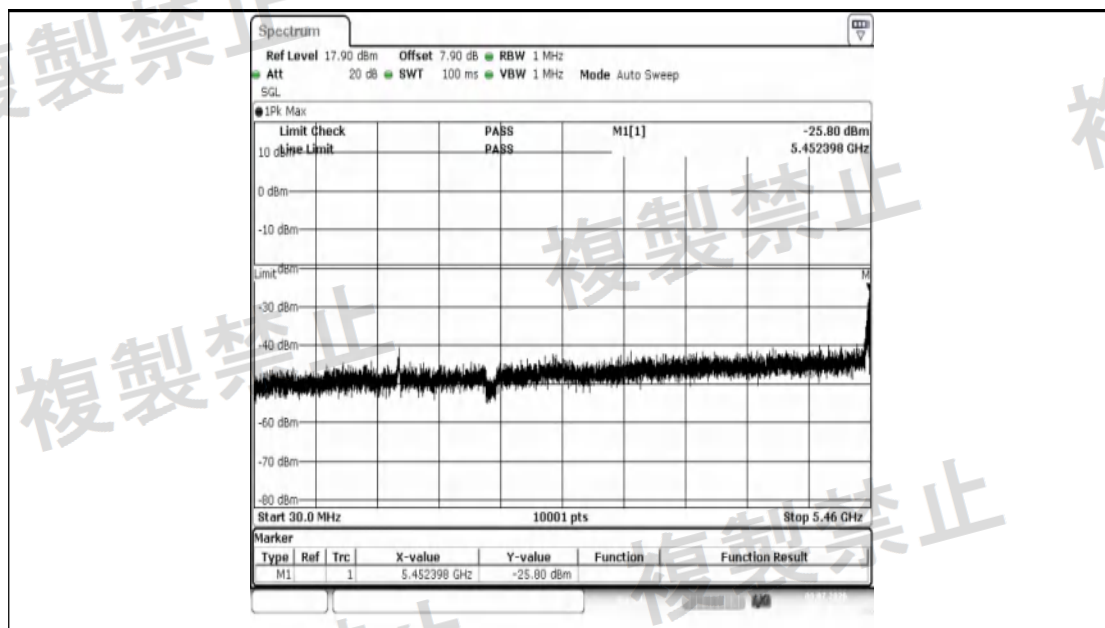
NTVN-11AX40SISO-Ant1-5510-30~5460-PASS
