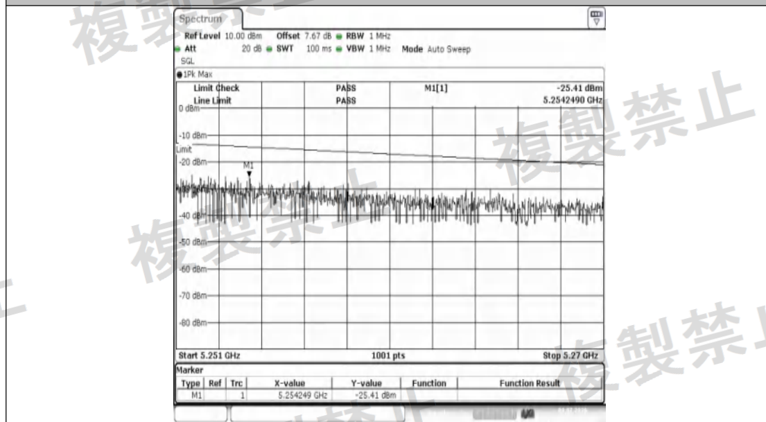
NTNV-11AX40SISO-Ant1-5190-5251~5270-PASS
