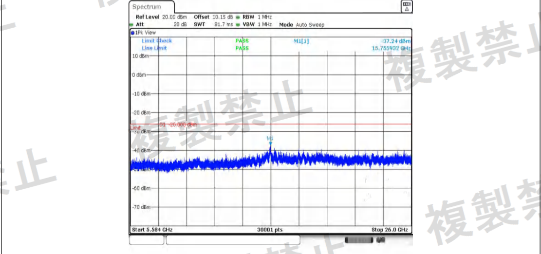
NTNV 11AC160MIMO Ant2 5250 5584~26000
