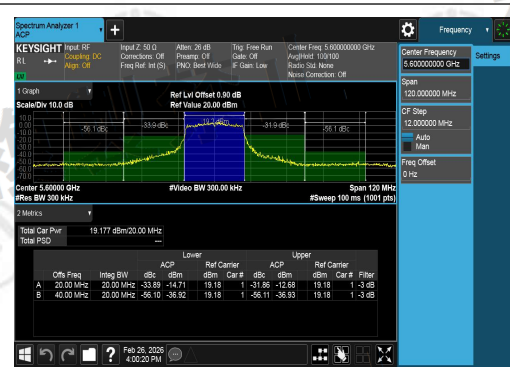
NNTV-11AX20SISO-Ant1-5600-PASS
