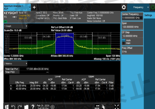
NTHV-11AC20SISO-Ant1-5500-PASS
