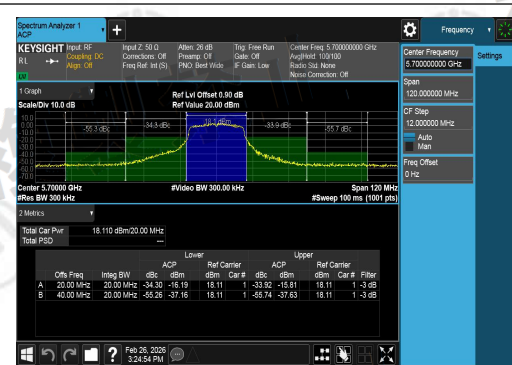
NTHV-11AC20SISO-Ant1-5700-PASS
