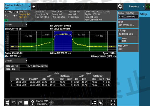
NTLV-11AX20SISO-Ant1-5700-PASS
