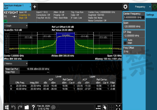
NTNV-11AC20SISO-Ant1-5600-PASS
