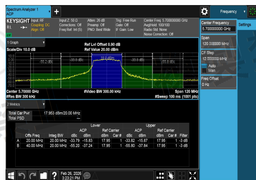
NTLV-11AC20SISO-Ant1-5700-PASS
