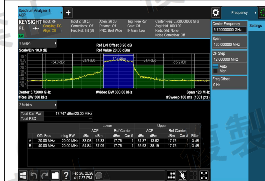
NTLV-11AX20SISO-Ant1-5720-PASS
