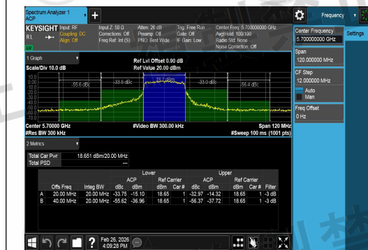
NNTV-11AX20SISO-Ant1-5700-PASS
