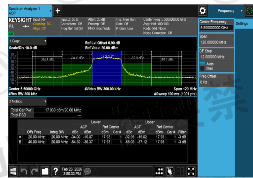
NTLV-11AX20SISO-Ant1-5500-PASS
