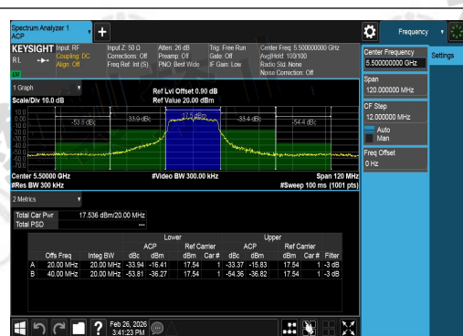
NTLV-11AC20SISO-Ant1-5500-PASS
