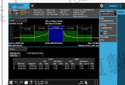
NTVN-11AX20SISO-Ant1-5500-PASS
