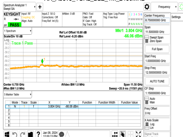
RX_Above_1GHz_BLE_1M_2480MHz
