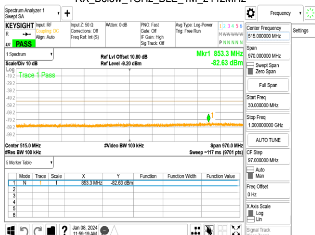
RX_Below_1GHz_BLE_1M_2480MHz
