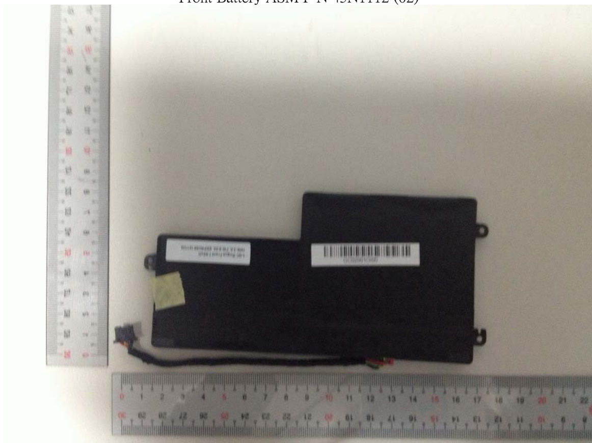
Front Battery ASM P-N 45N1112 (02)
