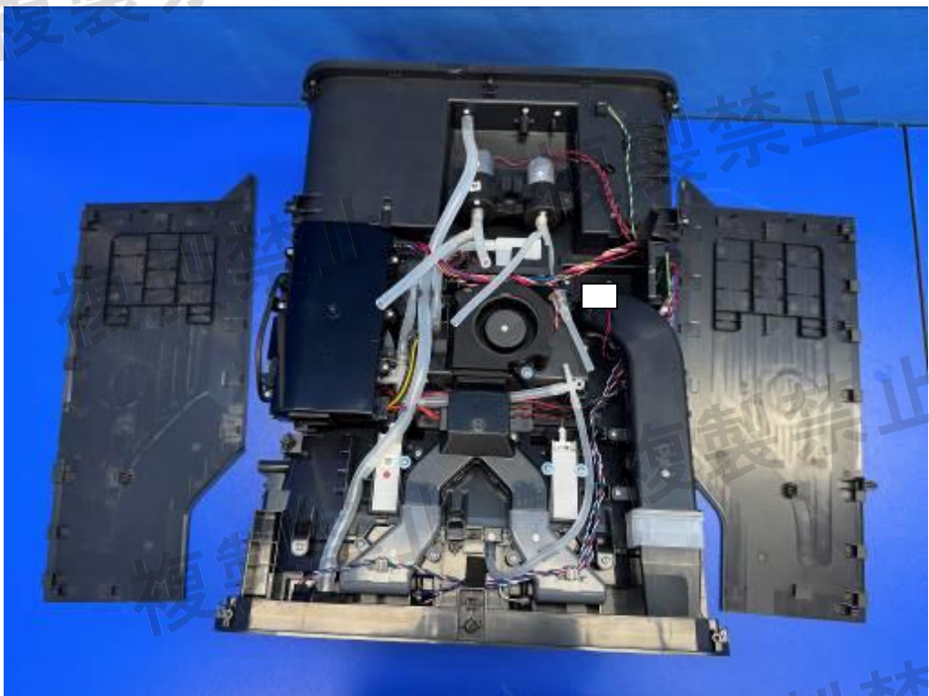
Figure 2. Internal view
