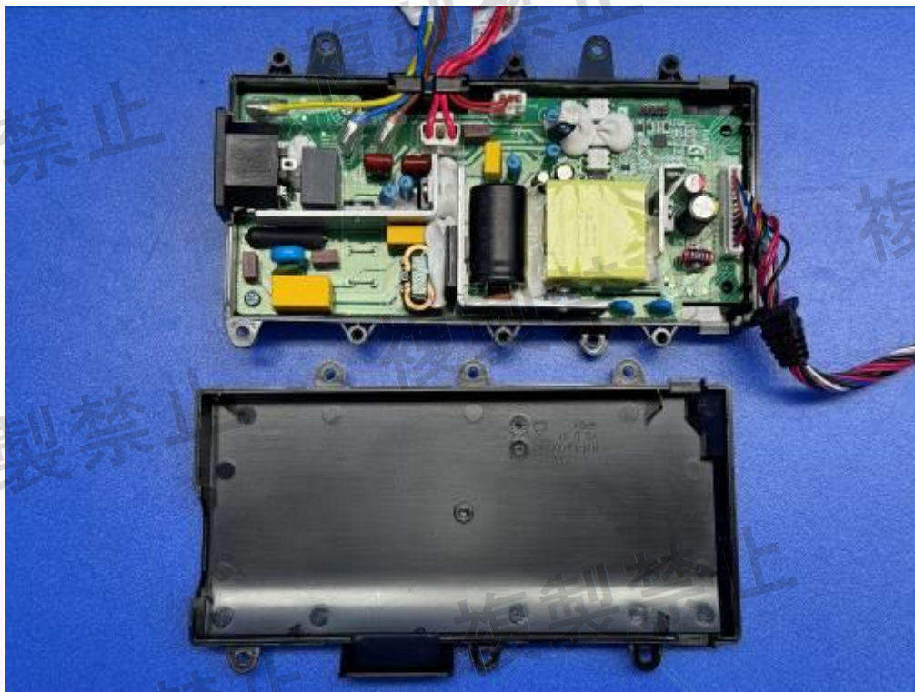
Figure 19. Built-in power supply
