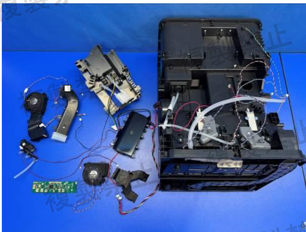
Figure 8. Internal view
