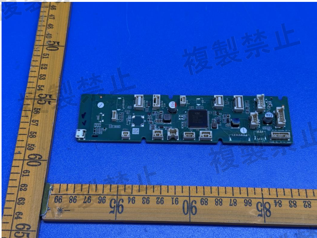
Figure 24. Control PCB
