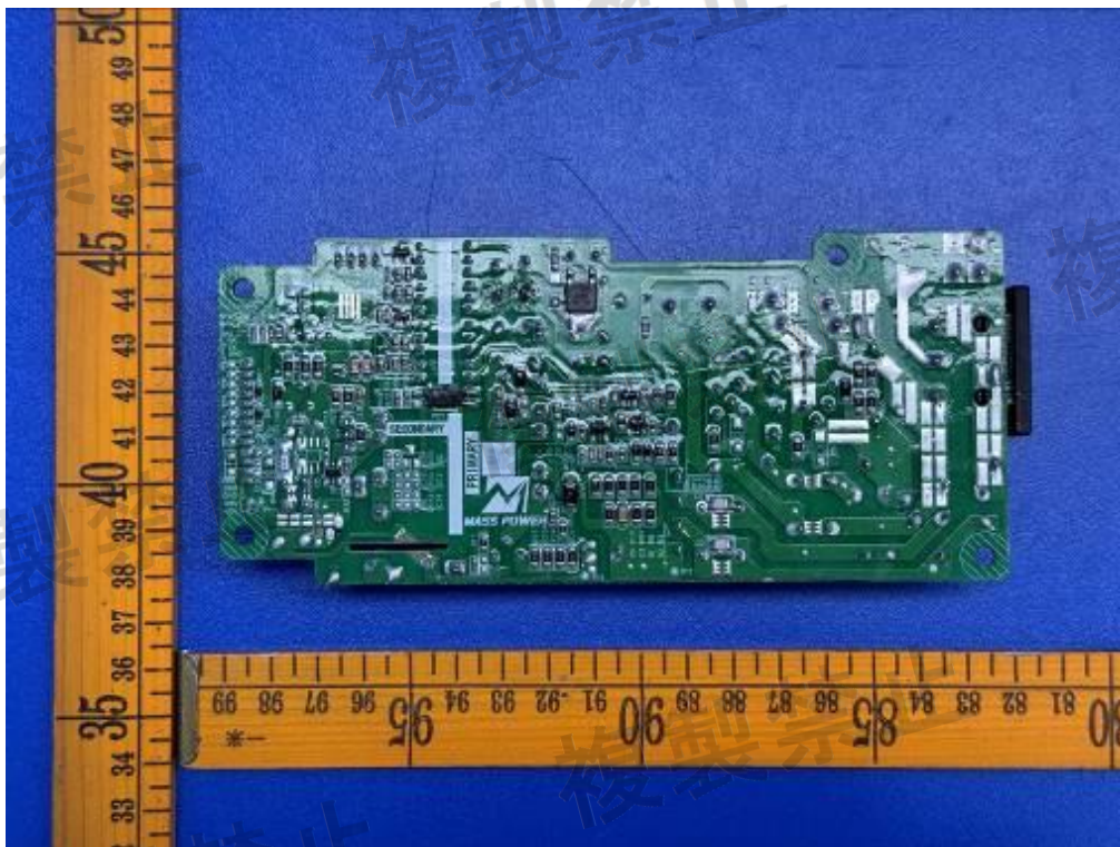
Figure 21. Built-in power supply
