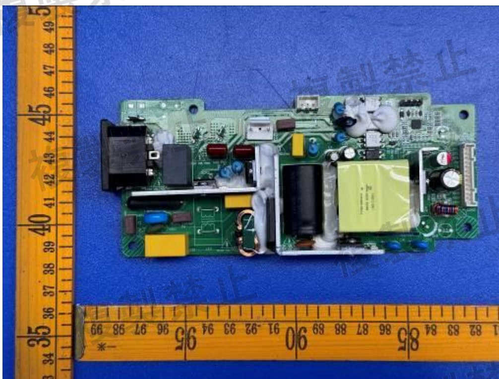
Figure 20. Built-in power supply
