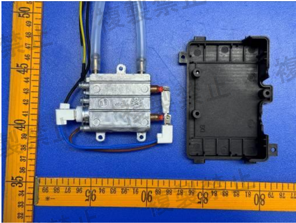
Figure 17. Water heater
