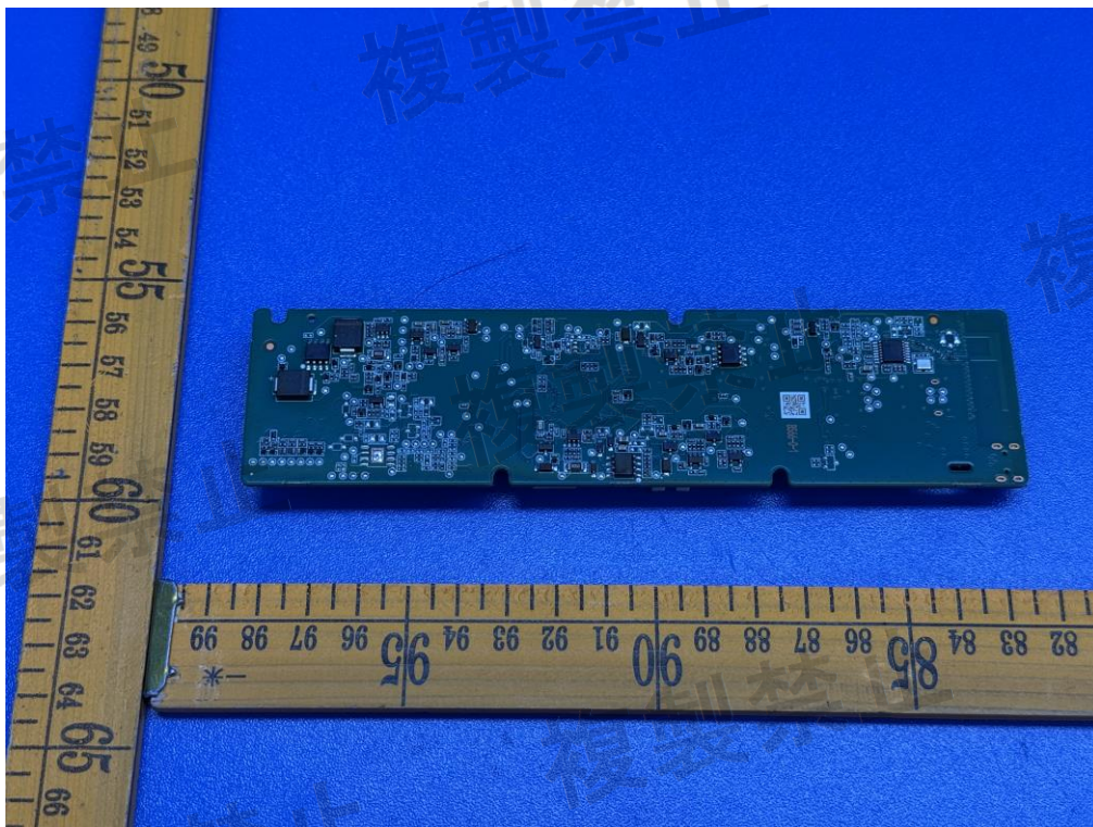
Figure 25. Control PCB
