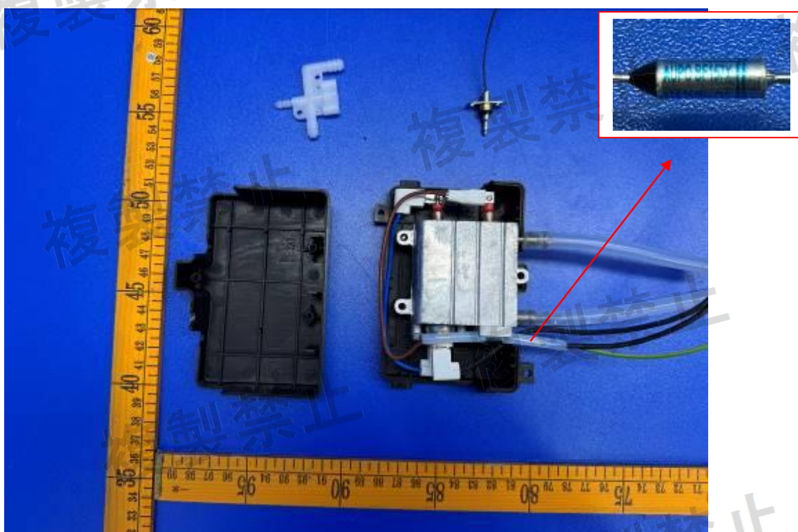
Figure 16. Water heater
