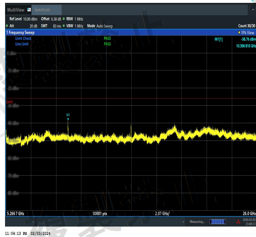
NTNV-11N20SISO-Ant3-5200-5266.7~26000-PA SS
