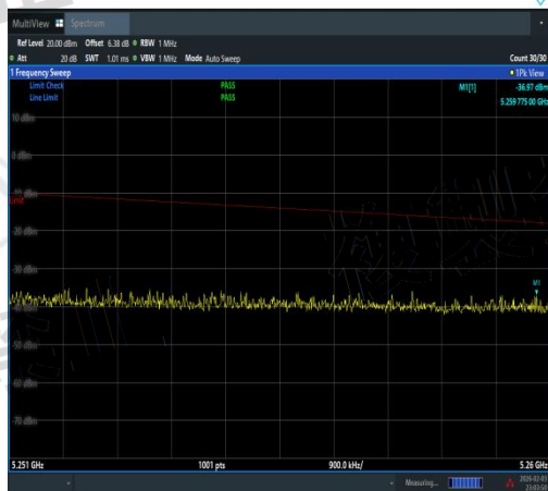
NTNV-11N20SISO-Ant3-5200-5251~5260-PASS
