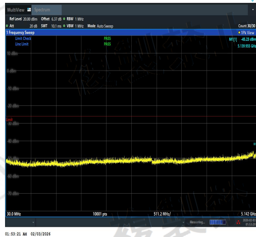
NTNV-11N20SISO-Ant2-5220-30~5142-PASS
