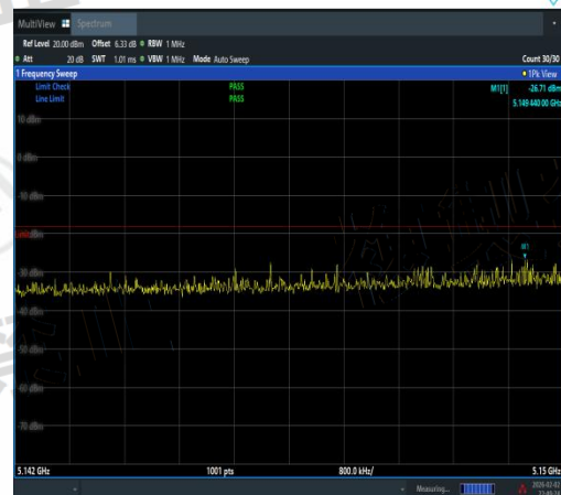
NTNV-11N20SISO-Ant1-5180-5142~5150-PASS
