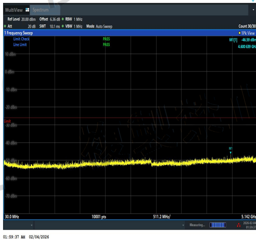
NTVN-11N20MIMO-Ant1-5220-30~5142-PASS
