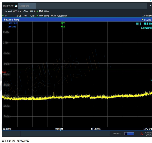
NTNV-11N20SISO-Ant1-5200-30~5142-PASS
