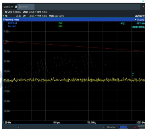
NTNV-11N20SISO-Ant1-5200-5250~5251-PASS
