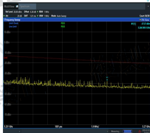
NTVN-11N40SISO-Ant3-5190-5251~5270-PASS
