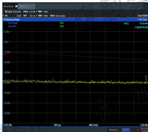
NTNV-11N20SISO-Ant2-5200-5251~5260-PASS
