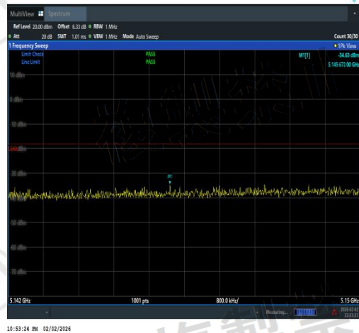
NTNV-11N20SISO-Ant1-5200-5142~5150-PASS
