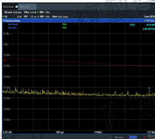
NTVN-11N40SISO-Ant2-5190-5251~5270-PASS
