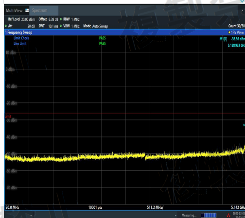
NTNV-11N20SISO-Ant3-5180-30~5142-PASS
