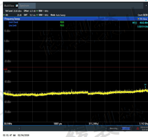
NTVN-11N20MIMO-Ant2-5220-30~5142-PASS
