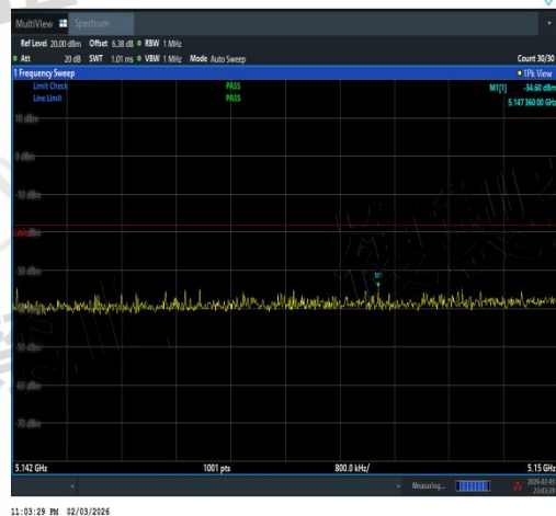
NTNV-11N20SISO-Ant3-5200-5142~5150-PASS
