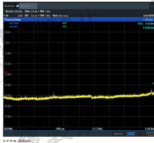
NTNV-11N20SISO-Ant2-5200-30~5142-PASS
