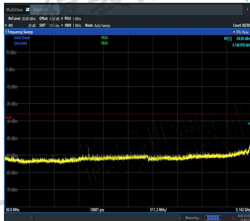
NTNV-11N20SISO-Ant1-5180-30~5142-PASS
