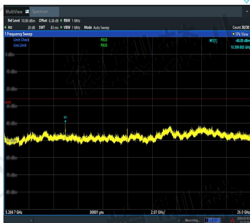
NTNV-11A-Ant3-5200-5266.7~26000-PASS
