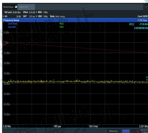
NTNV-11N20SISO-Ant2-5200-5250~5251-PASS
