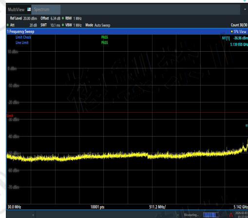
NTNV-11N20SISO-Ant2-5180-30~5142-PASS
