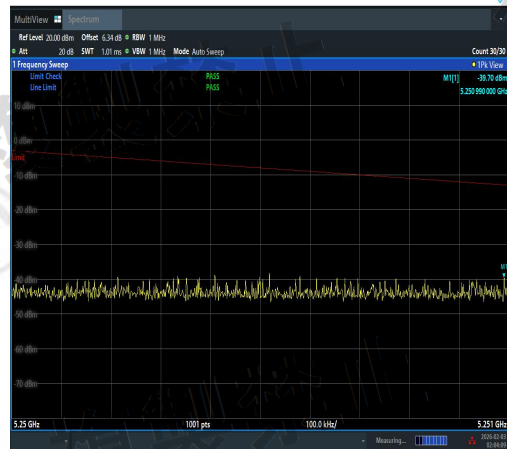
NTVN-11N40SISO-Ant2-5190-5250~5251-PASS
