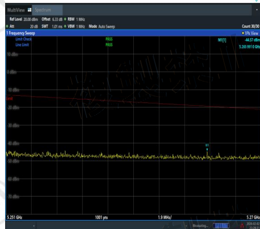
NTVN-11N40SISO-Ant1-5190-5251~5270-PASS
