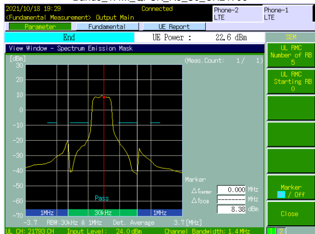
Band8_1.4M_QPSK_R5_S0_CH21793
