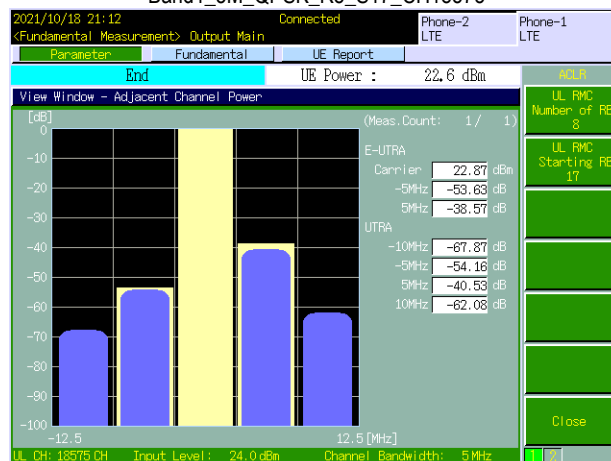
Band1 5M QPSK R8 S17 CH18575
