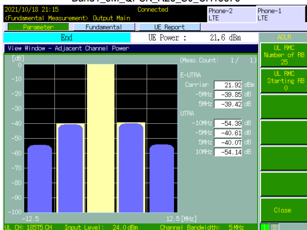
Band1_5M_QPSK_R25_S0_CH18575
