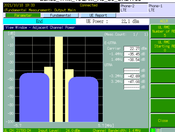
Band8_1.4M_16QAM_R5_S0_CH21793
