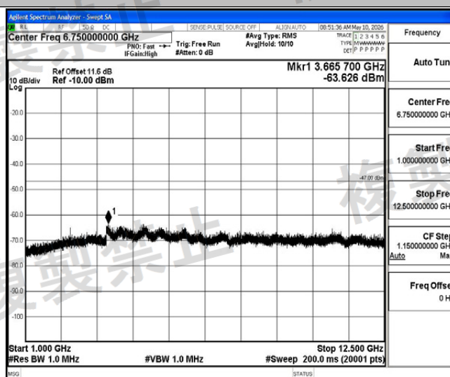
NTHV-DH5-Ant1-2480-1000~12500-PASS
