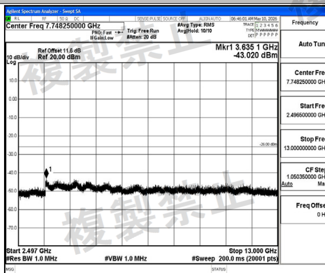
NTHV-3DH5-Ant1-2480-2496.5~13000-PASS
