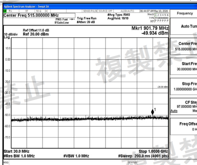
NTHV-3DH5-Ant1-2480-30~1000-PASS
