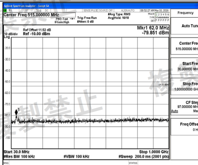
NTHV-2DH5-Ant1-2402-30~1000-PASS
