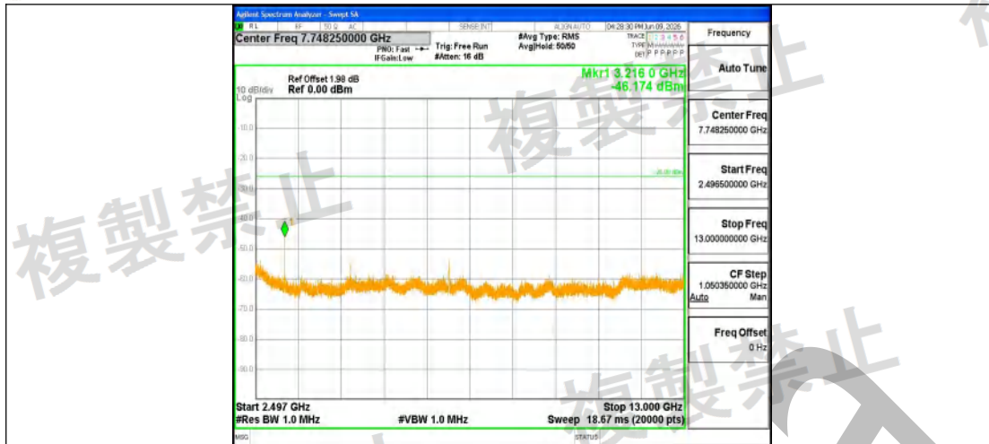
NTNV-11B-Ant1-2412-2496.5~13000-PASS
