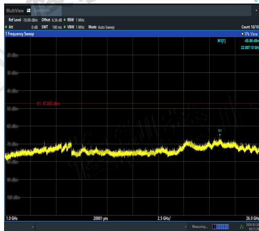
NTNV-11AX40SISO-Ant1-5710-1000~26000-PA SS
