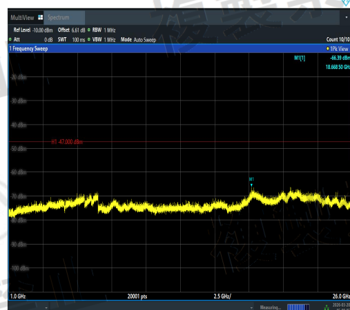
NTVN-11AX20MIMO-Ant3-5500-1000~26000-PA SS
