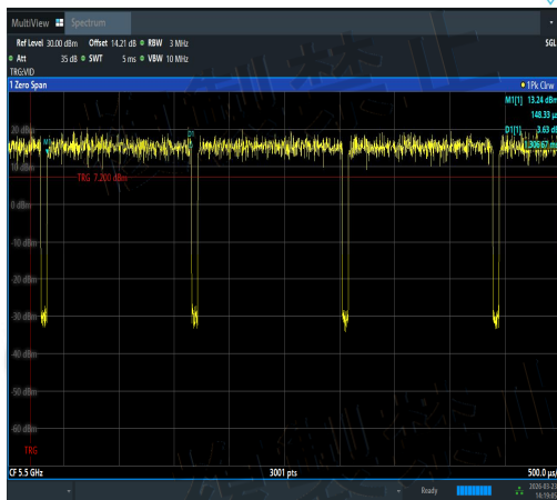
NTNV-11N20SISO-Ant3-5500-PASS
