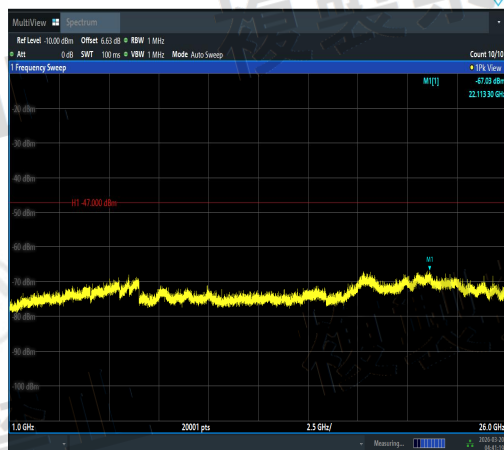
NTNV-11AX40SISO-Ant3-5710-1000~26000-PA SS
