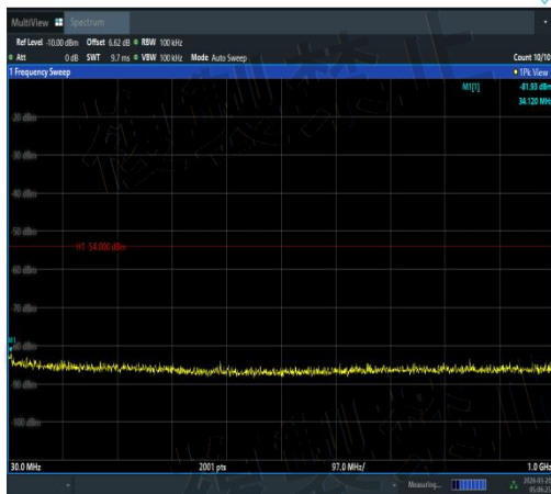
NTNV-11AC80MIMO-Ant3-5690-30~1000-PASS
