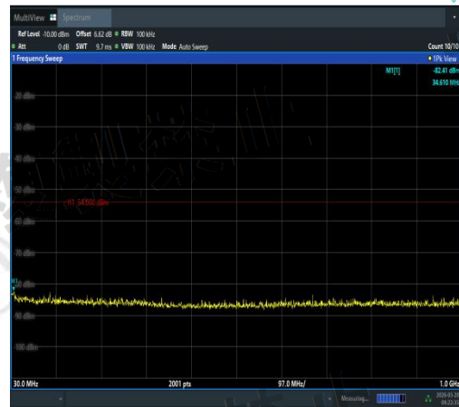
NTNV-11AC80SISO-Ant2-5690-30~1000-PASS
