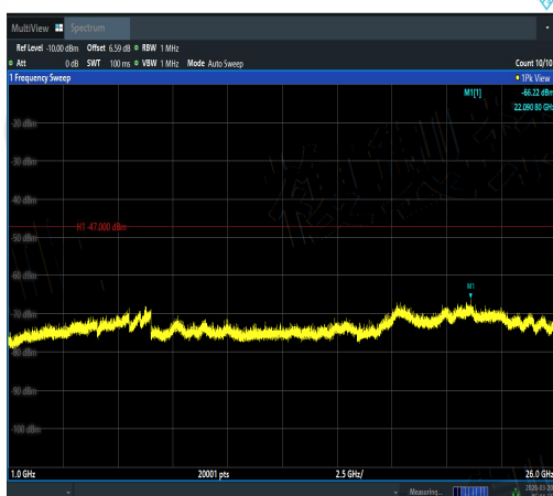
NTNV-11AC80MIMO-Ant2-5610-1000~26000-PA SS
