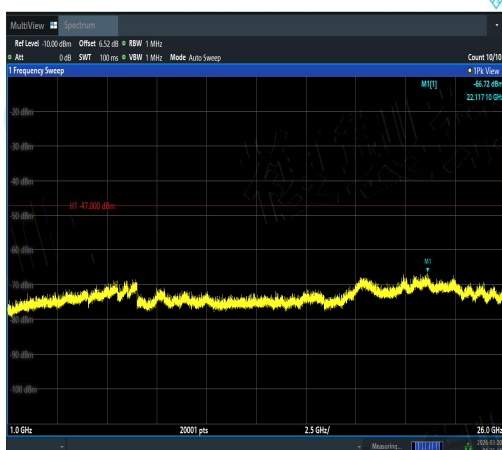
NTNV-11AX40SISO-Ant2-5510-1000~26000-PA SS
