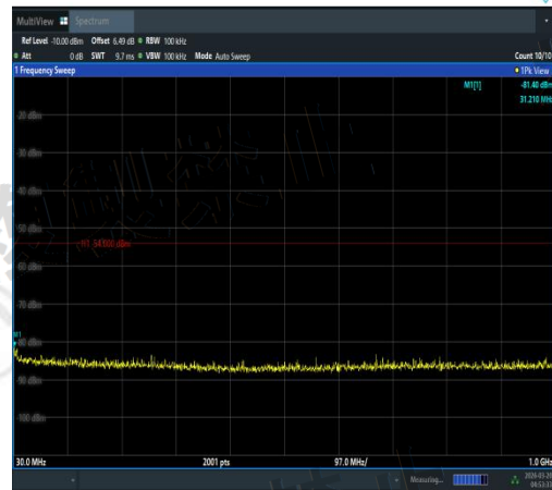
NTVN-11AC20MIMO-Ant2-5500-30~1000-PASS
