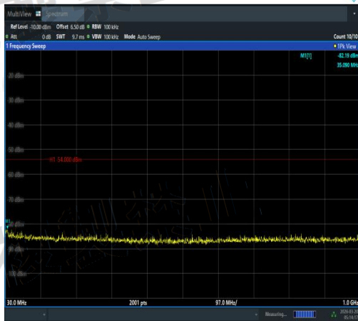
NTVN-11AX40MIMO-Ant1-5550-30~1000-PASS
