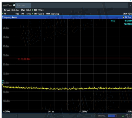
NTNV-11AC20MIMO-Ant3-5600-30~1000-PASS
