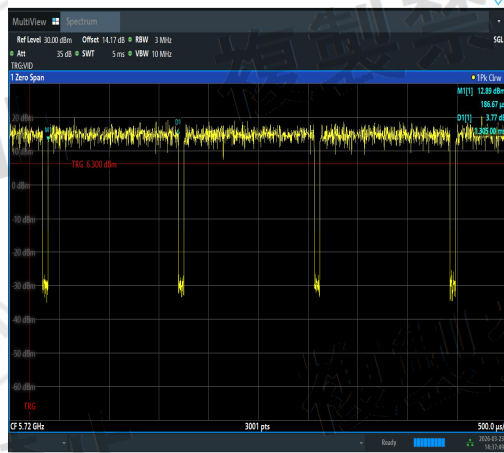
NTNV-11N20SISO-Ant3-5720-PASS
