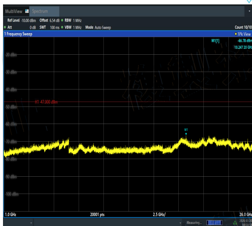
NTNV-11AC20MIMO-Ant2-5600-1000~26000-PA SS
