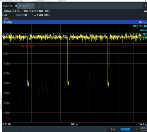
NTVN-11AC20SISO-Ant1-5500-PASS
