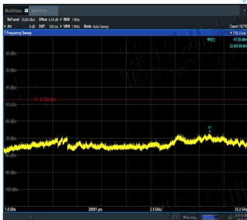
NTVN-11AC160MIMO-Ant2-5570-1000~26000-P ASS
