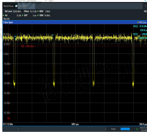
NTNV-11N20SISO-Ant1-5720-PASS
