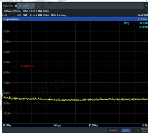
NTVN-11AX20MIMO-Ant1-5600-30~1000-PASS
