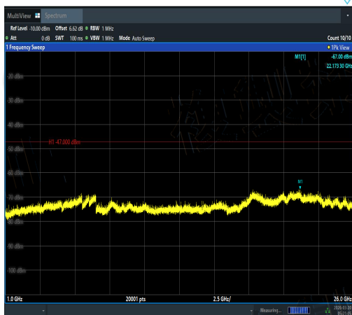
NTVN-11AX80MIMO-Ant2-5690-1000~26000-PA SS
