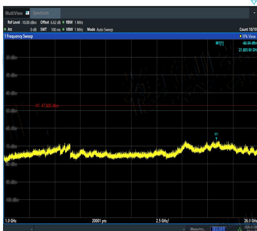
NTNV-11AC80SISO-Ant2-5690-1000~26000-PA SS
