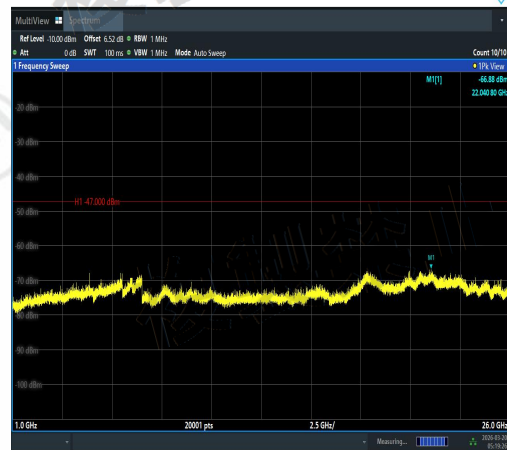
NTVN-11AX80MIMO-Ant1-5610-1000~26000-PA SS
