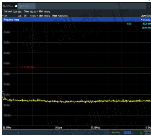
NTNV-11AC80SISO-Ant3-5690-30~1000-PASS
