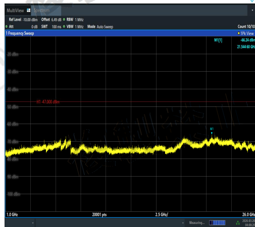
NTVN-11AC160SISO-Ant1-5570-1000~26000-PASS
