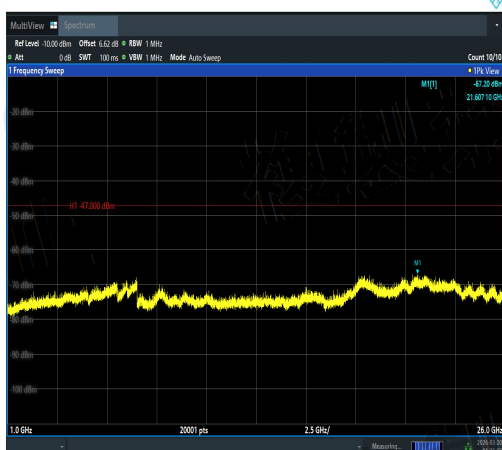
NTVN-11AX40SISO-Ant2-5670-1000~26000-PA SS
