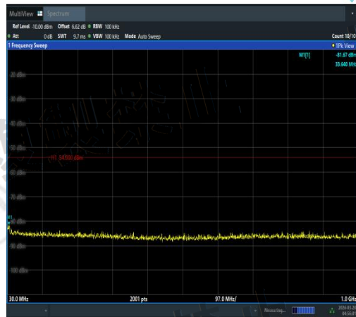
NTNV-11AC20MIMO-Ant2-5700-30~1000-PASS
