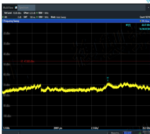
NTNV-11AX80SISO-Ant2-5530-1000~26000-PA SS
