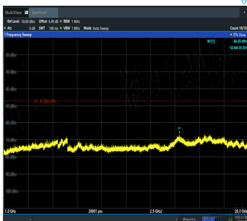
NTVN-11AC20MIMO-Ant2-5500-1000~26000-PA SS
