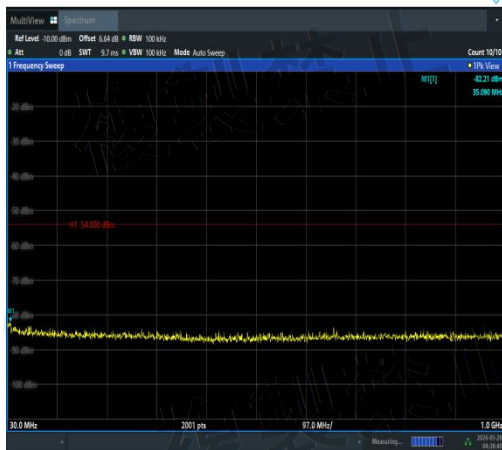
NTNV-11AX20SISO-Ant3-5600-30~1000-PASS
