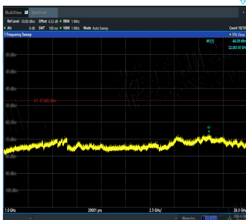
NTVN-11AX40MIMO-Ant2-5550-1000~26000-PA SS
