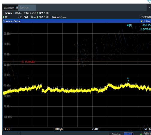
NTNV-11AC40SISO-Ant2-5550-1000~26000-PA SS
