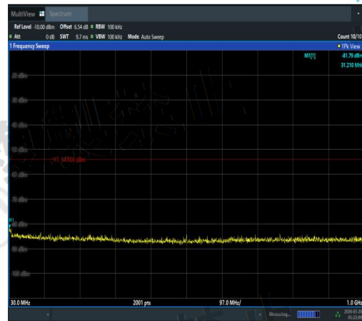
NTVN-11AX160MIMO-Ant2-5570-30~1000-PAS S
