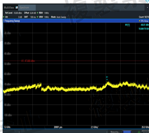
NTVN-11AX20MIMO-Ant3-5600-1000~26000-PA SS
