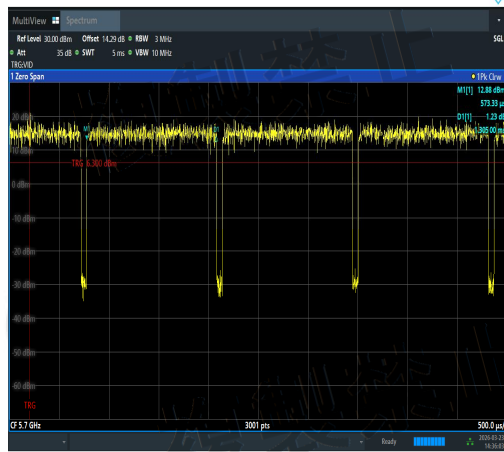
NTNV-11N20SISO-Ant3-5700-PASS
