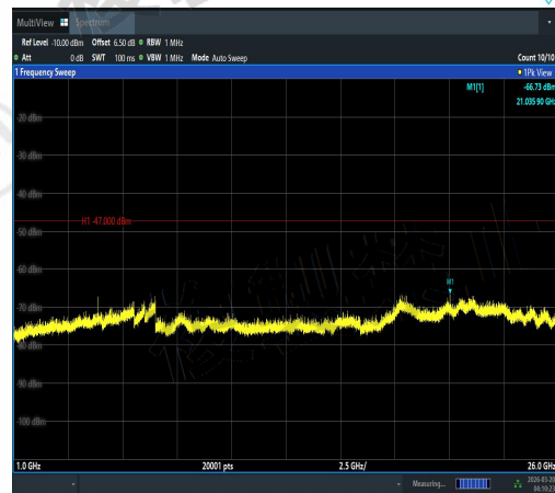
NTNV-11AX40SISO-Ant1-5510-1000~26000-PA SS
