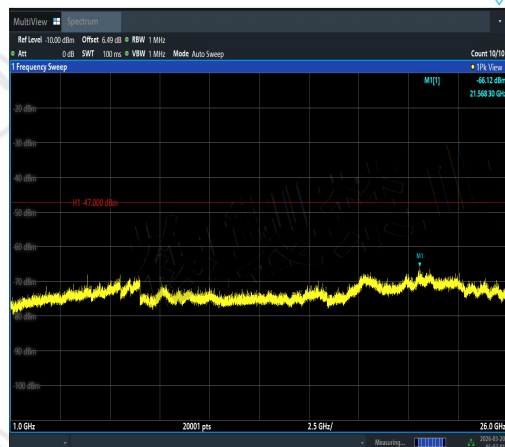
NTVN-11AC160MIMO-Ant1-5570-1000~26000-P ASS
