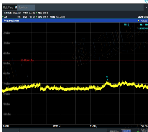
NTVN-11AC160SISO-Ant2-5570-1000~26000-PASS
