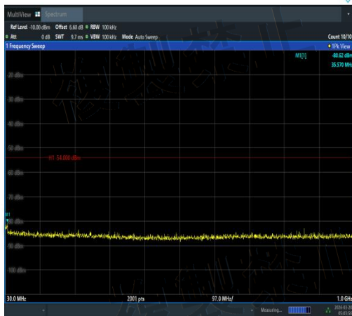
NTNV-11AC80MIMO-Ant3-5530-30~1000-PASS
