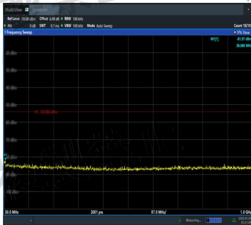
NTVN-11AX160MIMO-Ant1-5570-30~1000-PAS S
