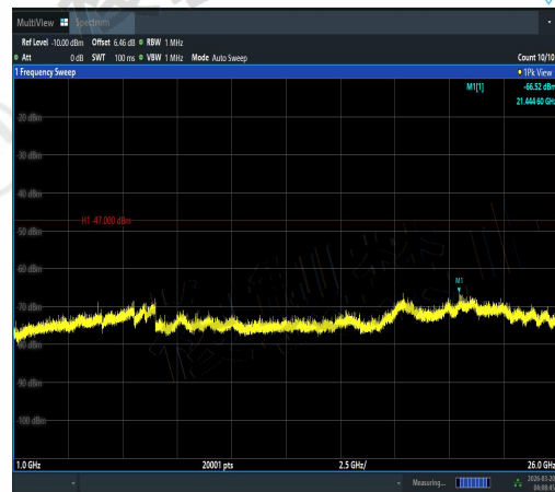
NTVN-11AX20SISO-Ant1-5500-1000~26000-PA SS
