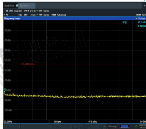
NTVN-11AX20SISO-Ant2-5500-30~1000-PASS
