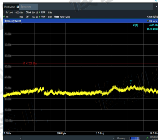
NTVN-11AC160MIMO-Ant3-5570-1000~26000-P ASS
