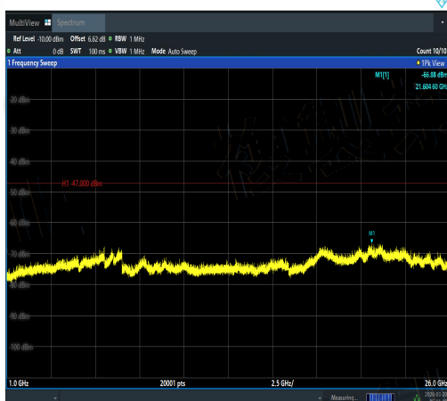
NTVN-11AX20MIMO-Ant2-5700-1000~26000-PA SS
