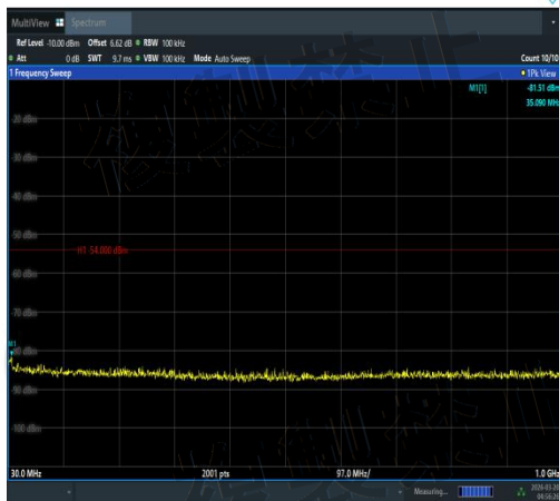
NTNV-11AC20MIMO-Ant3-5700-30~1000-PASS
