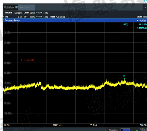
NTVN-11AC160SISO-Ant3-5570-1000~26000-PASS
