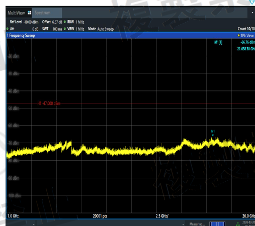
NTVN-11AX80MIMO-Ant3-5610-1000~26000-PA SS
