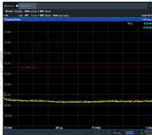
NTVN-11AC160MIMO-Ant2-5570-30~1000-PAS S
