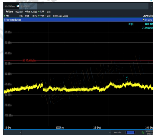
NTVN-11AC20MIMO-Ant1-5500-1000~26000-PA SS
