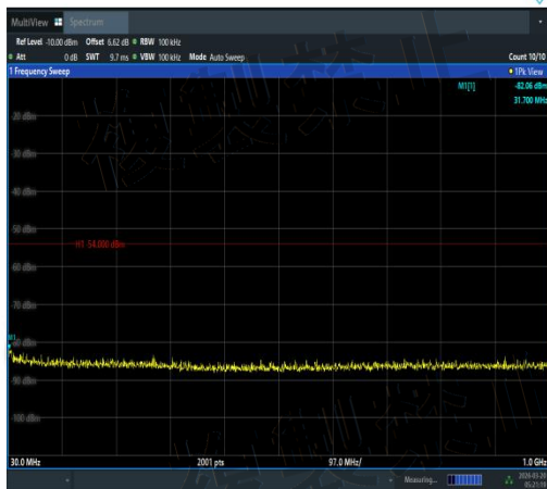
NTVN-11AX80MIMO-Ant3-5690-30~1000-PASS
