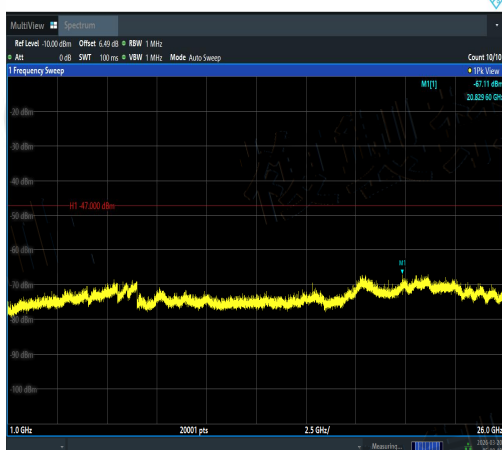
NTVN-11AX20MIMO-Ant2-5500-1000~26000-PA SS
