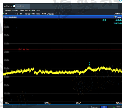
NTVN-11AX20SISO-Ant3-5700-1000~26000-PA SS
