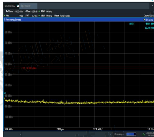
NTNV-11AX20SISO-Ant2-5600-30~1000-PASS
