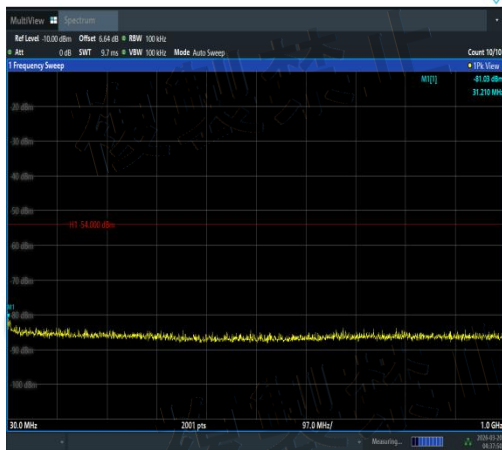
NTVN-11AC160SISO-Ant1-5570-30~1000-PASS
