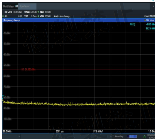
NTVN-11AX20MIMO-Ant3-5700-30~1000-PASS
