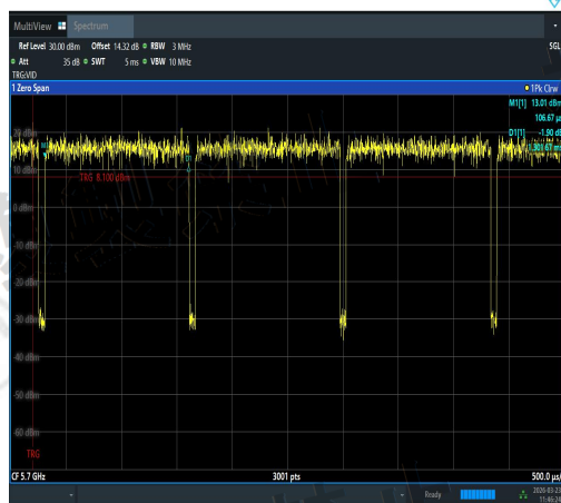
NTNV-11N20SISO-Ant2-5700-PASS
