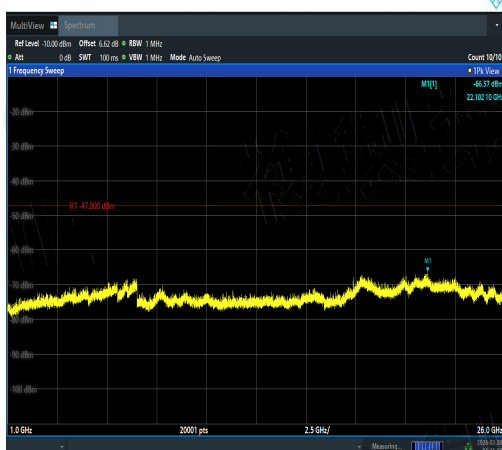
NTVN-11AC40SISO-Ant2-5670-1000~26000-PA SS
