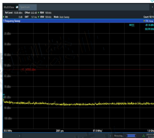
NTNV-11AX40MIMO-Ant2-5670-30~1000-PASS
