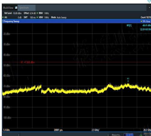
NTVN-11AX20MIMO-Ant2-5600-1000~26000-PA SS
