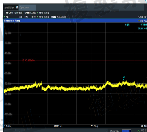
NTVN-11AX40MIMO-Ant3-5510-1000~26000-PA SS
