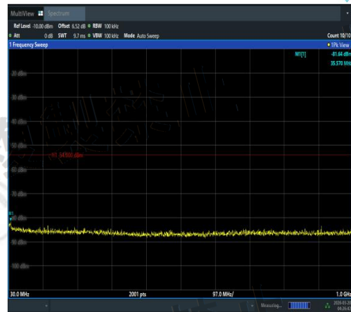
NTNV-11AX80SISO-Ant2-5530-30~1000-PASS
