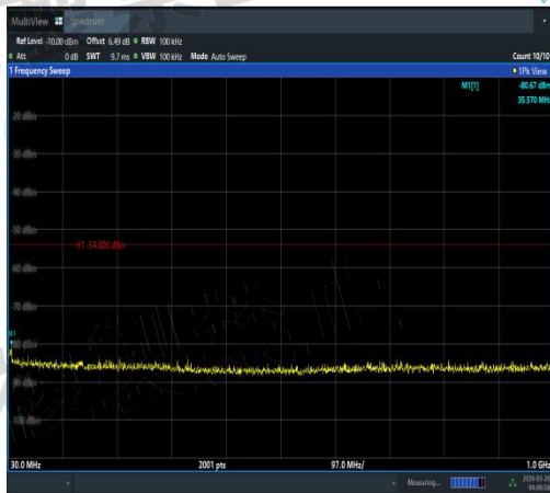
NTNV-11AX20SISO-Ant1-5600-30~1000-PASS
