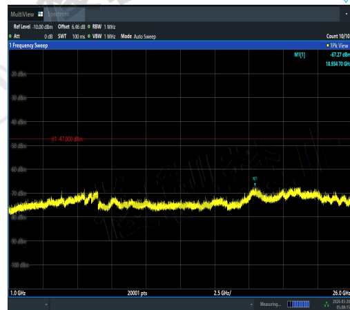
NTVN-11AX20MIMO-Ant1-5500-1000~26000-PA SS
