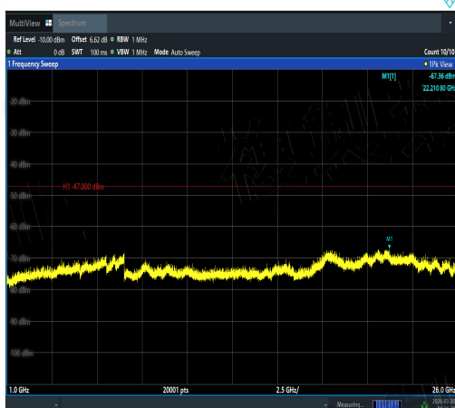
NTVN-11AX20SISO-Ant2-5700-1000~26000-PA SS
