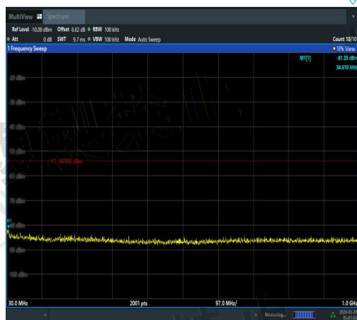
NTVN-11AC40MIMO-Ant2-5670-30~1000-PASS
