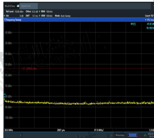
NTVN-11AX40MIMO-Ant2-5510-30~1000-PASS
