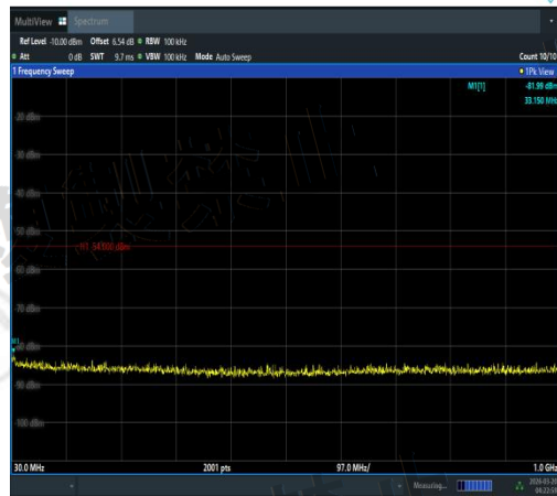
NTVN-11AC160SISO-Ant2-5570-30~1000-PASS
