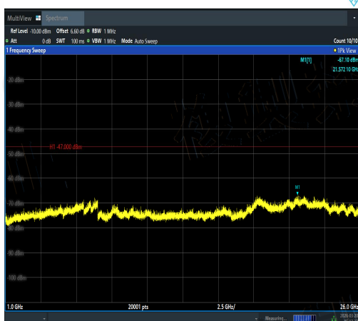
NTVN-11AX40MIMO-Ant2-5710-1000~26000-PA SS
