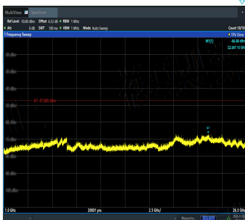
NTVN-11AC40SISO-Ant2-5510-1000~26000-PA SS
