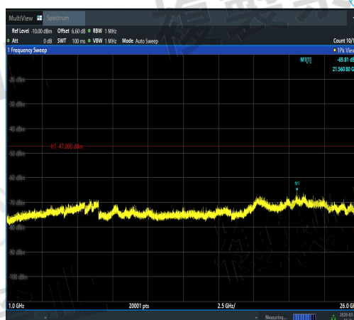
NTNV-11AC40SISO-Ant3-5550-1000~26000-PA SS
