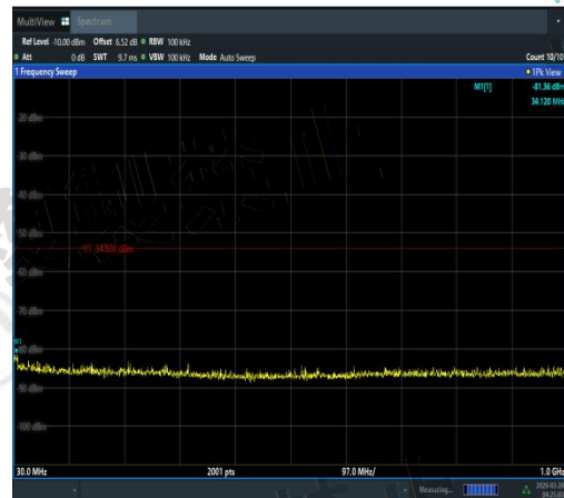
NTNV-11AX40SISO-Ant2-5510-30~1000-PASS
