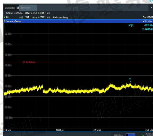
NTNV-11AC80MIMO-Ant3-5690-1000~26000-PA SS
