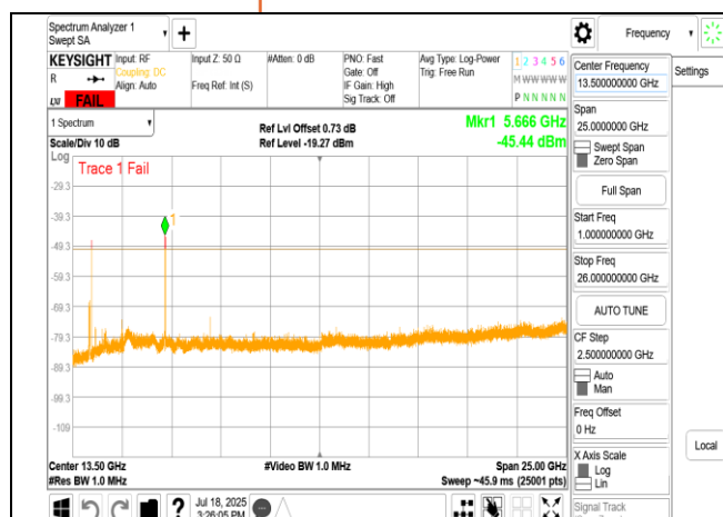
LPI 802.11n 40MHz Chain0 6405MHz Range2
