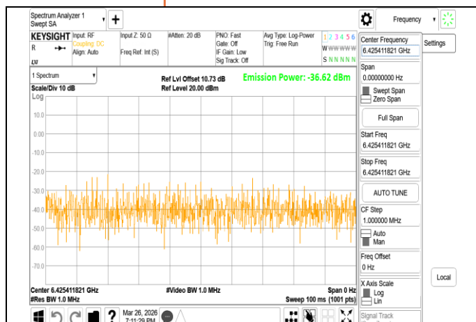
VLP 802.11ax 40MHz Chain1 6405MHz Range3 Sample
