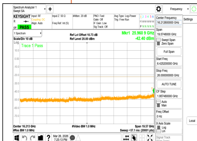
VLP 802.11ax 80MHz Chain0 6145MHz Range3
