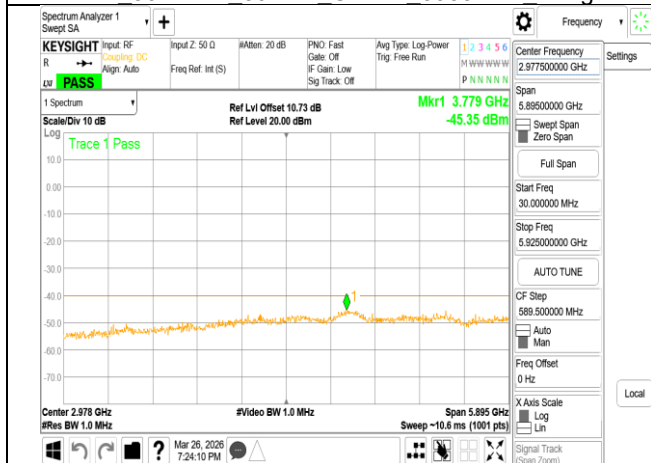
VLP 802.11ax 80MHz Chain1 6145MHz Range1
