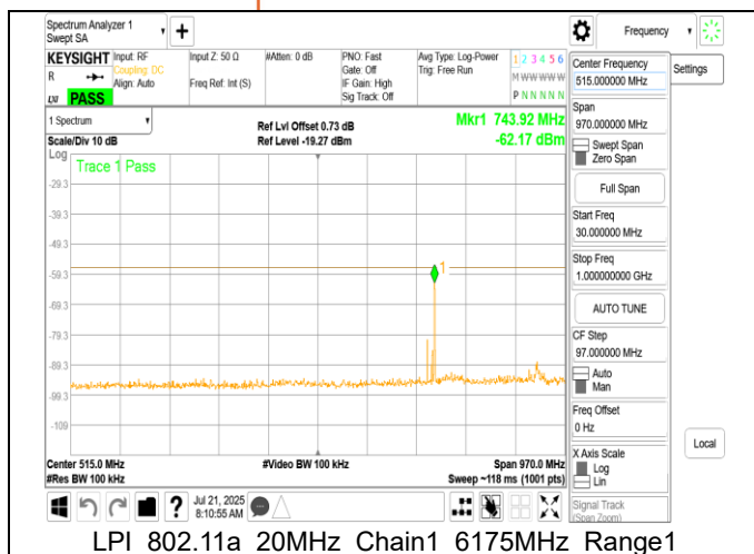
LPI 802.11a 20MHz Chain1 6175MHz Range1 Sample
