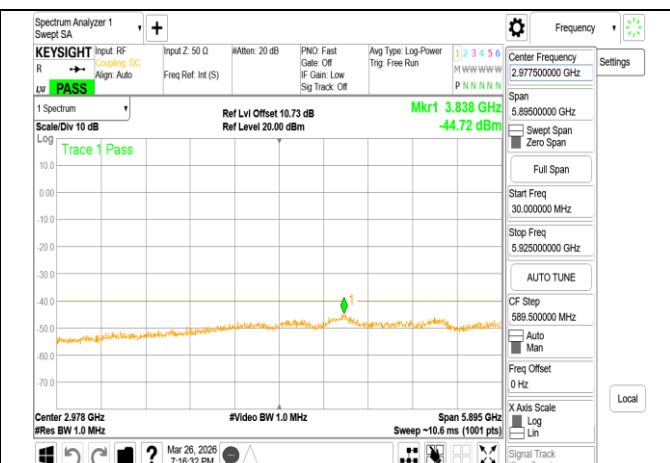
VLP 802.11ax 80MHz Chain0 5985MHz Range1
