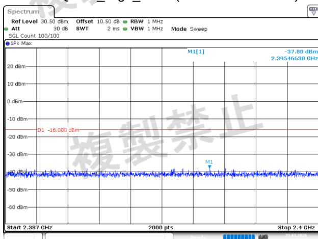
\pi/4 -DQPSK_High_2DH1(2.387GHz~2.4GHz)
