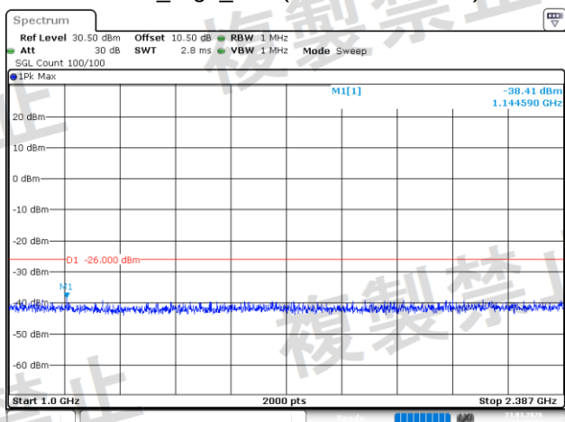
GFSK_High_DH1(1GHz~2.387GHz)
