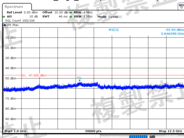
8DPSK_High_3DH1(1GHz~12.5GHz)
