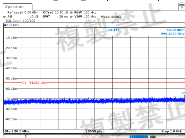
8DPSK_Middle_3DH1(30MHz~1GHz)
