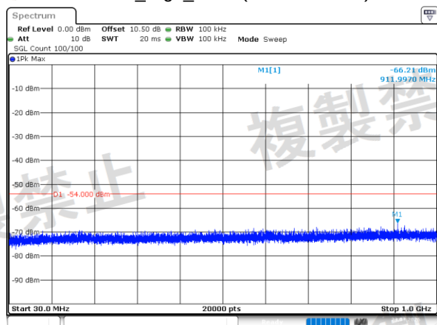
8DPSK_High_3DH1(30MHz~1GHz)
