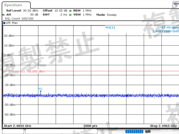
8DPSK_High_3DH1(2.4835GHz~2.4965GHz)
