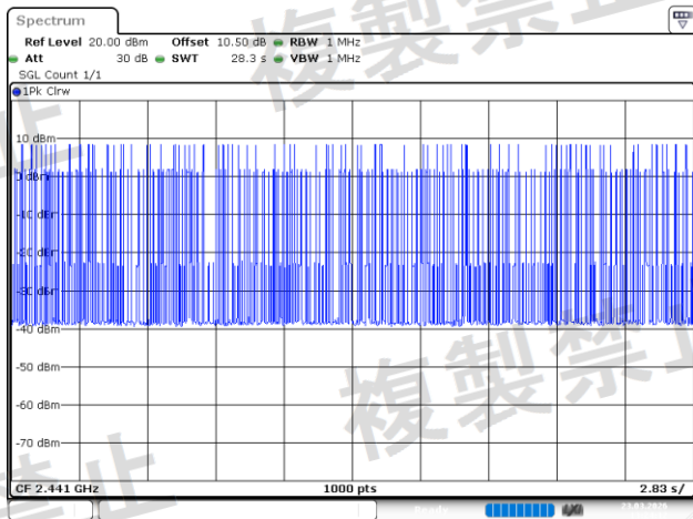
8DPSK_Hopping_3DH5
