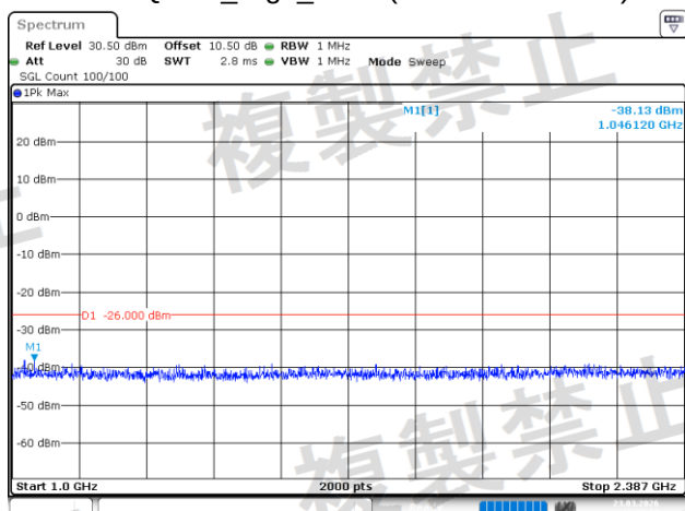
\pi/4 -DQPSK_High_2DH1(1GHz~2.387GHz)
