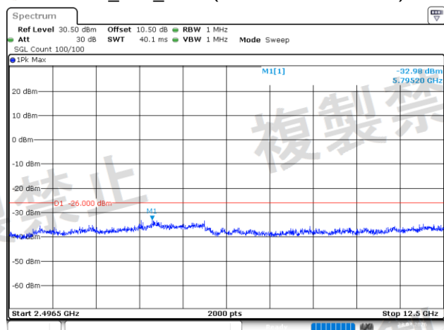
8DPSK_Low_3DH1(2.4965GHz~12.5GHz)
