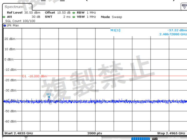
8DPSK_Low_3DH1(2.4835GHz~2.4965GHz)
