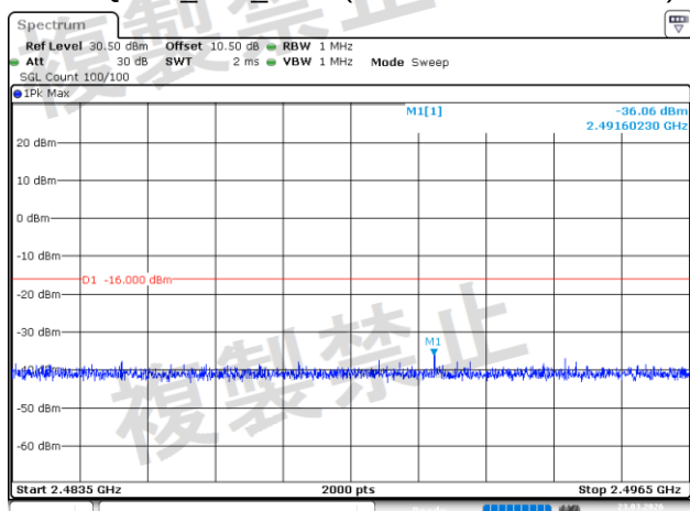
\pi/4 -DQPSK_Low_2DH1(2.4835GHz~2.4965GHz)
