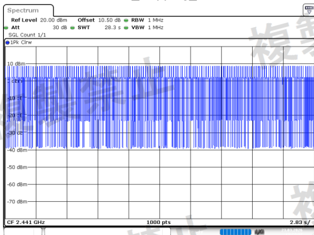
8DPSK_Hopping_3DH1
