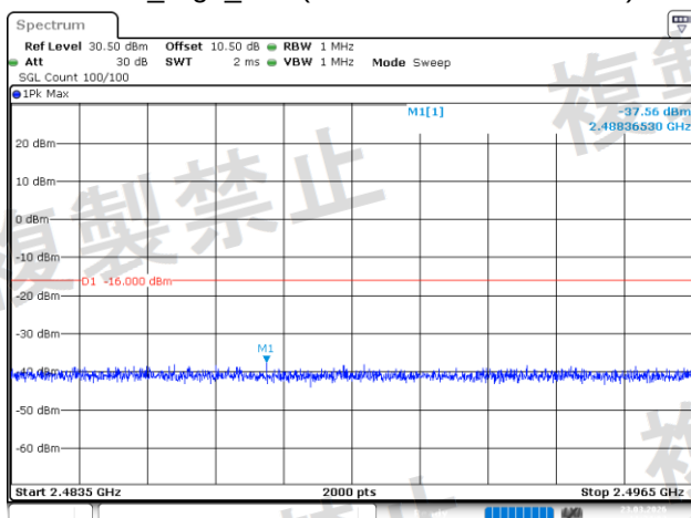
GFSK_High_DH1(2.4835GHz~2.4965GHz)
