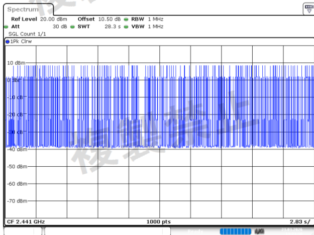
8DPSK_Hopping_3DH3
