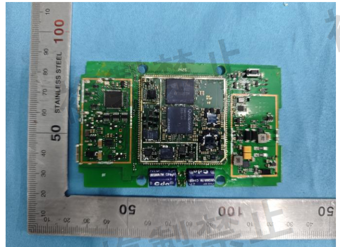
PCB 2
