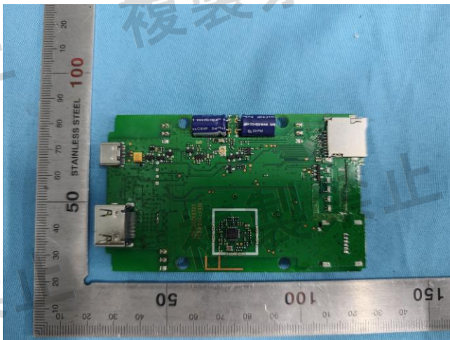
PCB 1
