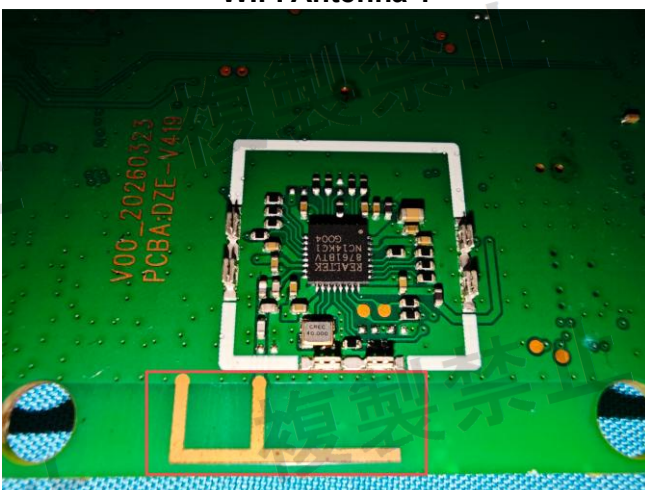
Bluetooth Antenna
