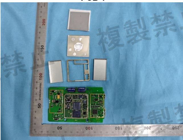
PCB 3
