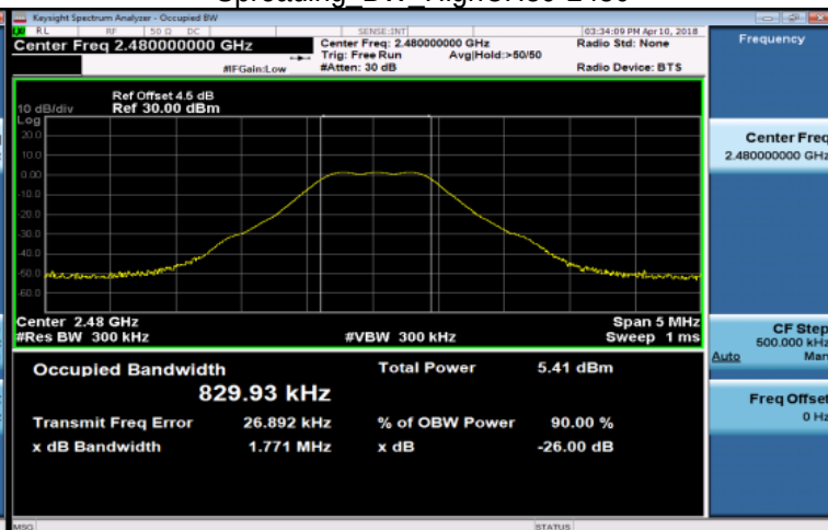
Spreading BW HighCH39-2480
