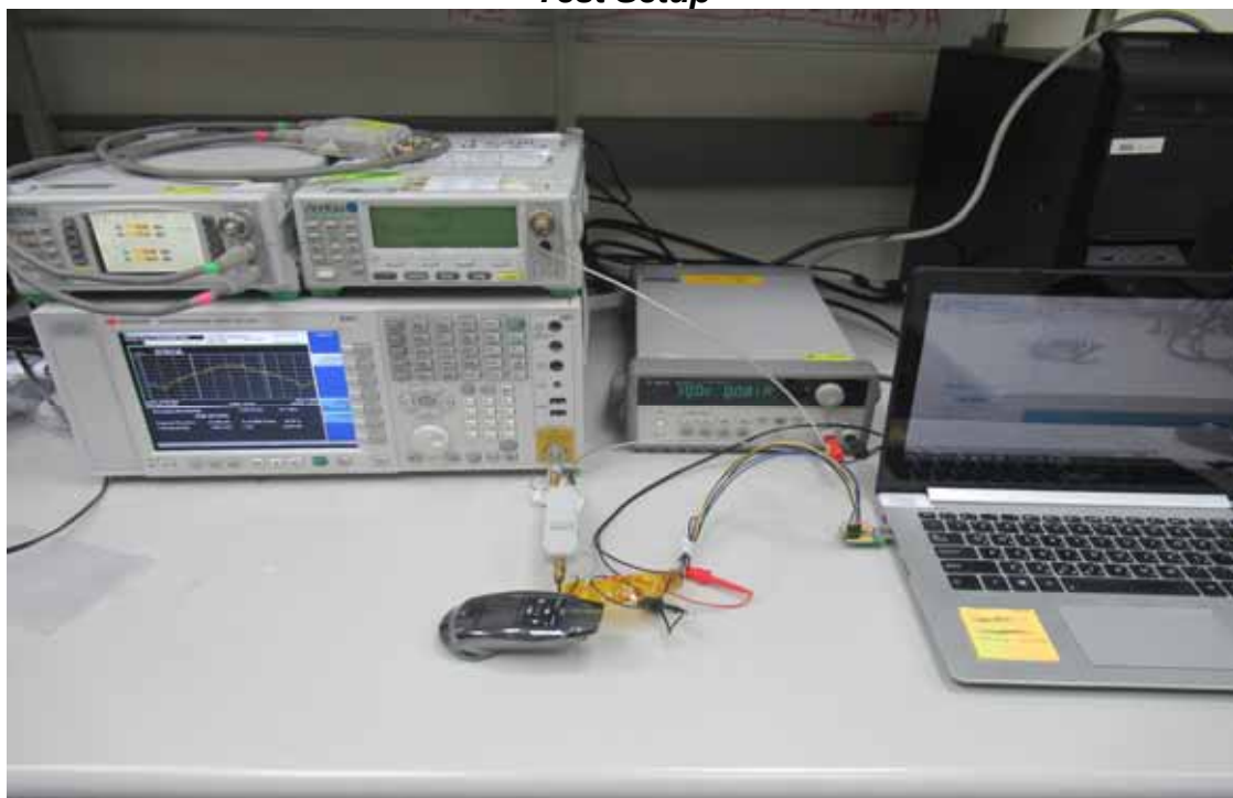
Test Setup
