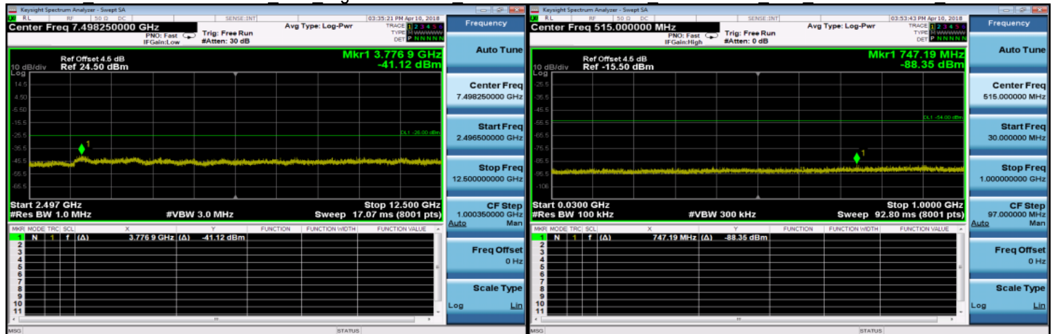
TX 2496.5MHz~12.5GHz BLE HighCH39-2480 5
