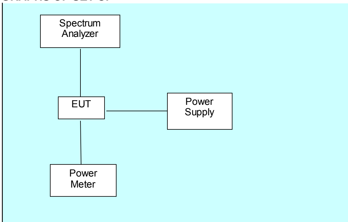
Test Setup
