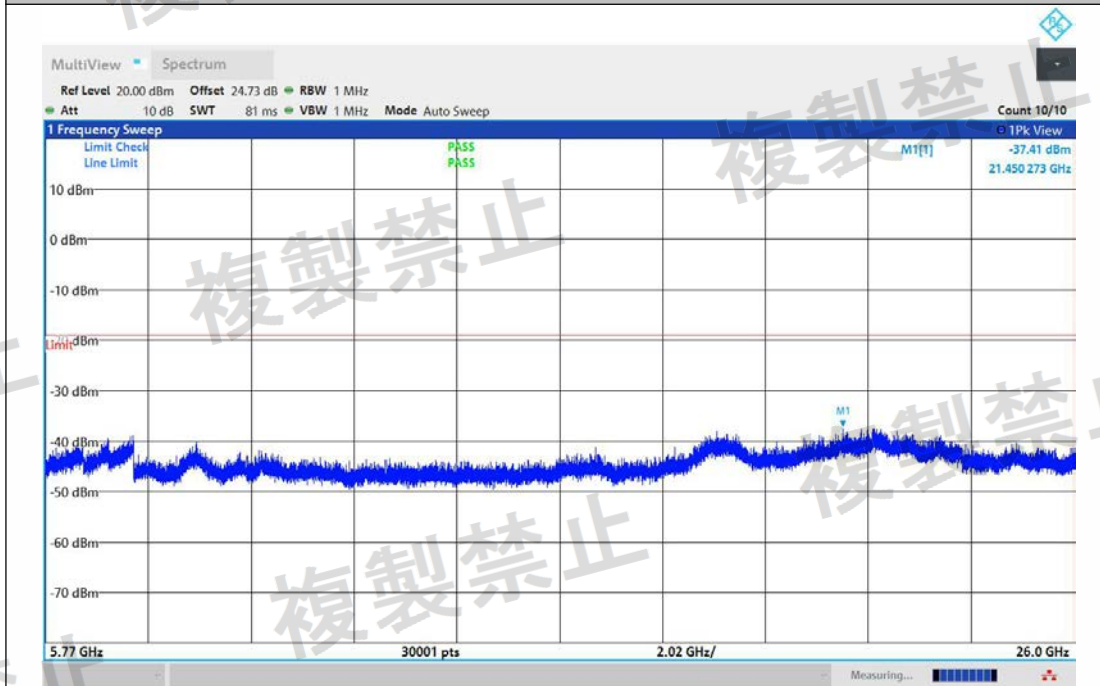
NTNV-11AX40MIMO-Ant2-5510-5770~26000-PASS
