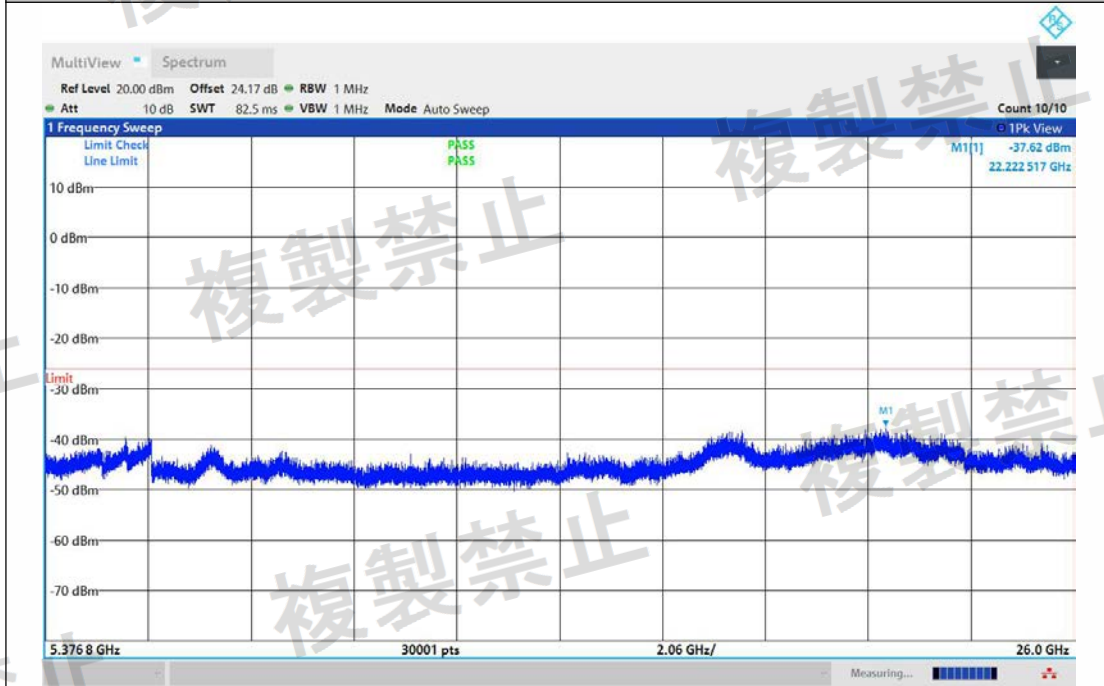
NTNV-11AX80MIMO-Ant2-5290-5376.8~26000-PASS
