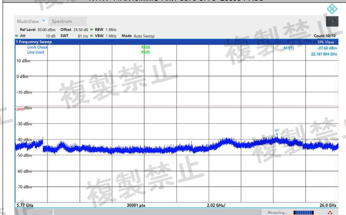
NTNV-11AX40MIMO-Ant2-5670-5770~26000-PASS
