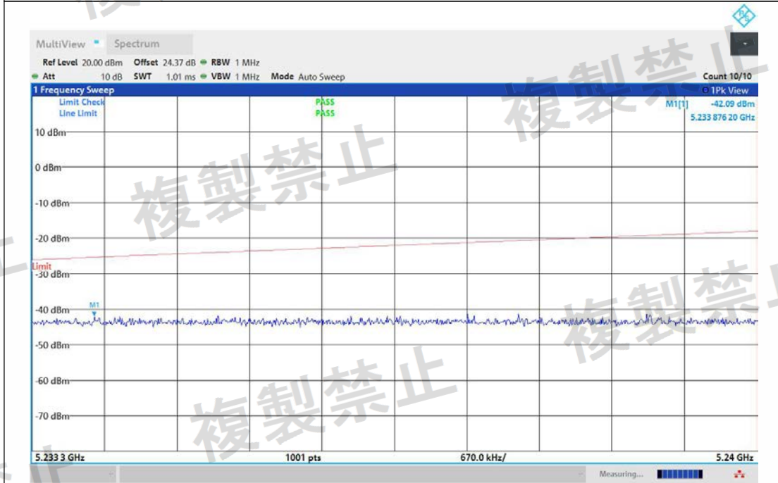
NTNV-11AX20MIMO-Ant2-5320-5233.3~5240-PASS
