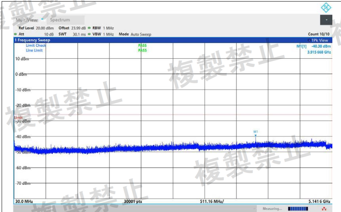
NTNV-11AX40MIMO-Ant1-5230-30~5141.6-PASS
