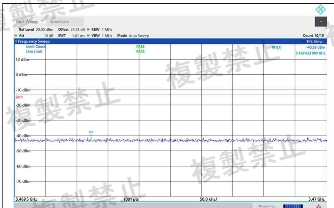
NTNV-11AX80MIMO-Ant1-5610-5469.5~5470-PASS
