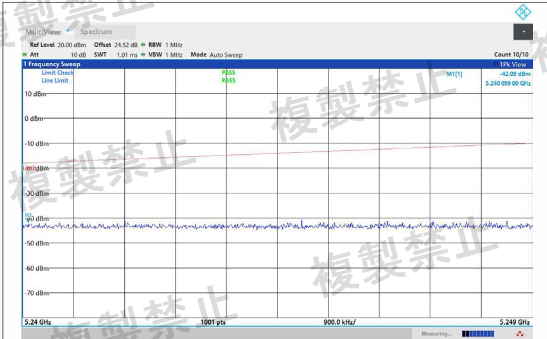
NTNV-11AX20MIMO-Ant1-5320-5240~5249-PASS
