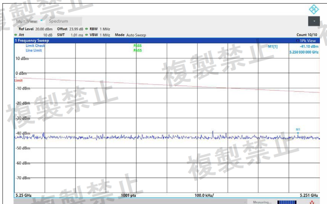
NTNV-11AX40MIMO-Ant1-5190-5250~5251-PASS
