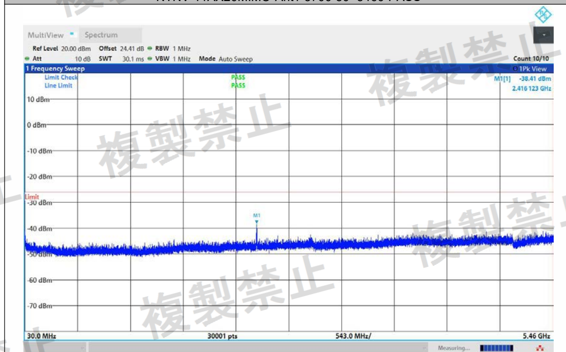
NTNV-11AX20MIMO-Ant2-5700-30~5460-PASS
