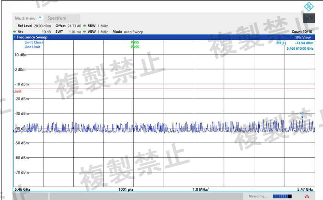
NTNV-11AX40MIMO-Ant2-5510-5460~5470-PASS
