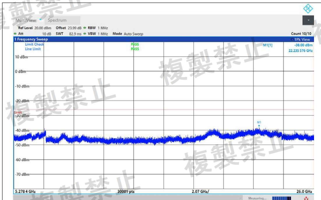
NTNV-11AX40MIMO-Ant1-5190-5278.4~26000-PASS
