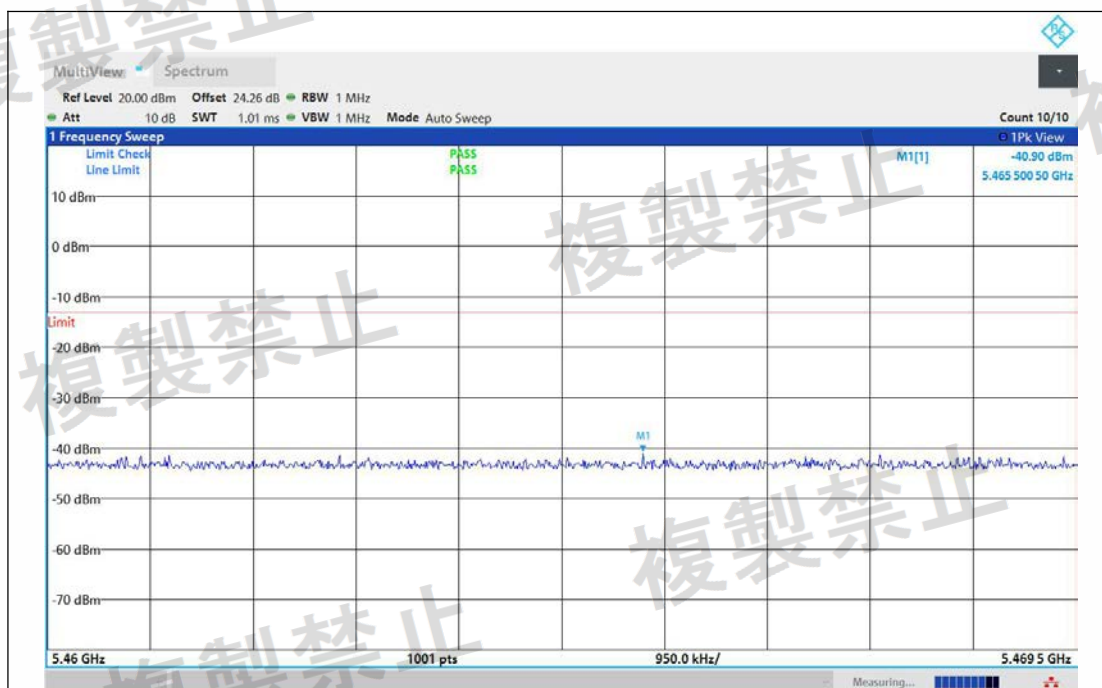
NTNV-11AX80MIMO-Ant1-5610-5460~5469.5-PASS
