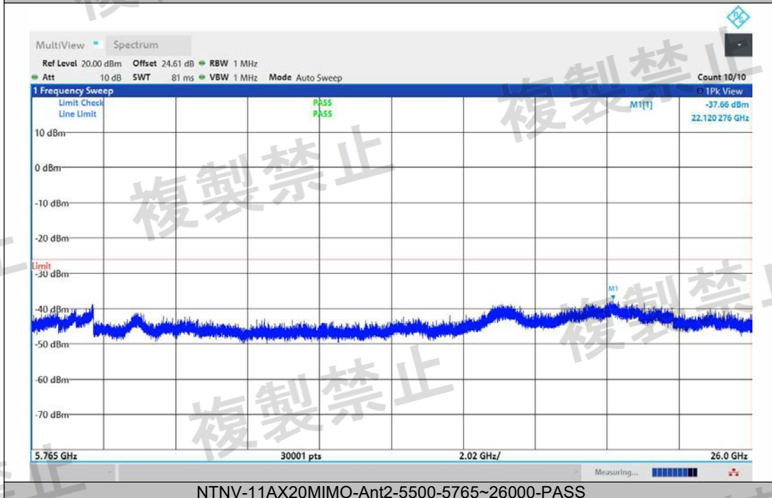
NTNV-11AX20MIMO-Ant2-5500-5765~26000-PASS
