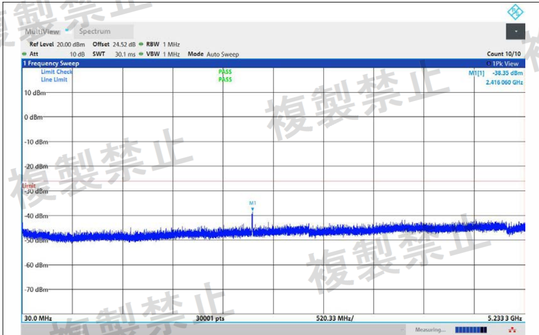
NTNV-11AX20MIMO-Ant1-5320-30~5233.3-PASS
