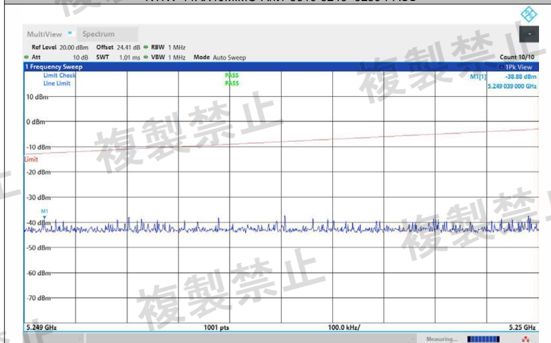
NTNV-11AX40MIMO-Ant2-5310-5249~5250-PASS
