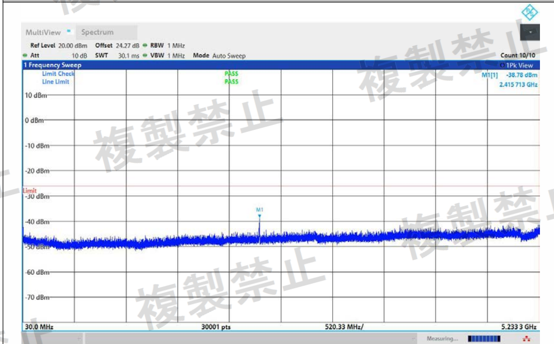
NTNV-11AX20MIMO-Ant2-5260-30~5233.3-PASS
