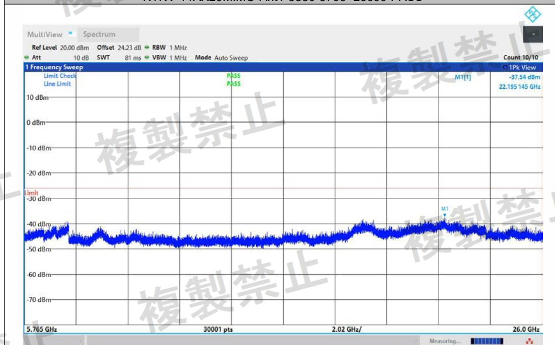
NTNV-11AX20MIMO-Ant2-5580-5765~26000-PASS
