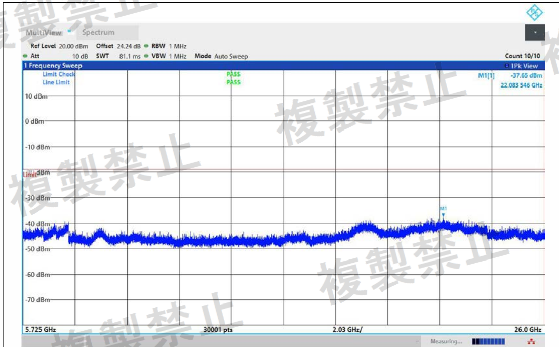
NTNV-11AX160MIMO-Ant1-5570-5725~26000-PASS
