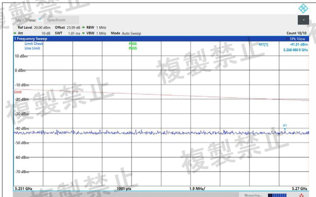
NTNV-11AX40MIMO-Ant1-5190-5251~5270-PASS
