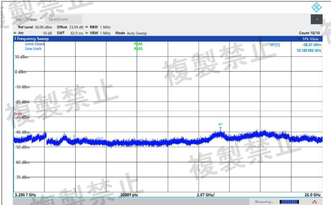
NTNV-11AX80MIMO-Ant1-5210-5296.7~26000-PASS
