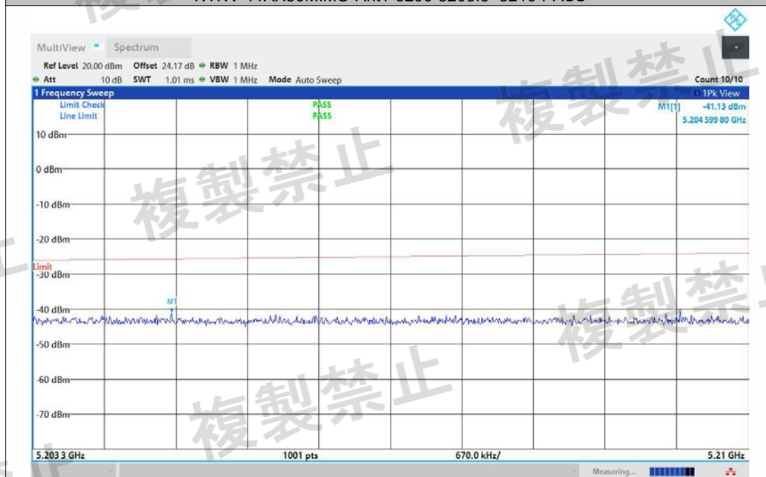
NTNV-11AX80MIMO-Ant2-5290-5203.3~5210-PASS
