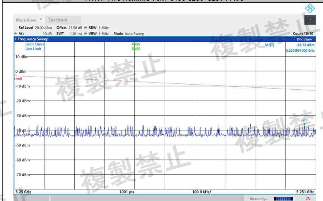
NTNV-11AX40MIMO-Ant2-5190-5250~5251-PASS
