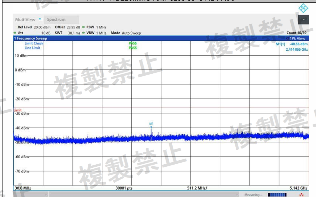
NTNV-11BE20MIMO-Ant2-5200-30~5142-PASS
