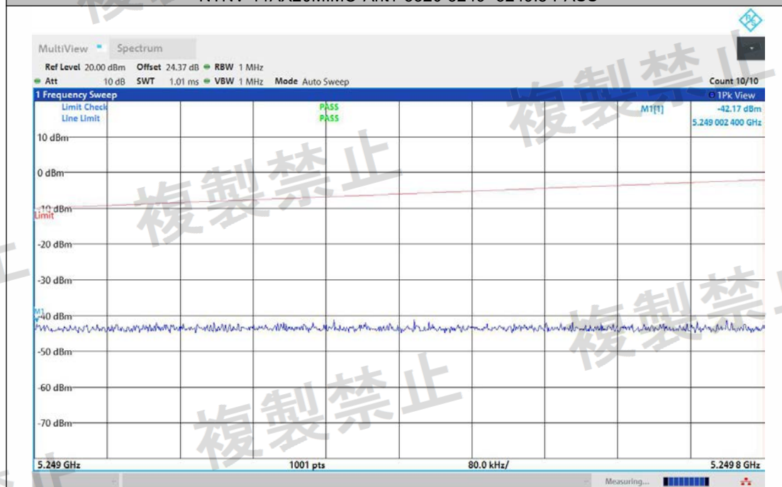
NTNV-11AX20MIMO-Ant2-5320-5249~5249.8-PASS
