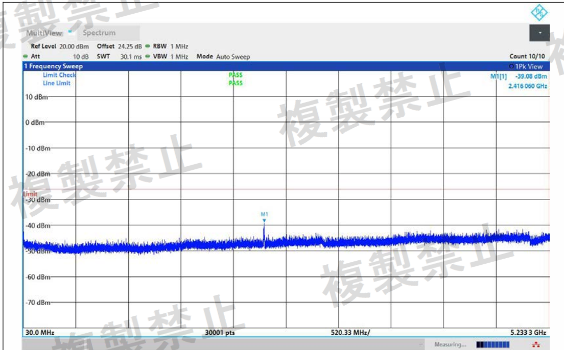
NTNV-11AX20MIMO-Ant1-5280-30~5233.3-PASS
