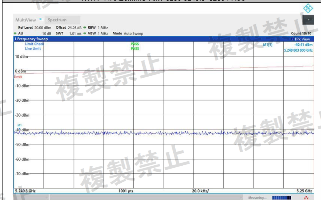
NTNV-11AX20MIMO-Ant2-5280-5249.8~5250-PASS
