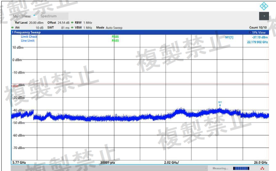
NTNV-11AX80MIMO-Ant1-5530-5770~26000-PASS
