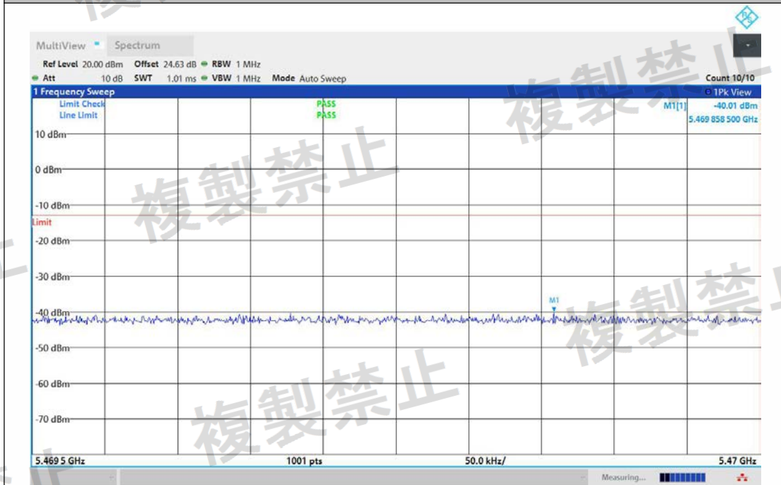
NTNV-11AX80MIMO-Ant2-5530-5469.5~5470-PASS
