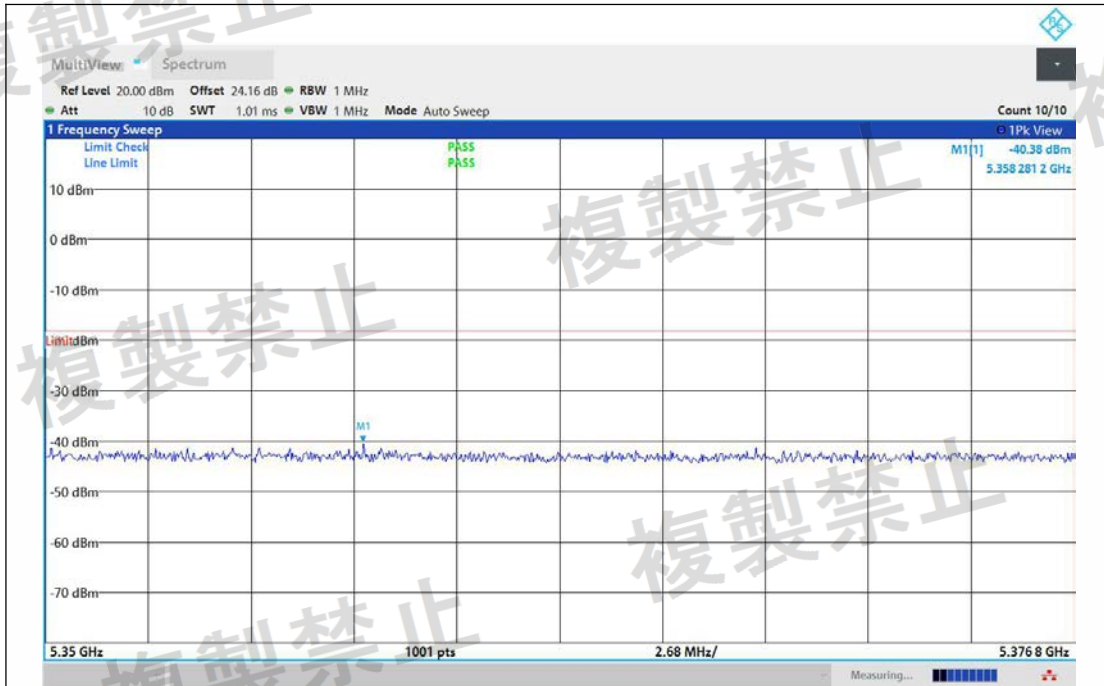
NTNV-11AX80MIMO-Ant1-5290-5350~5376.8-PASS
