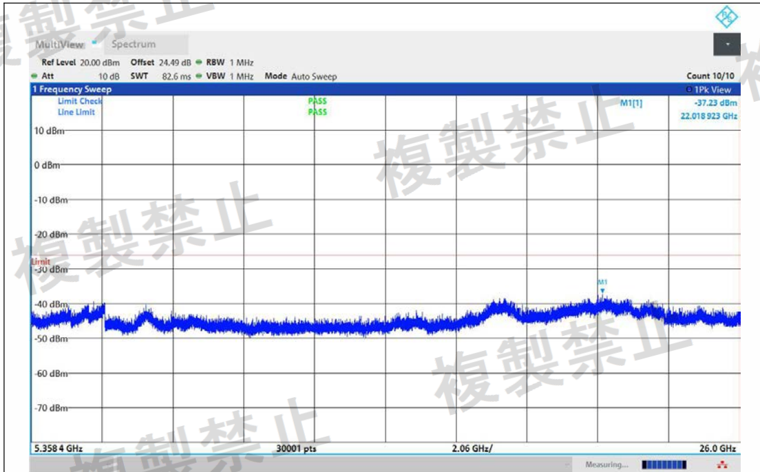
NTNV-11AX40MIMO-Ant1-5310-5358.4~26000-PASS
