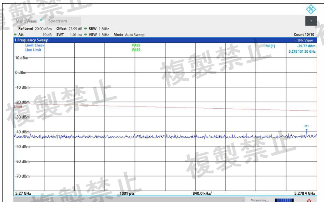
NTNV-11AX40MIMO-Ant1-5190-5270~5278.4-PASS
