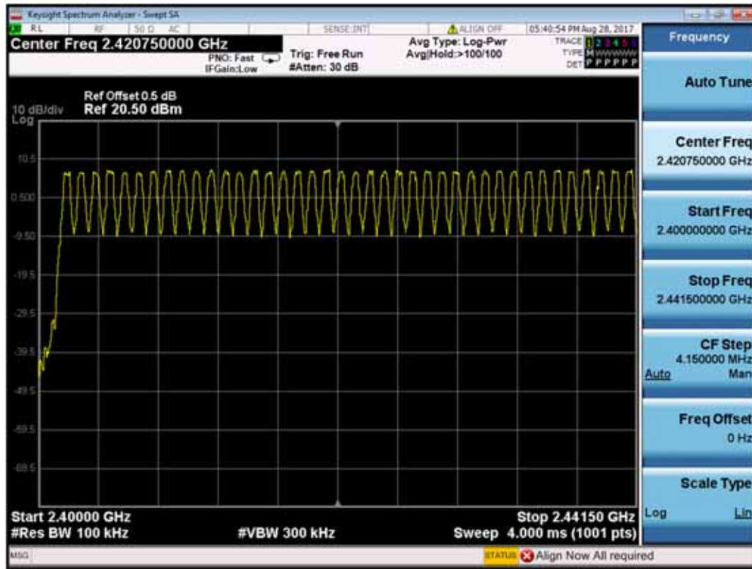
Hopping channel
