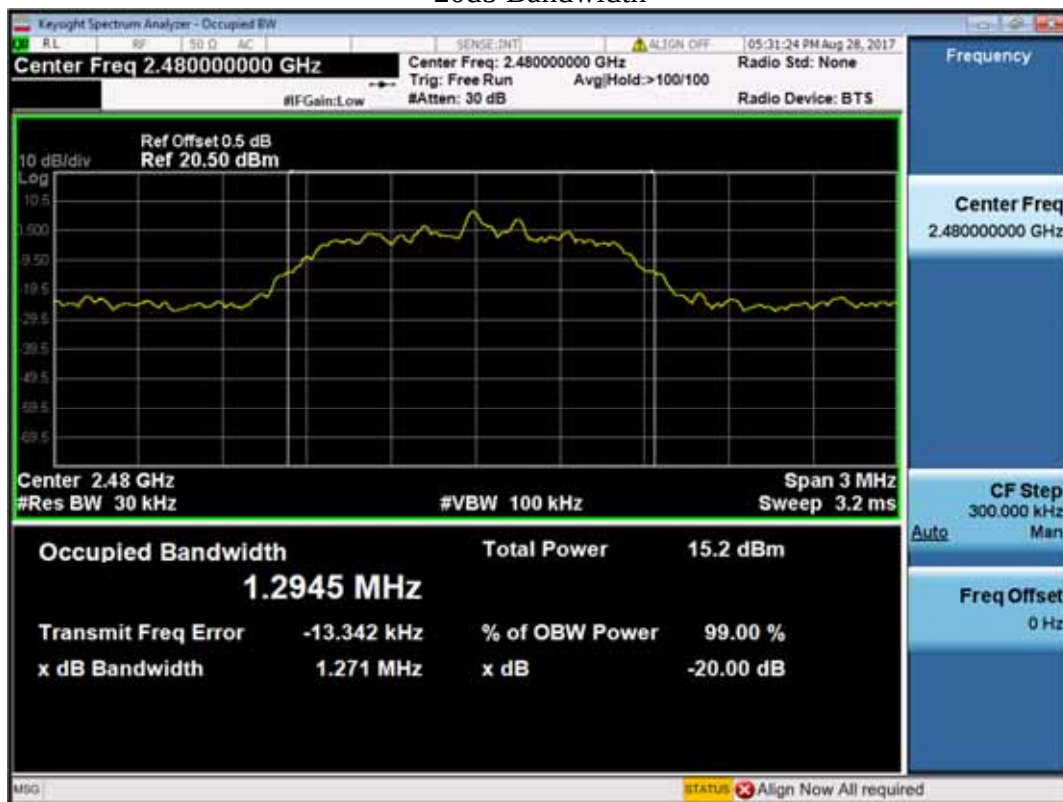
20db Bandwidth
