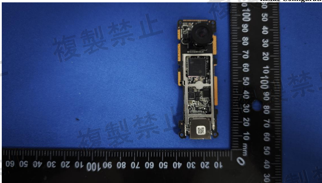
Figure 14 Inside Configuration of the EUT
