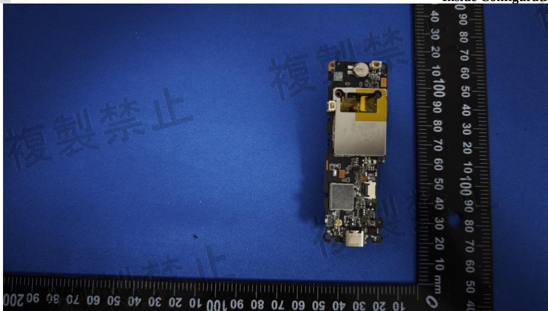
Figure 13 Inside Configuration of the EUT
