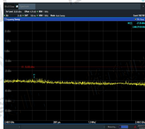
NTVN-11N40SISO-Ant2-2442-2483.5~2496.5-PASS
