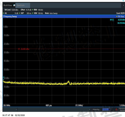
NTVN-11AX20MIMO-Ant2-2472-30~1000-PASS
