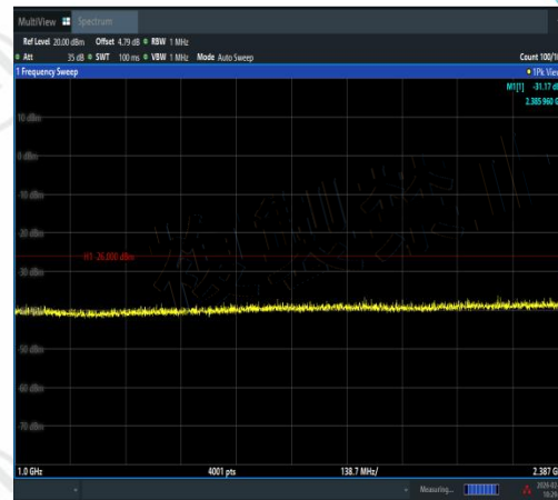
NTVN-11N40MIMO-Ant2-2442-1000~2387-PASS
