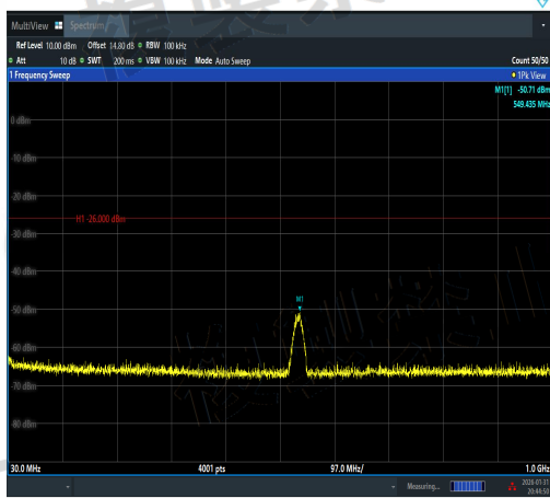
NTVN-11AX20SISO-Ant1-2472-30~1000-PASS
