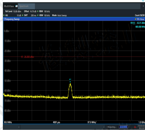
NTVN-11AX20SISO-Ant2-2442-30~1000-PASS
