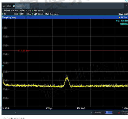
NTVN-11N40SISO-Ant2-2462-30~1000-PASS
