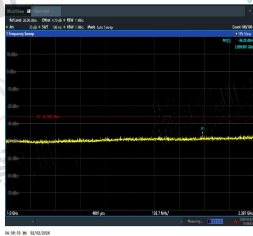
NTVN-11AX20MIMO-Ant2-2472-1000~2387-PAS
