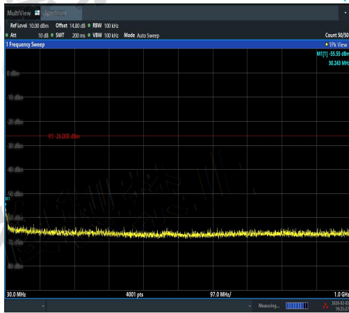
NTVN-11N40MIMO-Ant1-2442-30~1000-PASS
