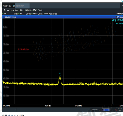
NTNV-11AX20MIMO-Ant2-2442-30~1000-PASS
