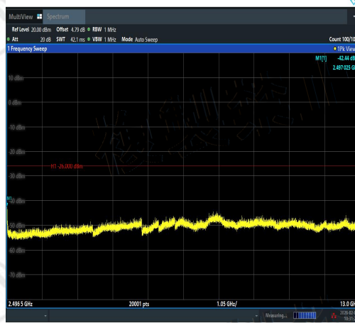
NTNV-11N40MIMO-Ant2-2442-2496.5~13000-P ASS
