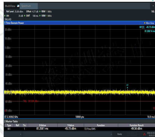
NTVN-11N20MIMO-Ant1-2412-1000~2387-PASS
