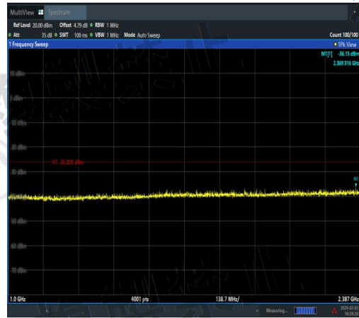
NTNV-11N40MIMO-Ant2-2462-1000~2387-PASS
