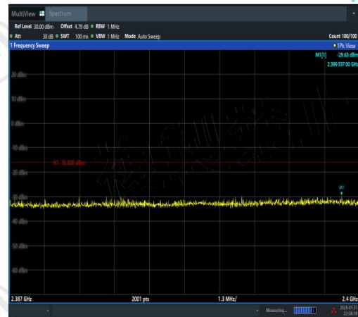
NTVN-11N40SISO-Ant2-2442-2387~2400-PASS
