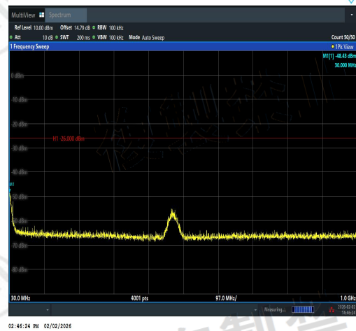
NTVN-11AX40SISO-Ant2-2442-30~1000-PASS
