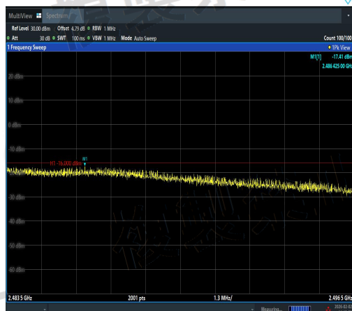
NTNV-11N20SISO-Ant2-2472-2483.5~2496.5-See table below
