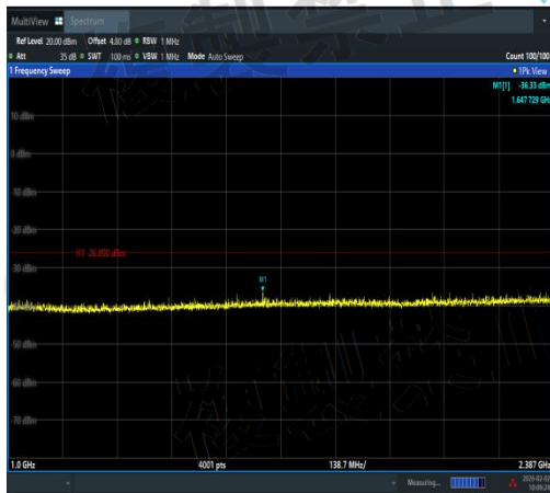
NTVN-11N20MIMO-Ant1-2472-1000~2387-PASS
