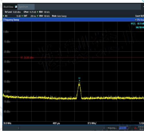
NTVN-11AX20SISO-Ant2-2472-30~1000-PASS
