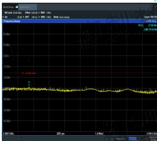
NTVN-11N40SISO-Ant1-2442-2483.5~2496.5-PASS
