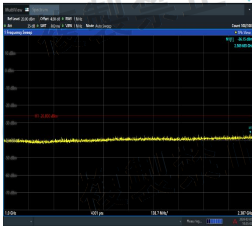
NTVN-11N40MIMO-Ant1-2442-1000~2387-PASS
