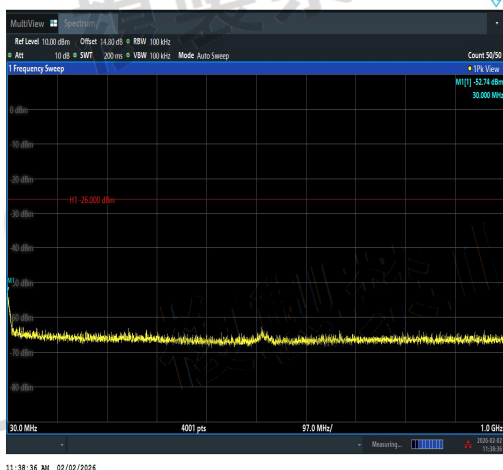
NTVN-11AX40MIMO-Ant1-2462-30~1000-PASS
