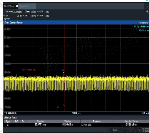
NTNV-11N40SISO-Ant2-2462-2483.5~2496.5-PA
