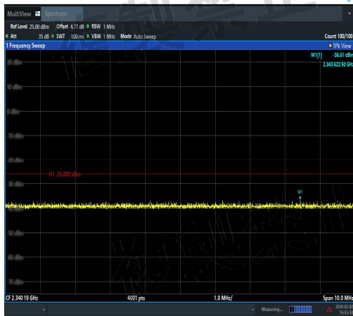
NTVN-11N20MIMO-Ant1-2412-1000~2387-PASS
