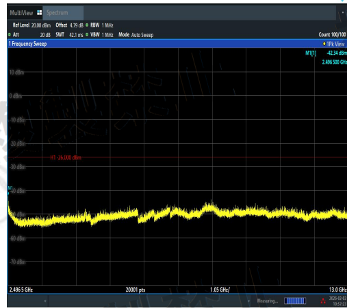
NTVN-11AX20MIMO-Ant2-2442-2496.5~13000-P ASS
