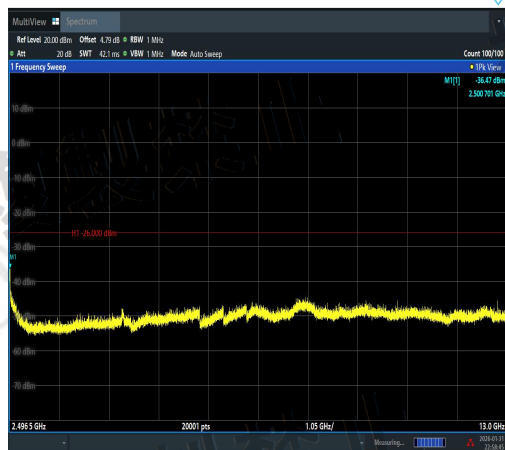
NTVN-11N40SISO-Ant2-2442-2496.5~13000-PA SS
