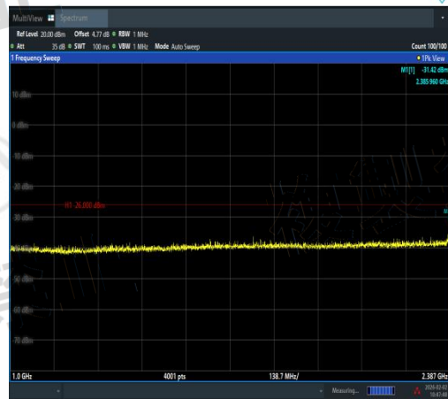
NTVN-11AX20MIMO-Ant2-2412-1000~2387-PAS
