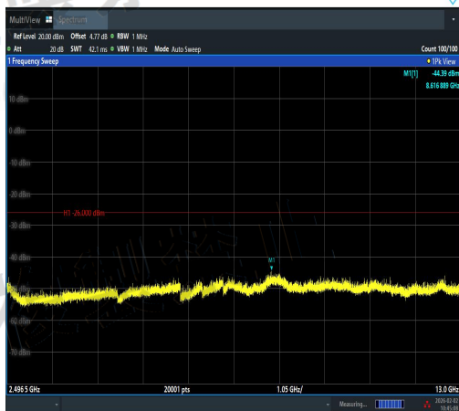
NTNV-11AX20MIMO-Ant1-2412-2496.5~13000-P ASS
