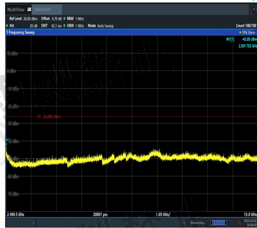
NTVN-11AX20MIMO-Ant2-2472-2496.5~13000-P ASS
