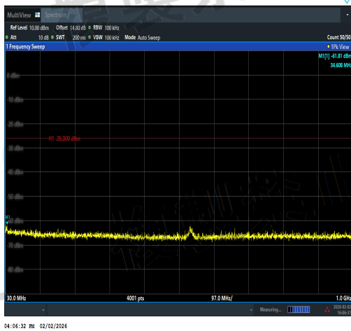
NTVN-11AX20MIMO-Ant1-2472-30~1000-PASS
