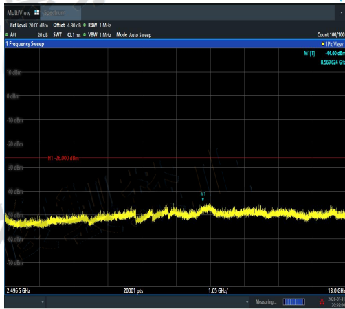
NTVN-11AX40SISO-Ant1-2422-2496.5~13000-P ASS
