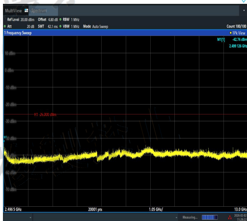
NTVN-11AX40MIMO-Ant1-2442-2496.5~13000-P ASS
