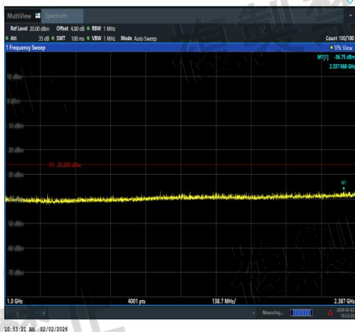
NTNV-11AX20MIMO-Ant1-2442-1000~2387-PAS
