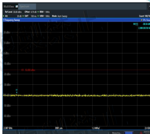
NTNV-11N20SISO-Ant2-2472-2387~2400-PASS
