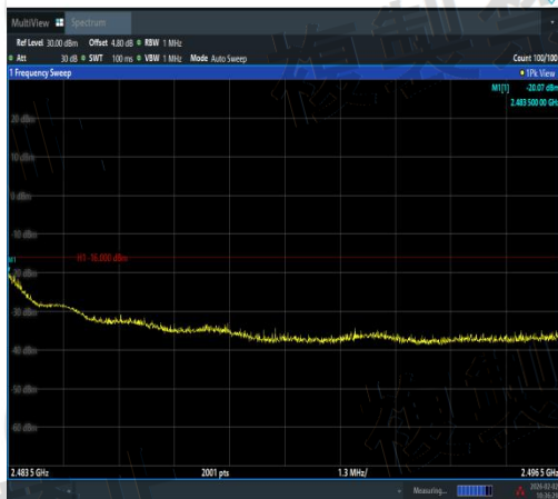
NTNV-11N40MIMO-Ant1-2462-2483.5~2496.5-P
