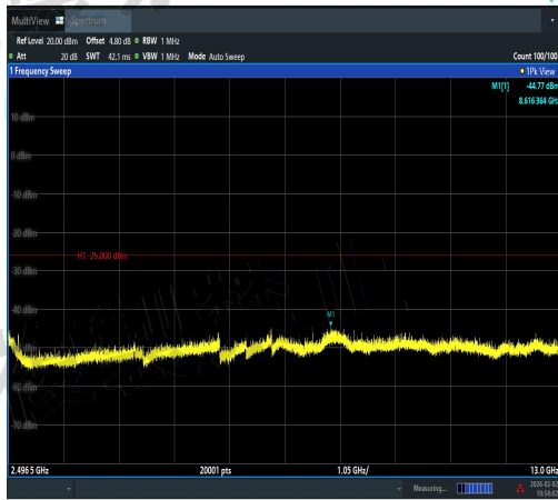
NTVN-11AX20MIMO-Ant1-2442-2496.5~13000-P ASS
