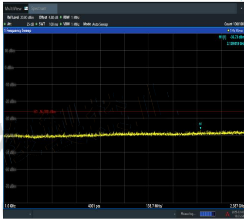
NTNV-11N40MIMO-Ant1-2462-1000~2387-PASS
