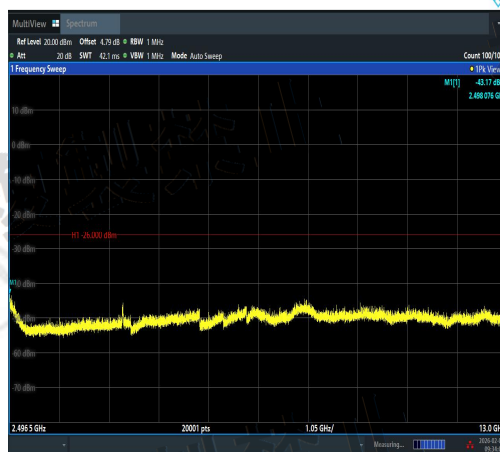
NTVN-11AX20SISO-Ant2-2442-2496.5~13000-P ASS
