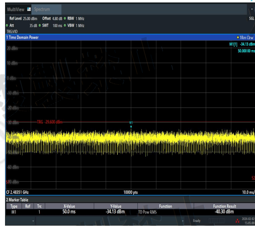
NTNV-11N40SISO-Ant1-2462-2483.5~2496.5-PA
