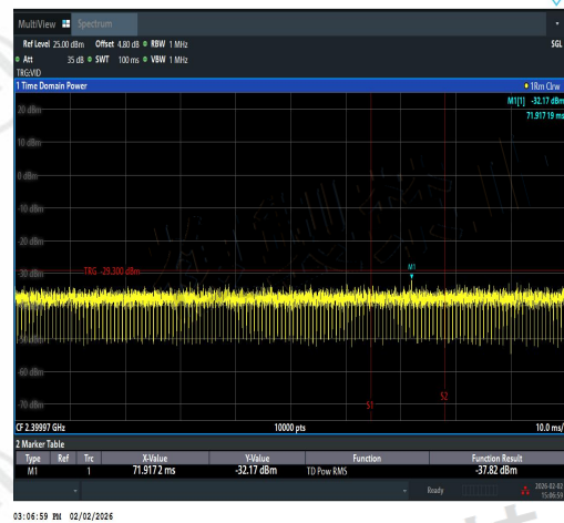
NTVN-11N40SISO-Ant1-2422-2387~2400-PASS
