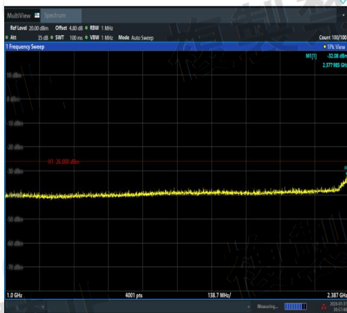
NTVN-11AX40SISO-Ant1-2422-1000~2387-PAS
