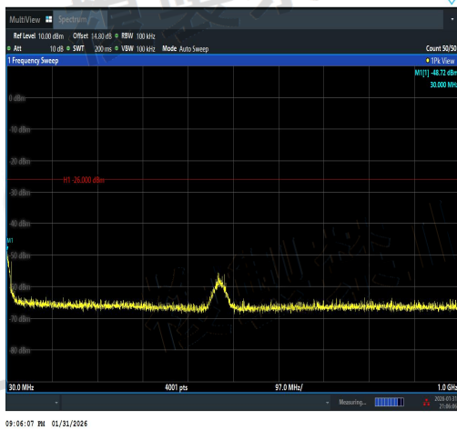
NTVN-11AX40SISO-Ant1-2442-30~1000-PASS
