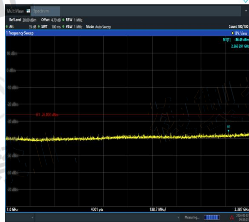
NTVN-11AX20SISO-Ant2-2442-1000~2387-PAS
