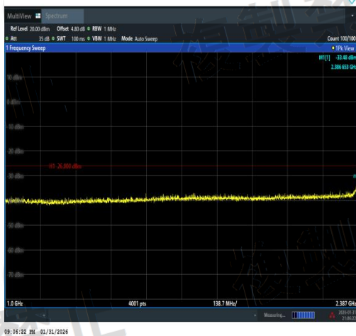
NTVN-11AX40SISO-Ant1-2442-1000~2387-PAS
