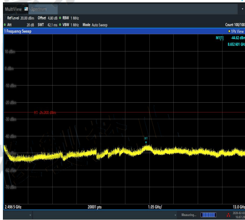
NTVN-11AX20MIMO-Ant1-2472-2496.5~13000-P ASS
