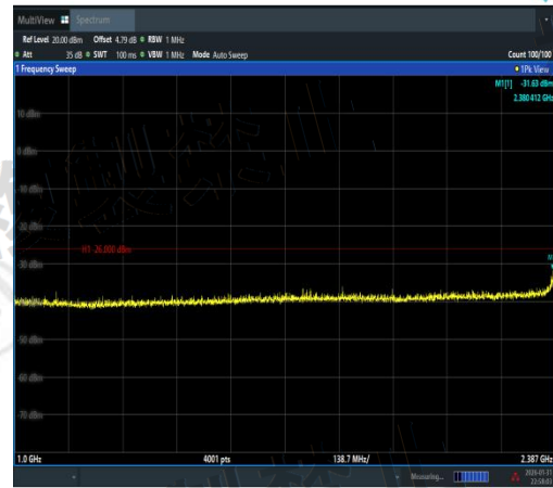
NTVN-11N40SISO-Ant2-2442-1000~2387-PASS
