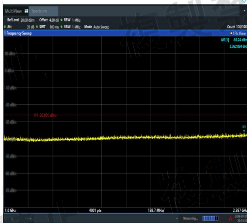
NTVN-11AX20SISO-Ant1-2442-1000~2387-PAS
