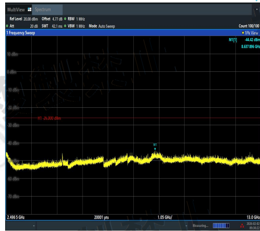
NTVN-11AX20SISO-Ant2-2412-2496.5~13000-P ASS
