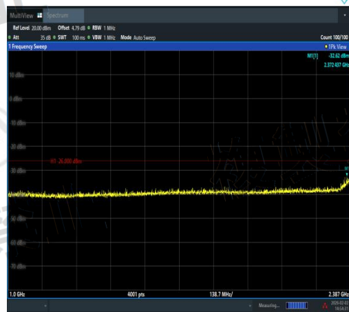
NTVN-11AX40SISO-Ant2-2422-1000~2387-PAS
