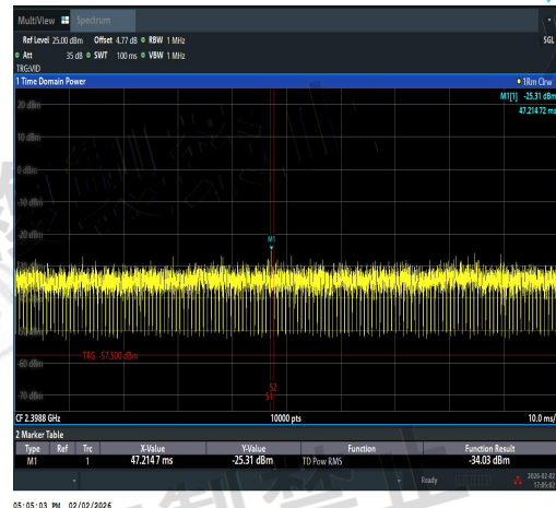
NTVN-11N20MIMO-Ant2-2412-2387~2400-PASS
