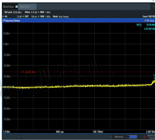
NTNV-11N40SISO-Ant2-2422-1000~2387-PASS
