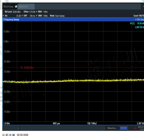
NTVN-11AX40MIMO-Ant2-2462-1000~2387-PAS
