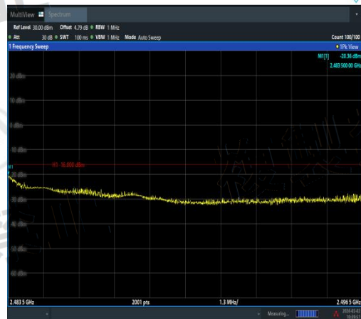
NTNV-11N40MIMO-Ant2-2462-2483.5~2496.5-P
