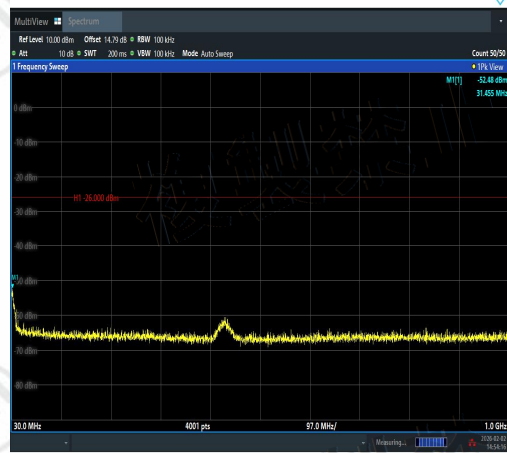
NTVN-11AX40SISO-Ant2-2422-30~1000-PASS
