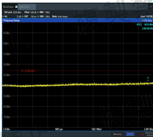
NTVN-11AX20SISO-Ant1-2472-1000~2387-PAS
