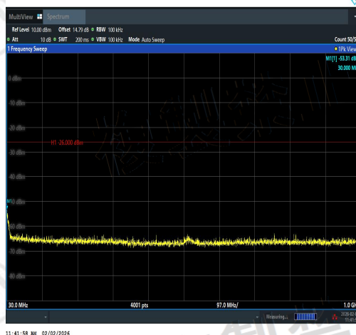
NTVN-11AX40MIMO-Ant2-2462-30~1000-PASS
