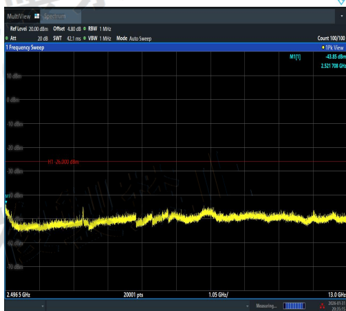
NTVN-11AX20SISO-Ant1-2442-2496.5~13000-P ASS
