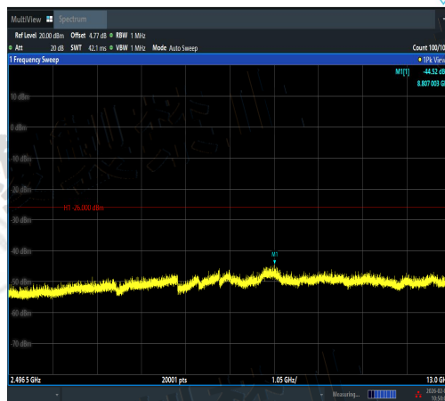
NTNV-11AX20MIMO-Ant2-2412-2496.5~13000-P ASS
