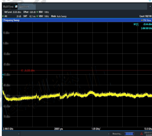
NTVN-11N40SISO-Ant1-2442-2496.5~13000-PA SS
