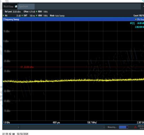
NTNV-11AX20MIMO-Ant2-2442-1000~2387-PAS
