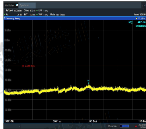
NTVN-11AX40SISO-Ant2-2422-2496.5~13000-P ASS
