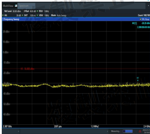
NTVN-11N40SISO-Ant1-2442-2387~2400-PASS
