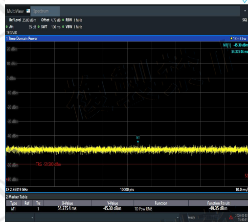
NTNV-11N40MIMO-Ant1-2422-1000~2387-PASS
