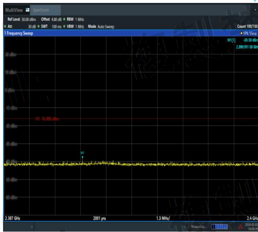
NTVN-11N20MIMO-Ant1-2472-2387~2400-PASS
