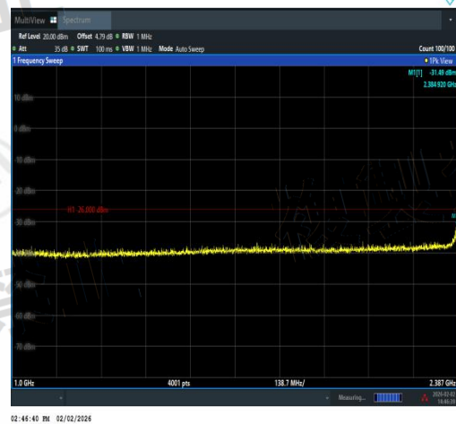
NTVN-11AX40SISO-Ant2-2442-1000~2387-PAS
