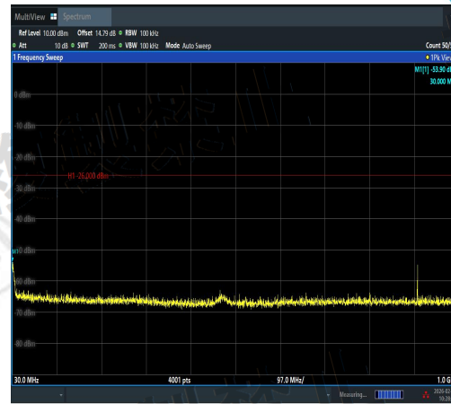
NTVN-11N40MIMO-Ant2-2442-30~1000-PASS
