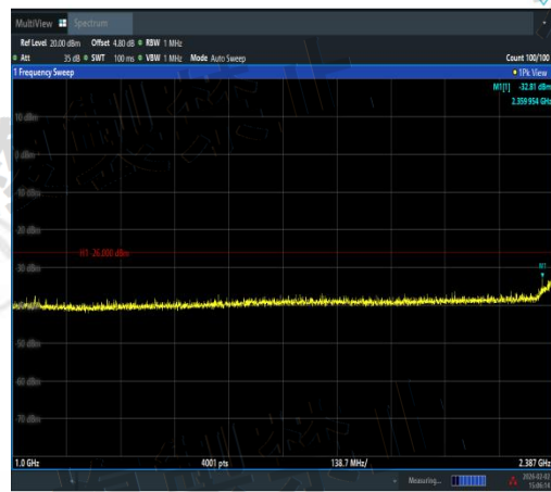
NTNV-11N40SISO-Ant1-2422-1000~2387-PASS
