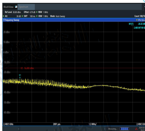
NTNV-11N40MIMO-Ant2-2442-2483.5~2496.5-P ASS
