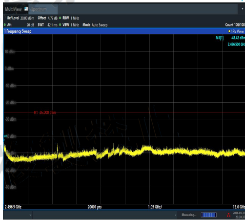
NTVN-11AX20SISO-Ant1-2412-2496.5~13000-P ASS
