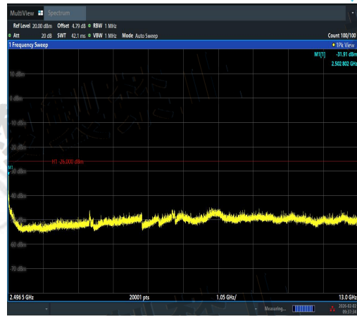
NTVN-11AX20SISO-Ant2-2472-2496.5~13000-P ASS
