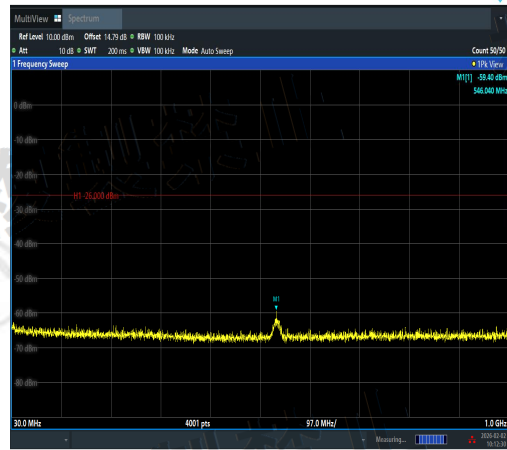
NTVN-11N20MIMO-Ant2-2472-30~1000-PASS
