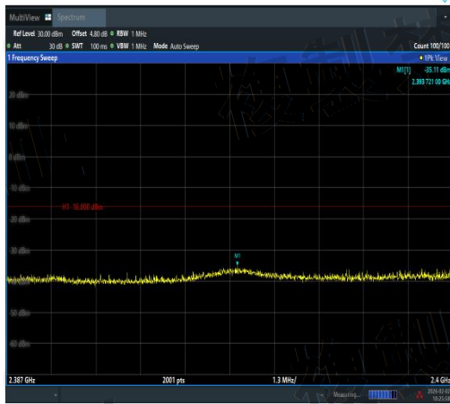
NTVN-11N40MIMO-Ant1-2442-2387~2400-See table below
