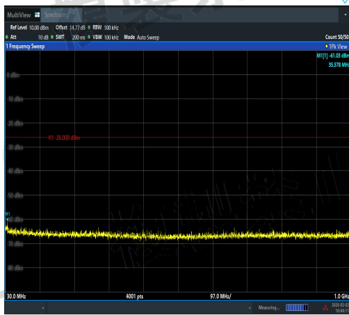
NTVN-11AX20MIMO-Ant1-2412-30~1000-PASS
