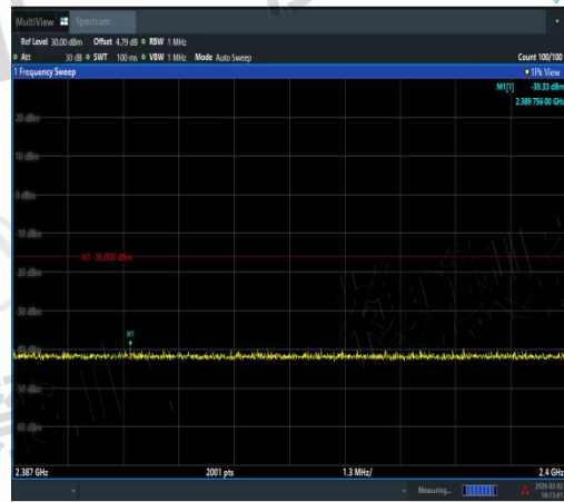
NTVN-11N20MIMO-Ant2-2472-2387~2400-PASS
