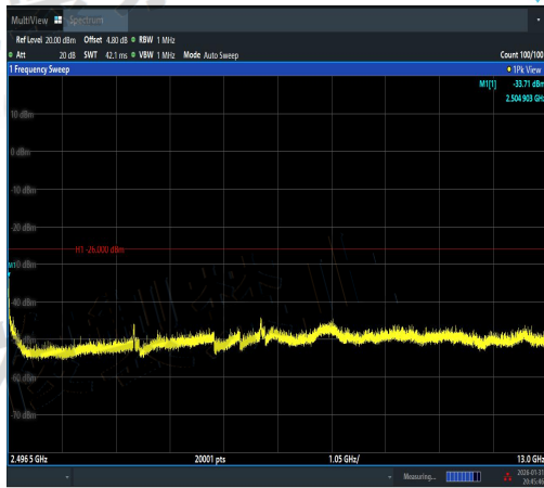
NTVN-11AX20SISO-Ant1-2472-2496.5~13000-P ASS
