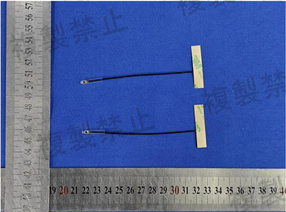
View of Product-10 (Antenna: 1001932PT)
