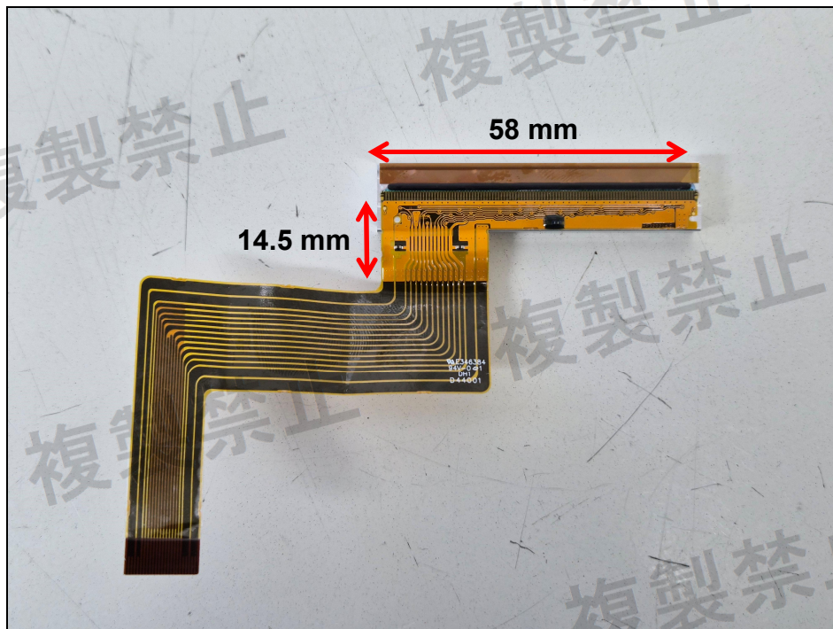
Top view of Sub PCB 4
