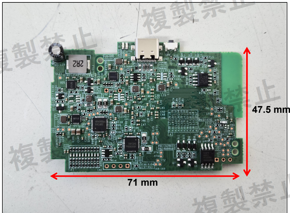
Top view of Main PCB
