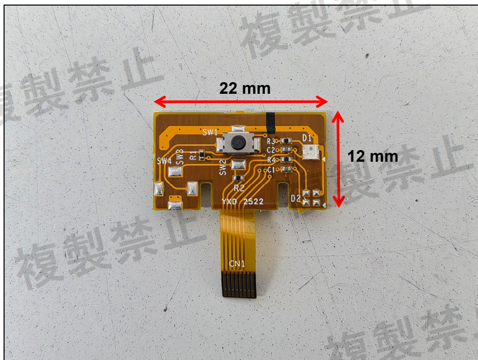
Top view of Sub PCB 1
