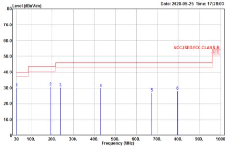
BLE Receiver Mode Vertical (30 MHz – 1GHz)
