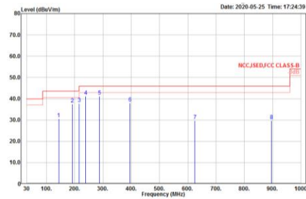
BLE Receiver Mode Horizontal (30 MHz – 1GHz)
