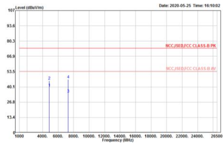
BLE Receiver Mode Vertical (1 GHz – 26.5GHz)
