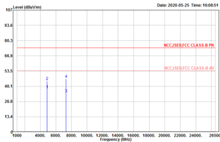
BLE Receiver Mode Horizontal (1 GHz – 26.5GHz)
