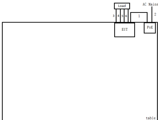
Test Setup Diagram – AC Line Conducted Emission Test (RX)
