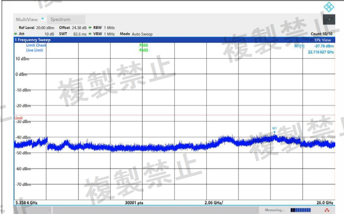
NTNV-11BE40MIMO-Ant2-5270-5358.4~26000-PASS
