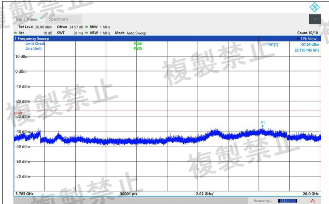
NTNV-11BE20MIMO-Ant1-5500-5765~26000-PASS
