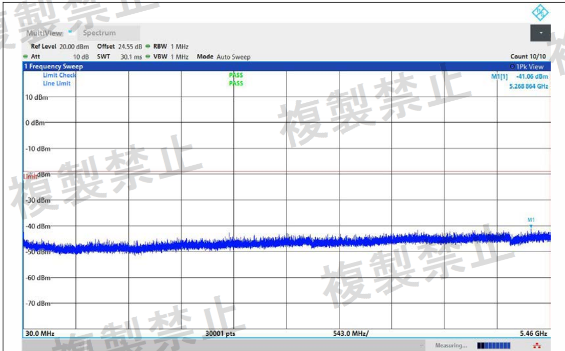
NTNV-11BE40MIMO-Ant1-5670-30~5460-PASS
