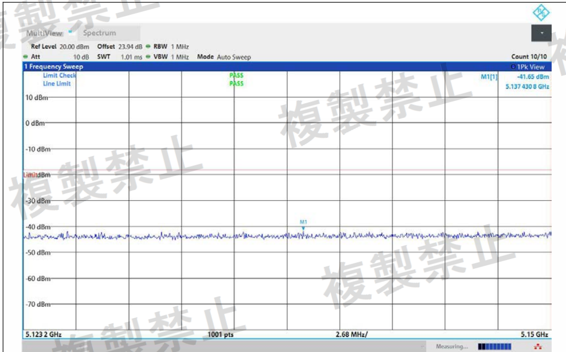
NTNV-11BE80MIMO-Ant1-5210-5123.2~5150-PASS
