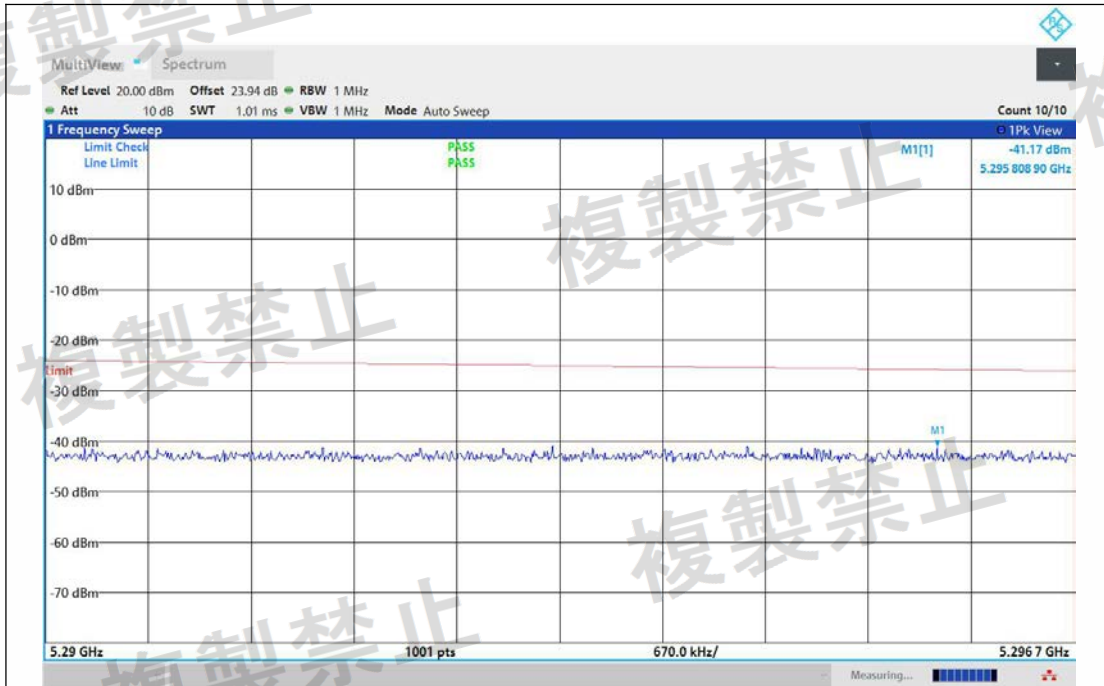
NTNV-11BE80MIMO-Ant1-5210-5290~5296.7-PASS
