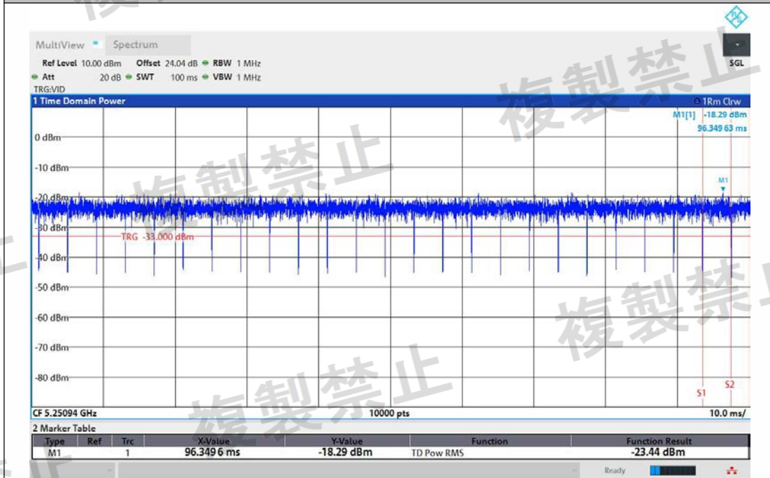
NTNV-11N20MIMO-Ant2-5240-5250~5251-PASS
