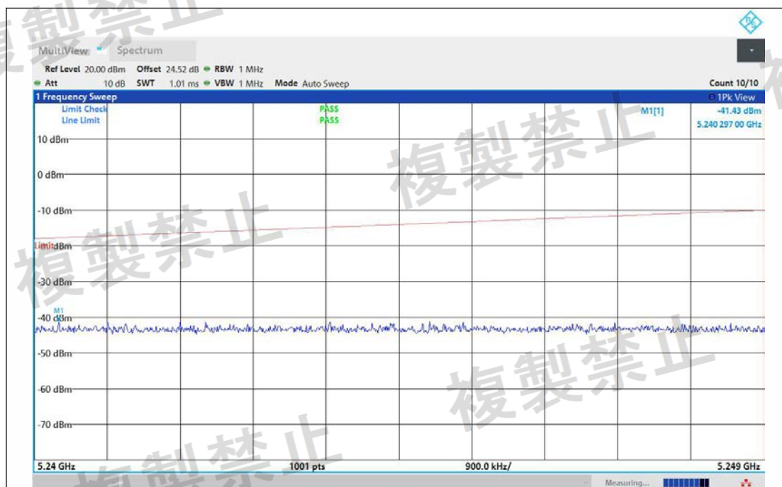
NTNV-11BE20MIMO-Ant1-5320-5240~5249-PASS
