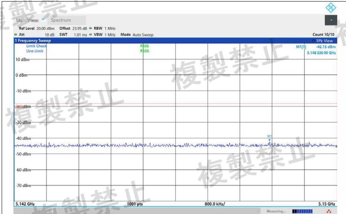
NTNV-11BE20MIMO-Ant1-5240-5142~5150-PASS
