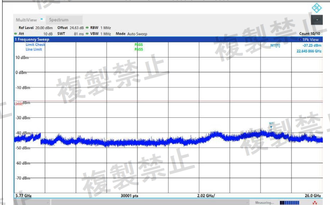
NTNV-11BE80MIMO-Ant2-5530-5770~26000-PASS
