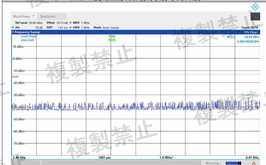
NTNV-11BE40MIMO-Ant2-5510-5460~5470-PASS
