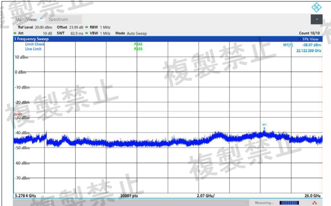
NTNV-11BE40MIMO-Ant1-5230-5278.4~26000-PASS
