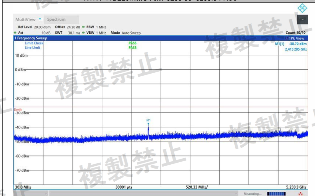
NTNV-11BE20MIMO-Ant2-5280-30~5233.3-PASS
