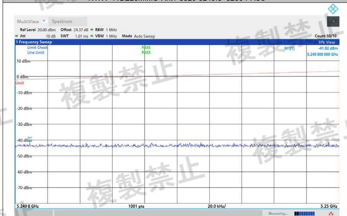
NTNV-11BE20MIMO-Ant2-5320-5249.8~5250-PASS
