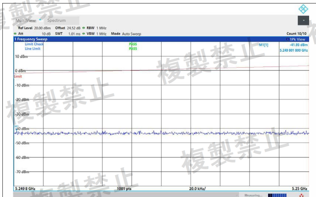
NTNV-11BE20MIMO-Ant1-5320-5249.8~5250-PASS
