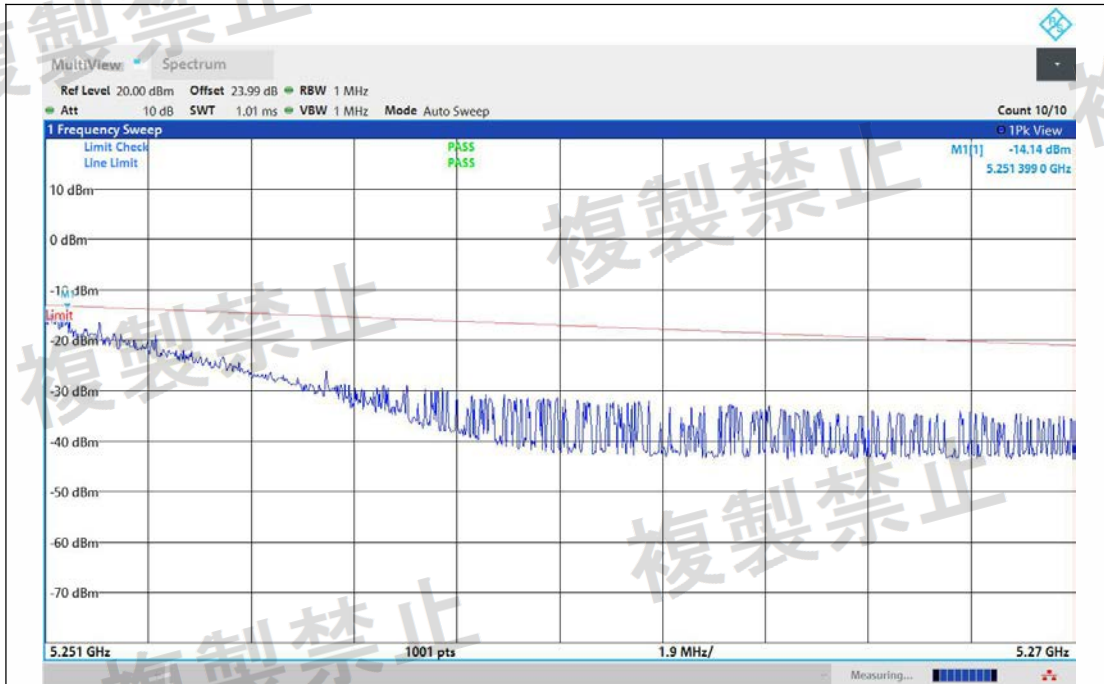
NTNV-11BE40MIMO-Ant1-5230-5251~5270-PASS
