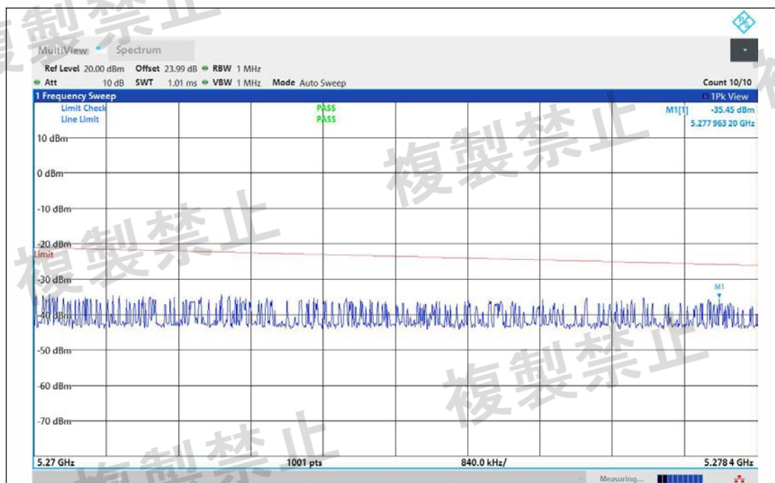
NTNV-11BE40MIMO-Ant1-5230-5270~5278.4-PASS
