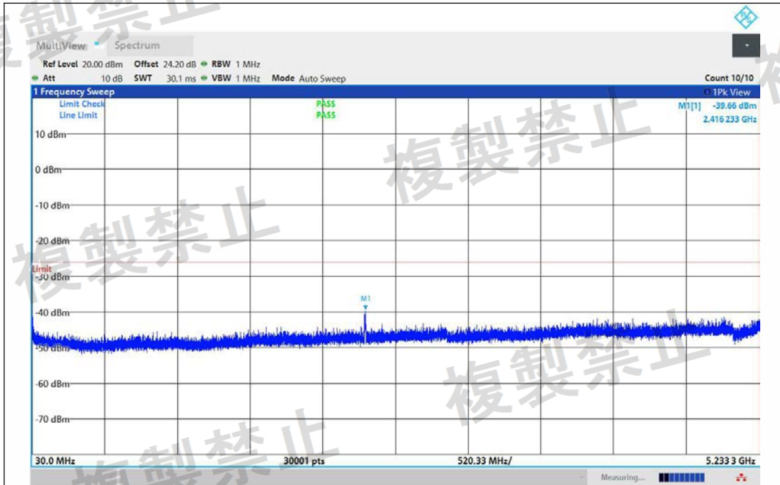
NTNV-11BE20MIMO-Ant1-5260-30~5233.3-PASS
