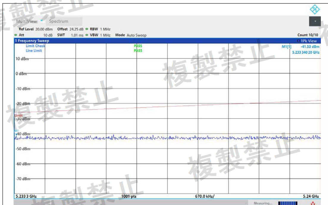
NTNV-11BE20MIMO-Ant1-5280-5233.3~5240-PASS
