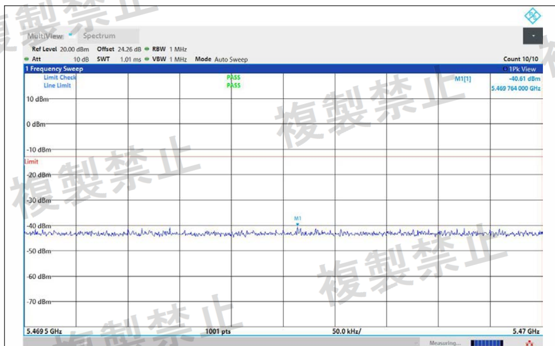
NTNV-11BE80MIMO-Ant1-5610-5469.5~5470-PASS
