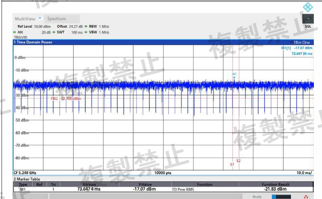
NTNV-11A-Ant2-5260-5249~5250-PASS
