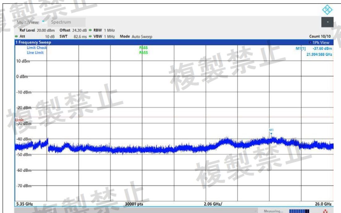
NTNV-11BE20MIMO-Ant1-5260-5350~26000-PASS
