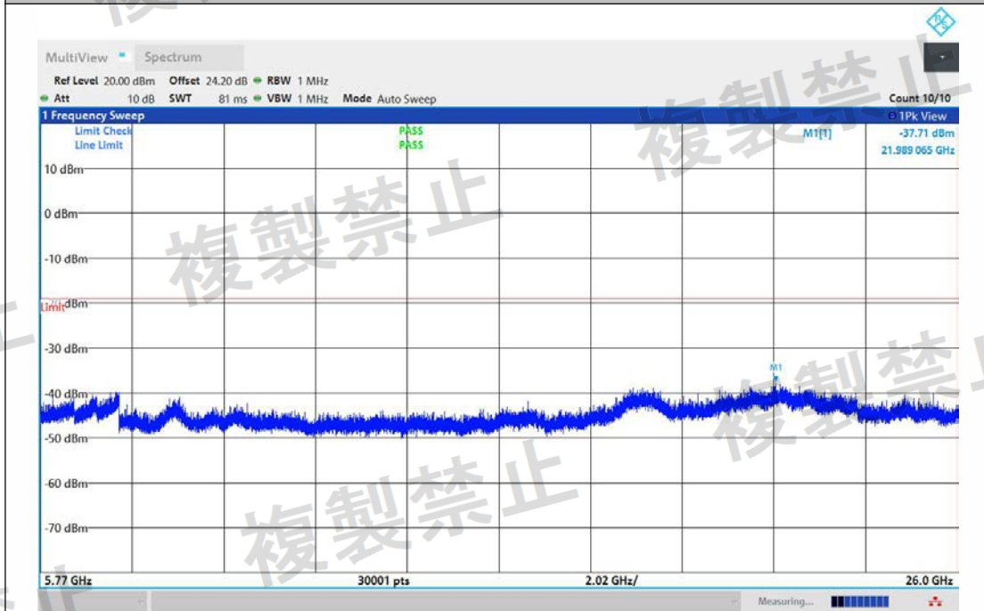
NTNV-11BE80MIMO-Ant2-5610-5770~26000-PASS
