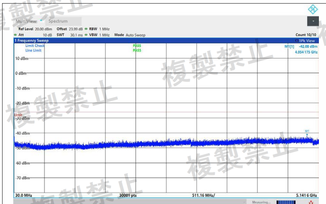
NTNV-11BE40MIMO-Ant1-5230-30~5141.6-PASS
