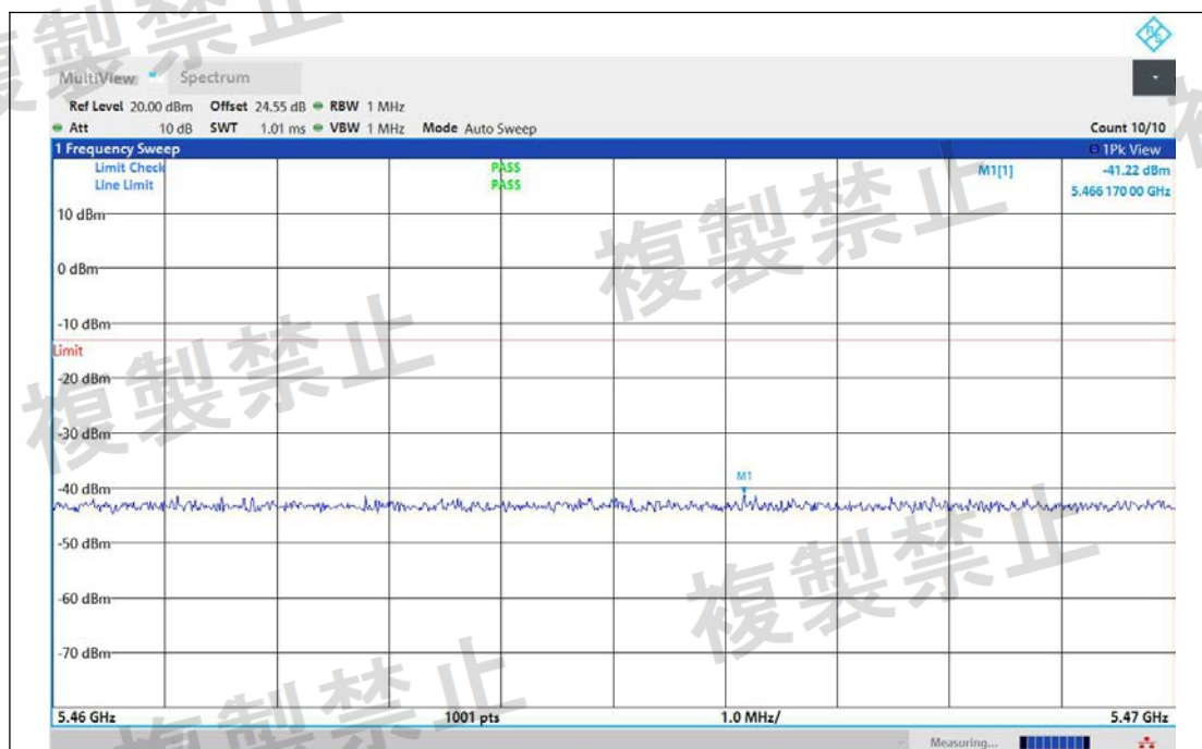
NTNV-11BE40MIMO-Ant1-5670-5460~5470-PASS
