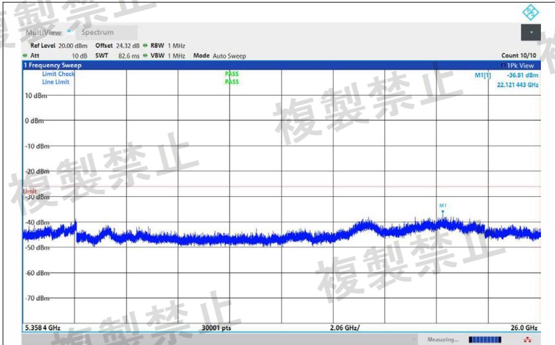
NTNV-11BE40MIMO-Ant1-5270-5358.4~26000-PASS
