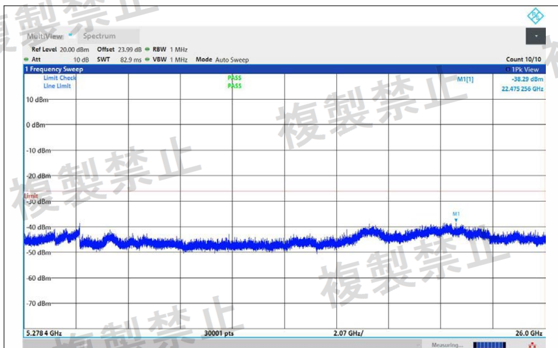
NTNV-11BE40MIMO-Ant1-5190-5278.4~26000-PASS
