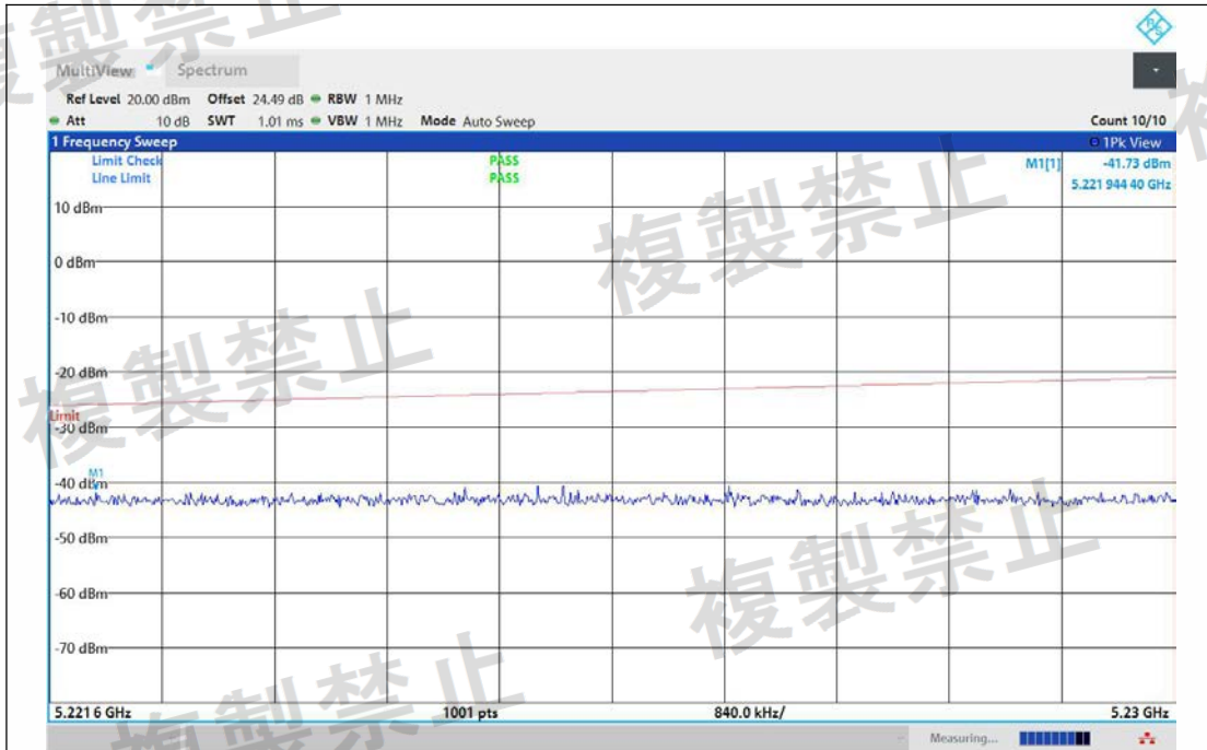
NTNV-11BE40MIMO-Ant1-5310-5221.6~5230-PASS
