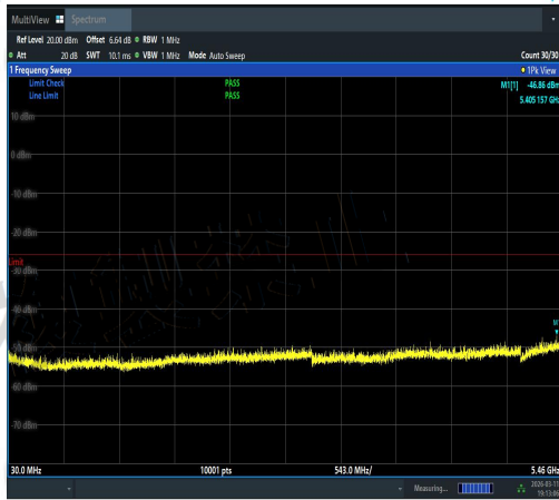
NTNV-11N20MIMO-Ant3-5600-30~5460-PASS
