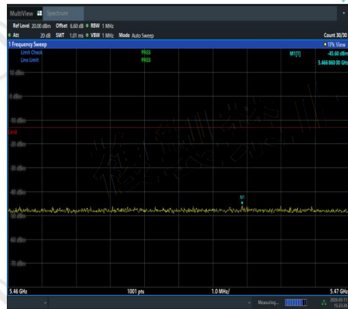
NTNV-11N40SISO-Ant2-5710-5460~5470-PASS
