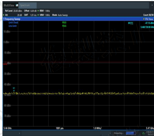
NTNV-11N20MIMO-Ant3-5600-5460~5470-PASS
