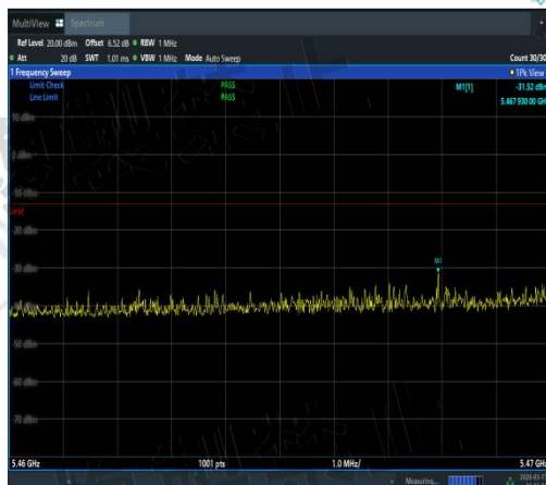
NTNV-11N40SISO-Ant2-5550-5460~5470-PASS
