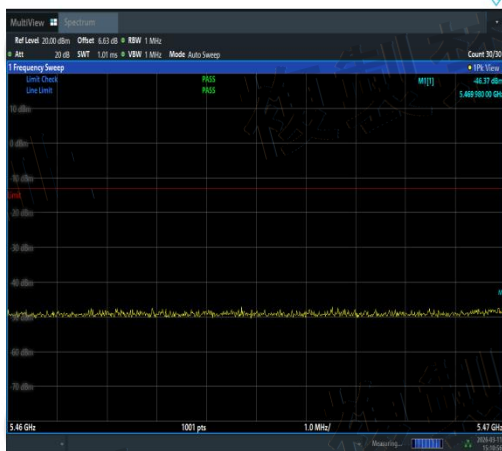
NTNV-11N40SISO-Ant3-5710-5460~5470-PASS
