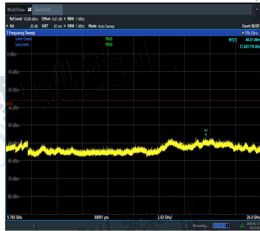
NTNV-11N20SISO-Ant3-5500-5765~26000-PAS
