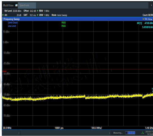
NTNV-11N20MIMO-Ant3-5700-30~5460-PASS
