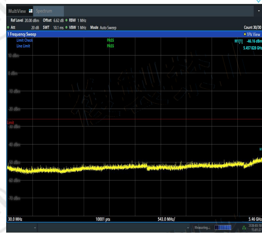
NTNV-11N20SISO-Ant2-5700-30~5460-PASS
