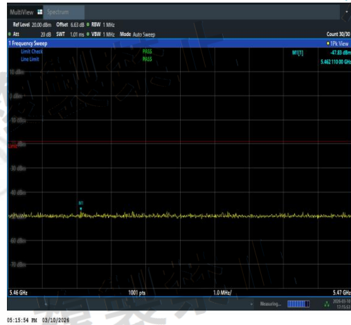
NTNV-11N20SISO-Ant3-5720-5460~5470-PASS
