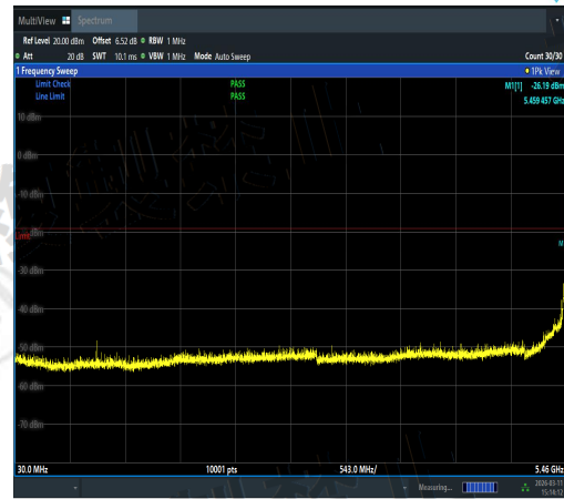
NTVN-11N40SISO-Ant2-5510-30~5460-PASS
