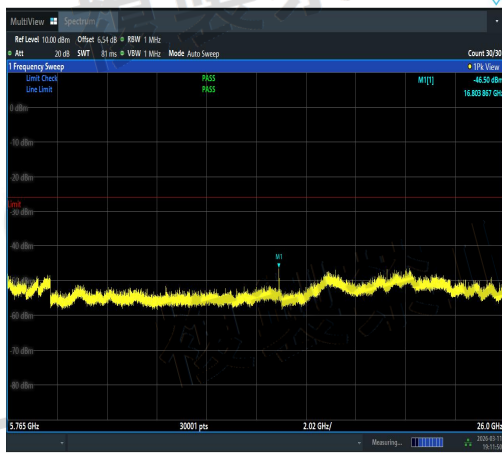
NTNV-11N20MIMO-Ant2-5600-5765~26000-PAS S
