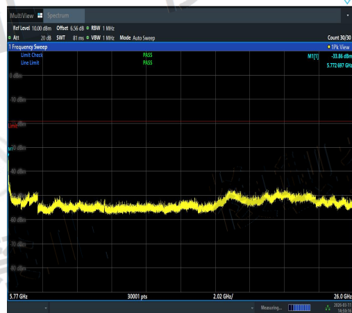
NTNV-11N40SISO-Ant1-5710-5770~26000-PASS
