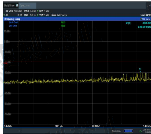
NTNV-11AC20MIMO-Ant3-5500-5460~5470-PAS
