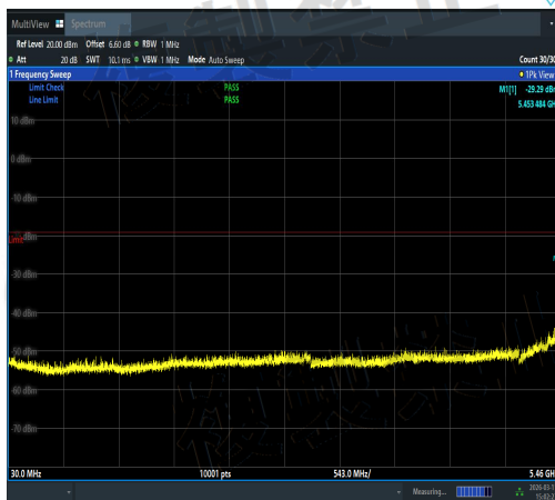
NTVN-11N40SISO-Ant3-5510-30~5460-PASS
