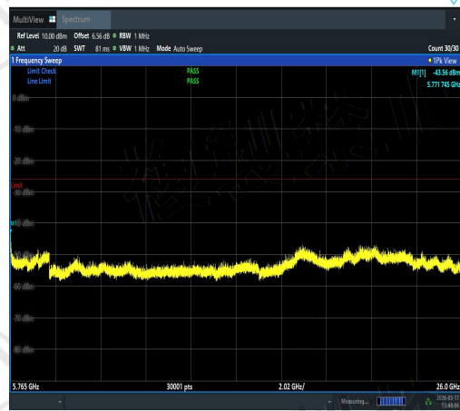
NTVN-11A-Ant1-5720-5765~26000-PASS
