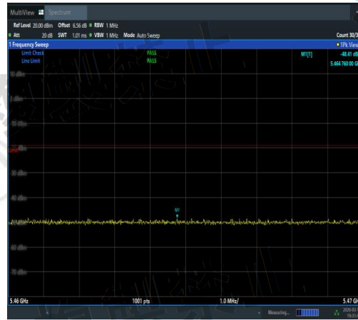
NTNV-11N20MIMO-Ant1-5720-5460~5470-PASS
