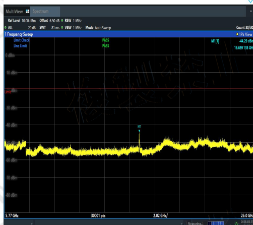
NTNV-11N40SISO-Ant1-5550-5770~26000-PAS S
