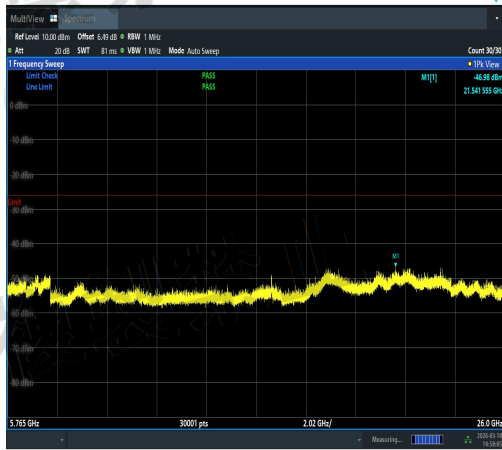
NTNV-11N20SISO-Ant2-5500-5765~26000-PAS
