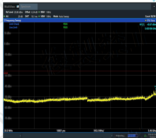
NTNV-11N20SISO-Ant2-5600-30~5460-PASS
