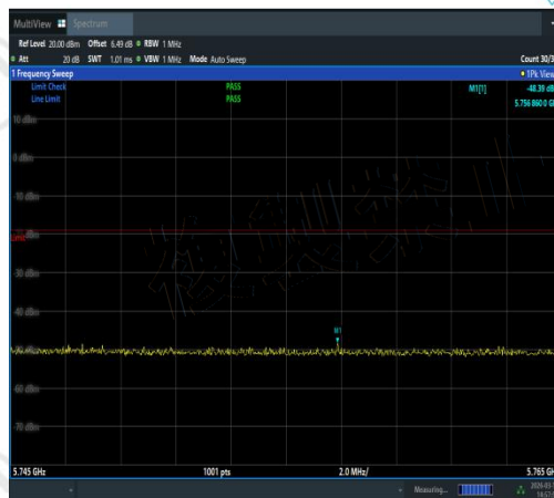
NTNV-11N20SISO-Ant2-5500-5745~5765-PASS
