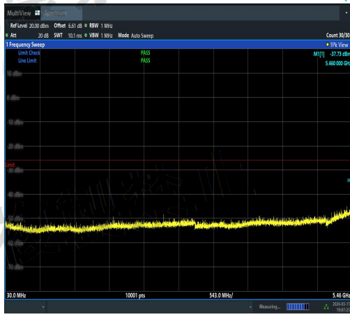
NTVN-11N20MIMO-Ant3-5500-30~5460-PASS
