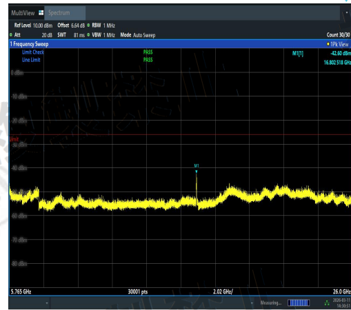
NTNV-11N20SISO-Ant3-5600-5765~26000-PAS S
