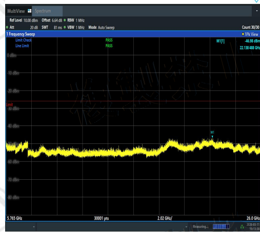
NTNV-11N20MIMO-Ant3-5600-5765~26000-PAS S
