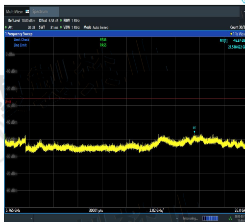
NTNV-11AC20SISO-Ant1-5700-5765~26000-PA SS
