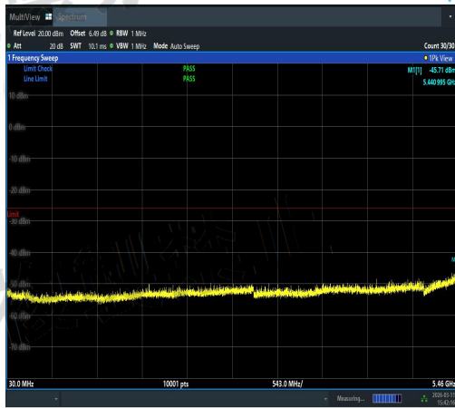
NTNV-11AC20SISO-Ant1-5600-30~5460-PASS
