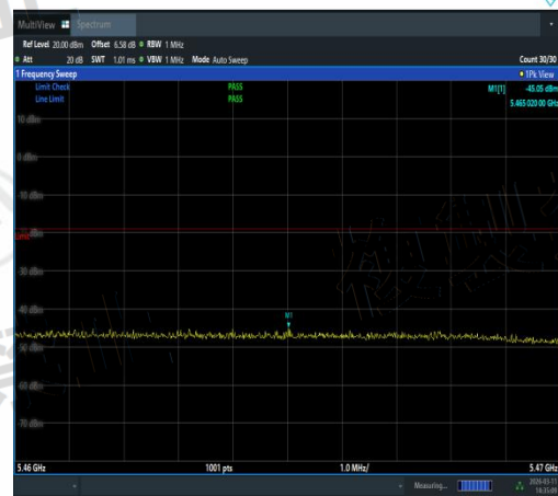
NTNV-11N20SISO-Ant1-5700-5460~5470-PASS
