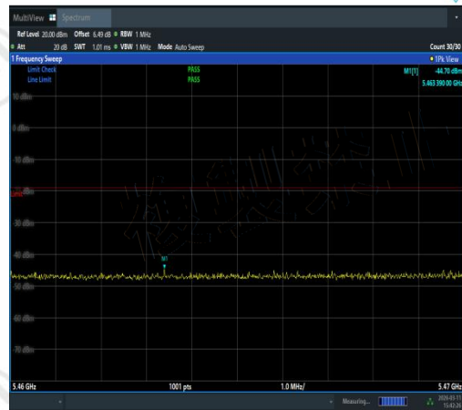
NTNV-11AC20SISO-Ant1-5600-5460~5470-PAS S
