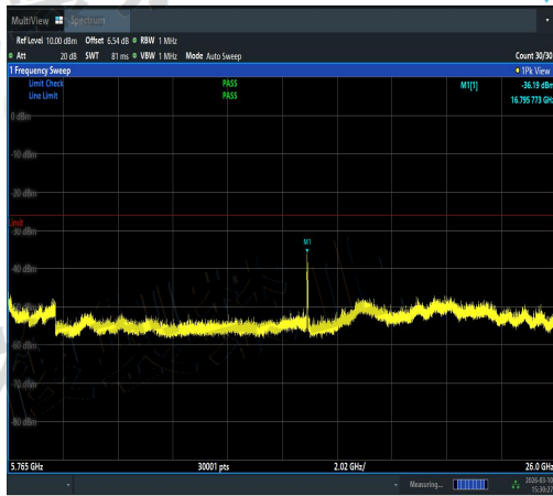
NTVN-11AC20SISO-Ant2-5600-5765~26000-PA SS
