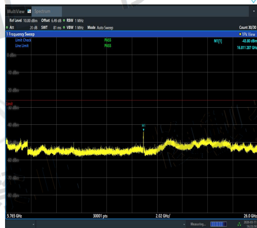
NTNV-11N20SISO-Ant1-5600-5765~26000-PAS S
