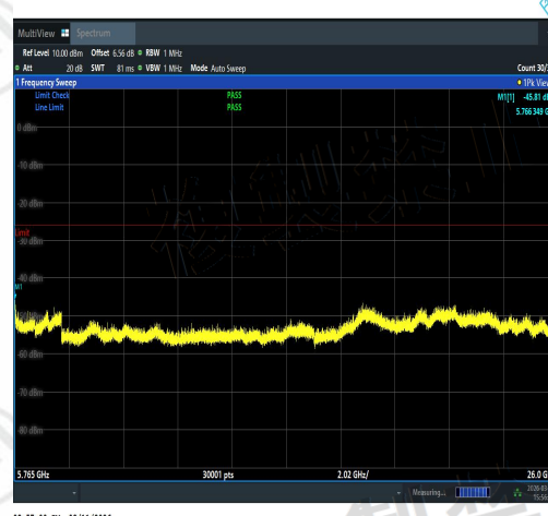
NTNV-11AC20SISO-Ant1-5720-5765~26000-PA SS
