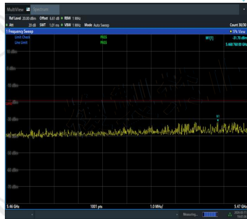
NTVN-11N20MIMO-Ant3-5500-5460~5470-PASS
