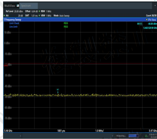
NTNV-11AC20MIMO-Ant3-5600-5460~5470-PAS S
