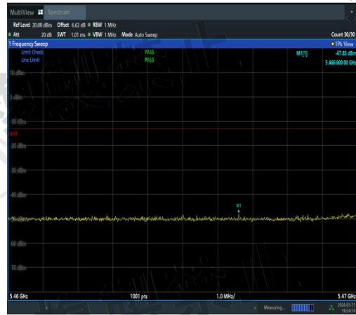
NTNV-11N40MIMO-Ant3-5670-5460~5470-PASS
