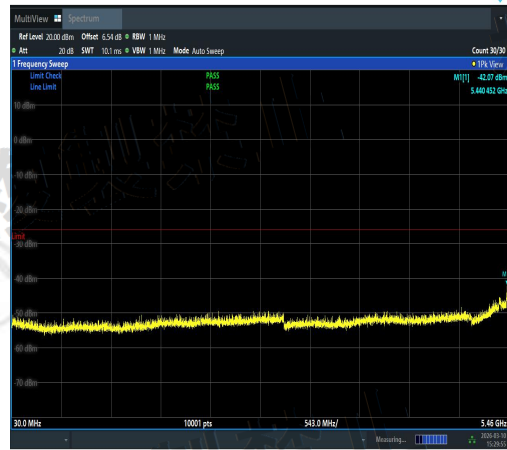
NTNV-11AC20SISO-Ant2-5600-30~5460-PASS
