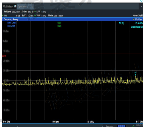
NTNV-11N40SISO-Ant1-5550-5460~5470-PASS
