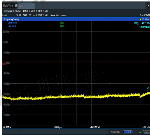
NTNV-11N40SISO-Ant2-5710-30~5460-PASS
