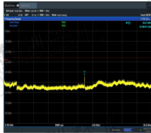
NTVN-11AC20SISO-Ant3-5600-5765~26000-PA SS
