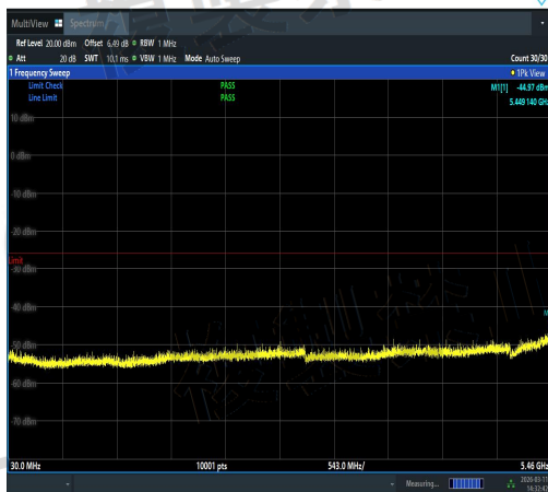
NTNV-11N20SISO-Ant1-5600-30~5460-PASS
