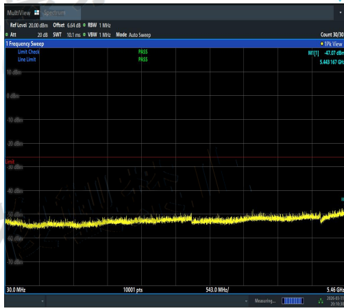
NTNV-11AC20MIMO-Ant3-5600-30~5460-PASS
