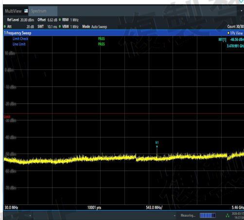
NTNV-11N20SISO-Ant3-5700-30~5460-PASS
