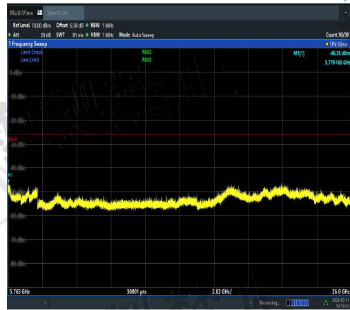
NTNV-11N20MIMO-Ant1-5700-5765~26000-PASS S
