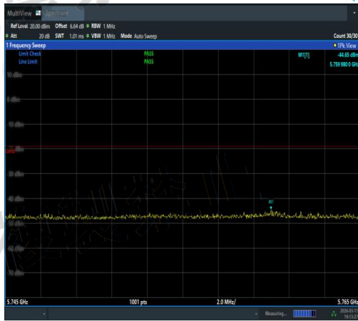
NTNV-11N20MIMO-Ant3-5600-5745~5765-PASS
