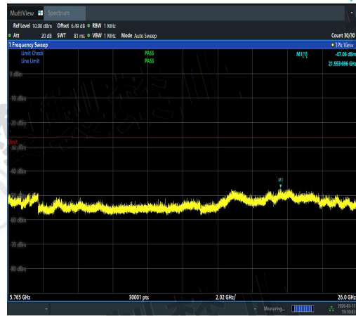
NTNV-11N20MIMO-Ant1-5600-5765~26000-PAS S
