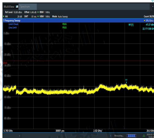
NTNV-11N20MIMO-Ant1-5500-5765~26000-PASS S
