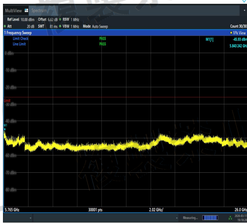
NTNV-11N20MIMO-Ant2-5700-5765~26000-PASS S
