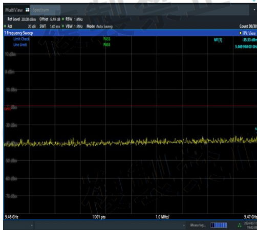
NTVN-11N20MIMO-Ant2-5500-5460~5470-PASS
