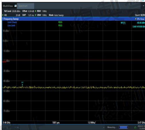
NTNV-11AC20SISO-Ant2-5600-5460~5470-PAS
