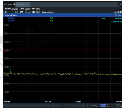
NTVN-11N20SISO-Ant3-5700-5460~5470-PASS
