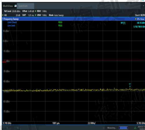
NTNV-11N20MIMO-Ant1-5600-5745~5765-PASS
