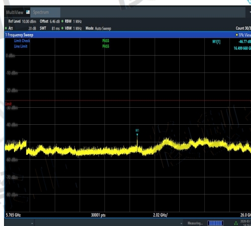
NTNV-11N20SISO-Ant1-5500-5765~26000-PASS
