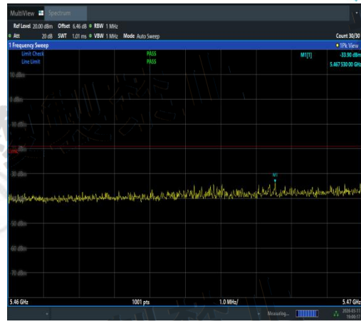
NTVN-11N20MIMO-Ant1-5500-5460~5470-PASS
