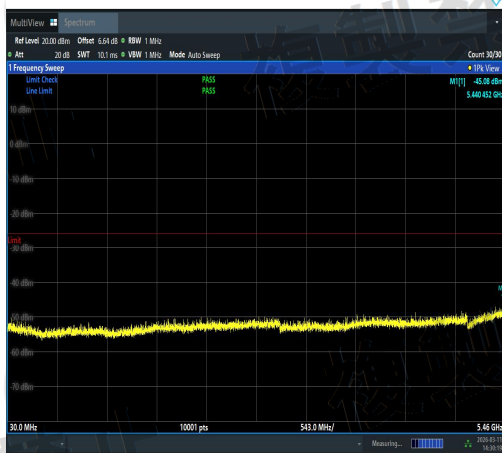
NTNV-11N20SISO-Ant3-5600-30~5460-PASS
