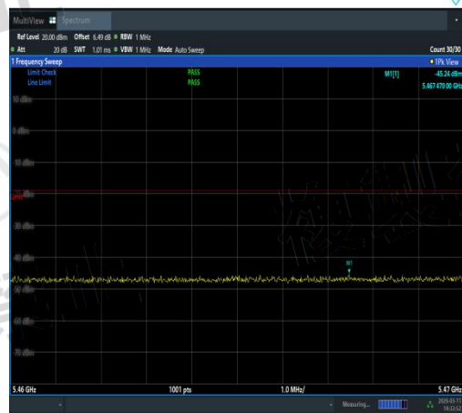
NTNV-11N20SISO-Ant1-5600-5460~5470-PASS
