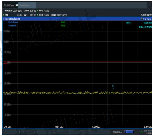
NTNV-11N20MIMO-Ant1-5600-5460~5470-PASS
