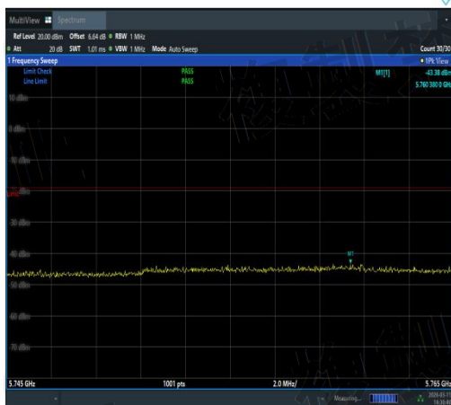
NTNV-11N20SISO-Ant3-5600-5745~5765-PASS
