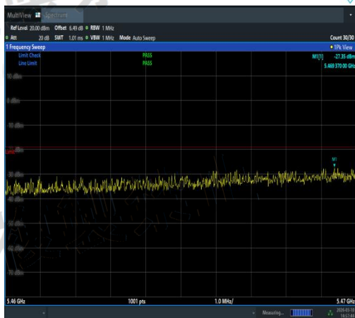
NTNV-11N20SISO-Ant2-5500-5460~5470-PASS
