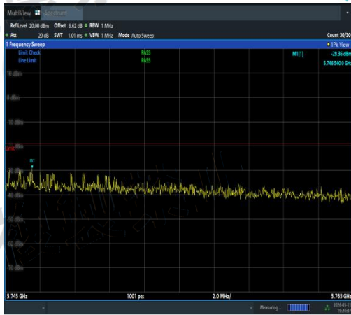
NTNV-11N20MIMO-Ant3-5700-5745~5765-PASS
