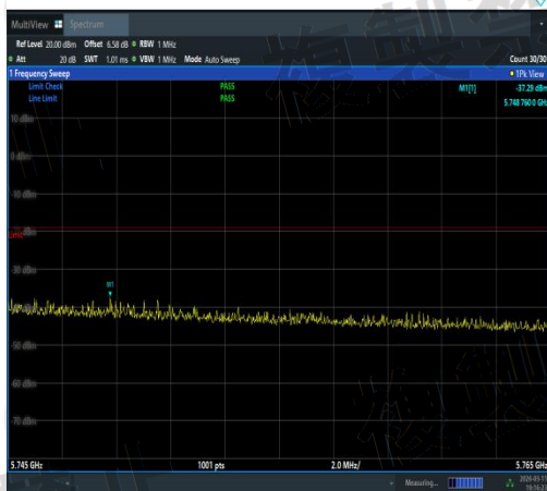
NTNV-11N20MIMO-Ant1-5700-5745~5765-PASS
