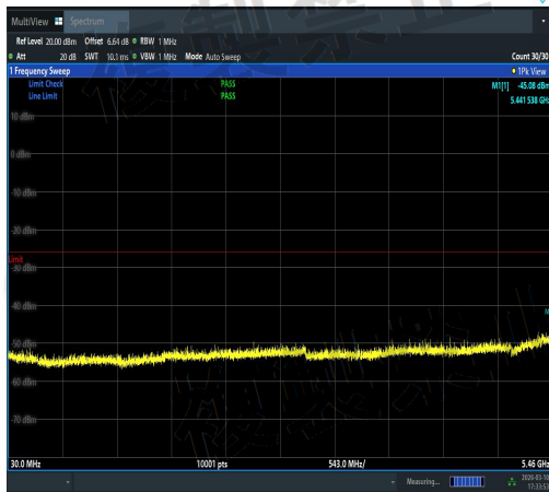
NTNV-11AC20SISO-Ant3-5600-30~5460-PASS
