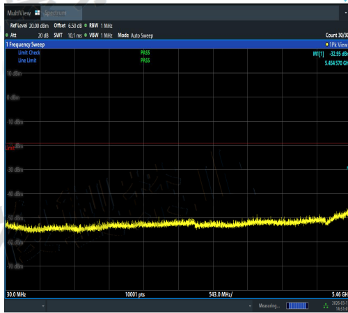
NTVN-11N40SISO-Ant1-5510-30~5460-PASS
