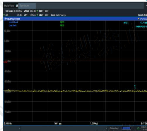
NTNV-11N20MIMO-Ant3-5700-5460~5470-PASS
