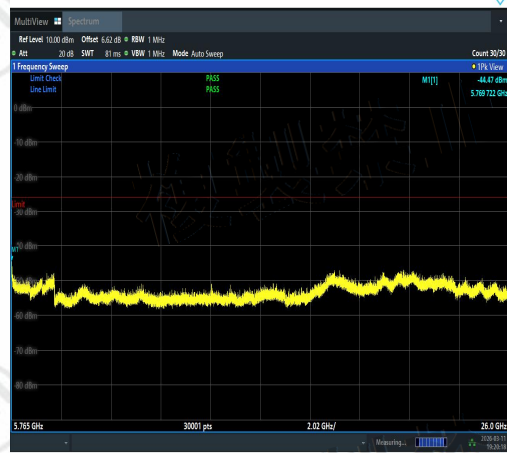
NTNV-11N20MIMO-Ant3-5700-5765~26000-PASS S
