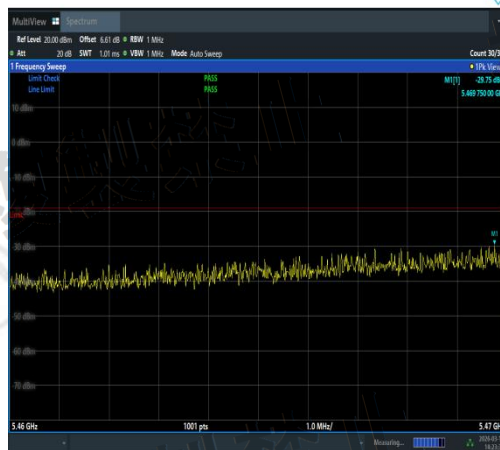
NTNV-11N20SISO-Ant3-5500-5460~5470-PASS
