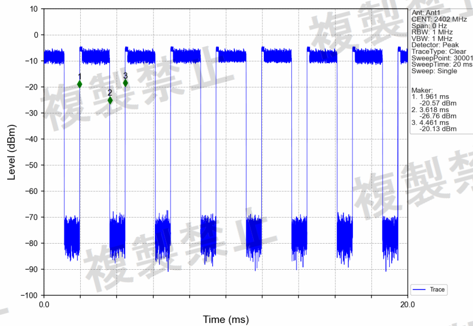
8DPSK_3DH3_2402MHz_Ant1_NTLV
