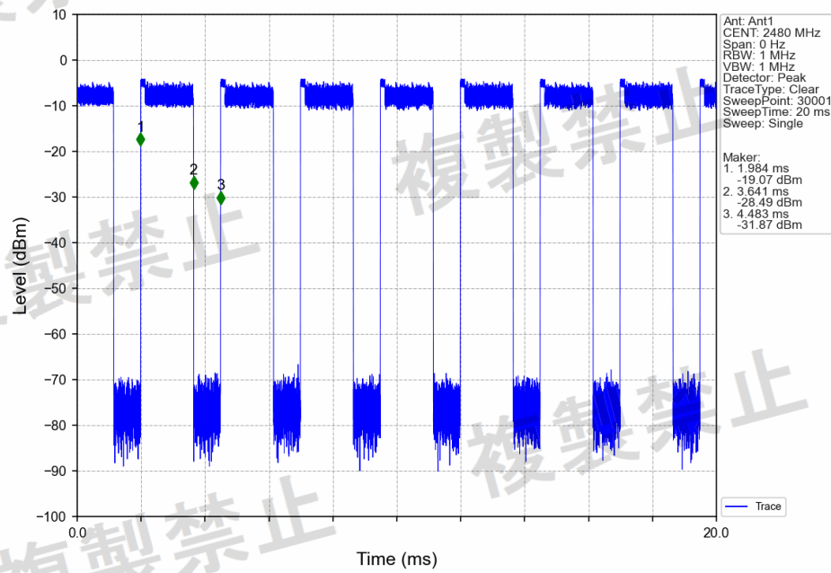
8DPSK_3DH5_2480MHz_Ant1_NTLV
