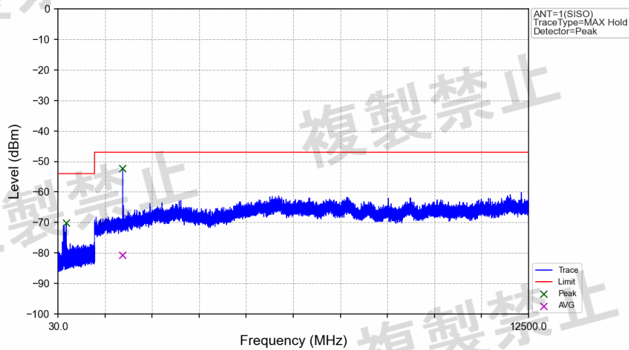
Pi/4DQPSK_2DH5_2480MHz_Ant1_NTLV
