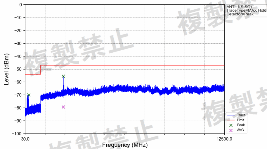
8DPSK_3DH5_2402MHz_Ant1_NTHV
