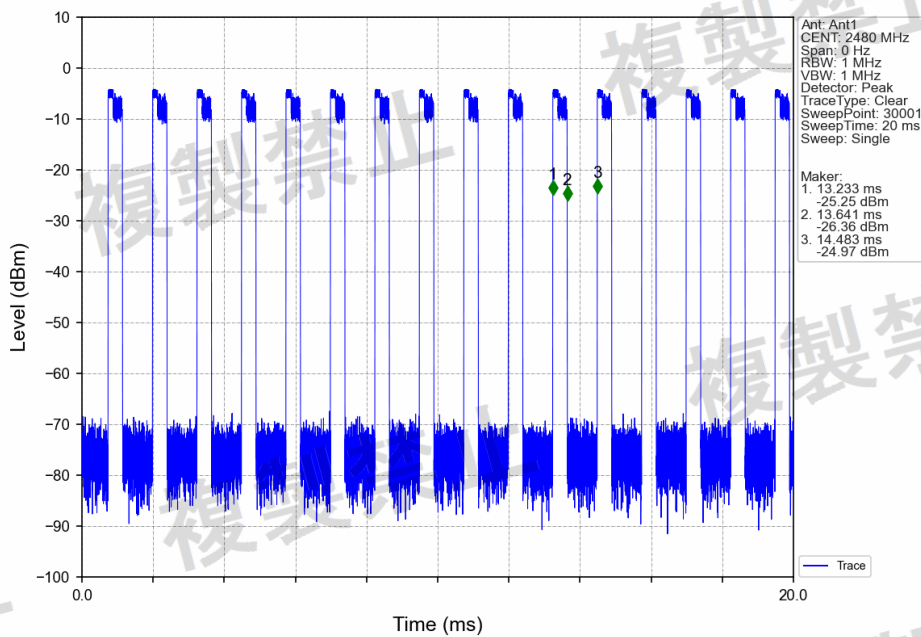
8DPSK_3DH1_2480MHz_Ant1_NTLV
