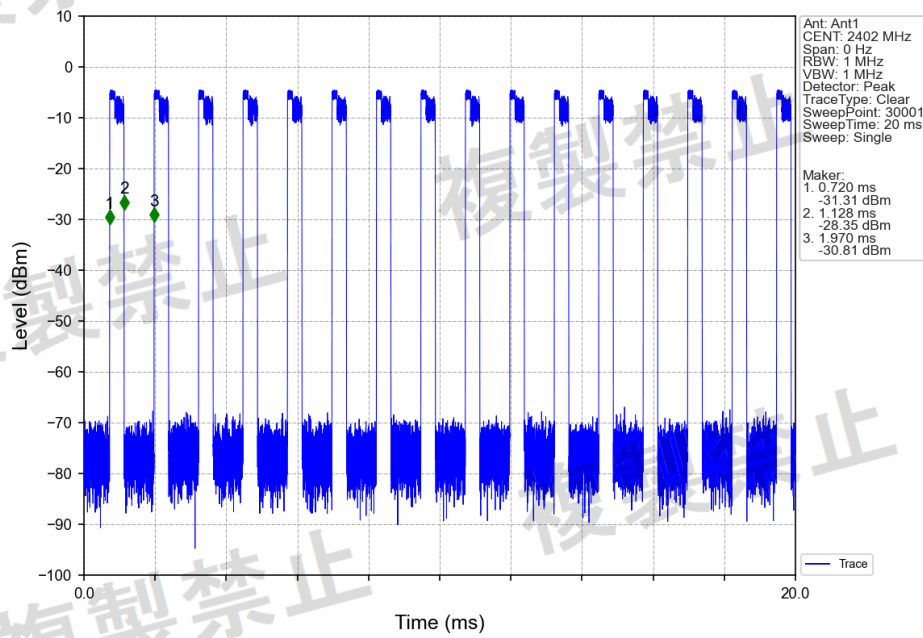
Pi/4DQPSK_2DH3_2402MHz_Ant1_NTLV
