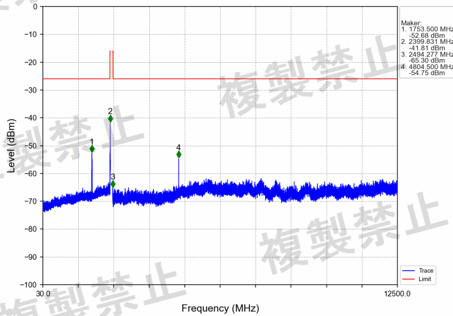
Pi/4DQPSK_2DH5_2402MHz_Ant1_NTLV
