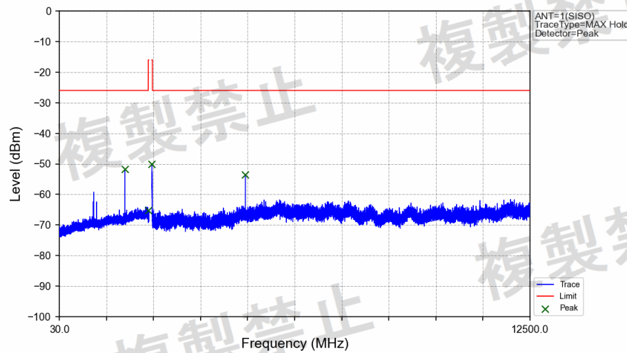
8DPSK_3DH5_2480MHz_Ant1_NTNV
