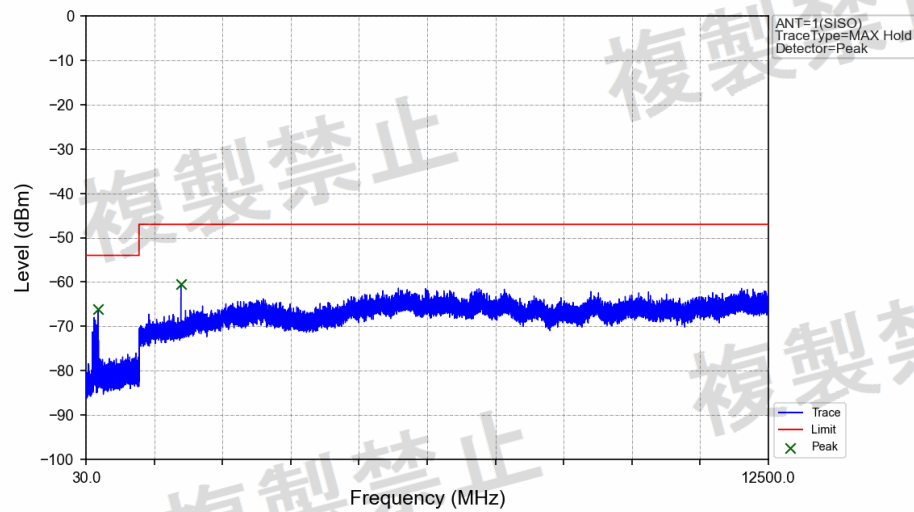
GFSK_DH5_2480MHz_Ant1_NTLV
