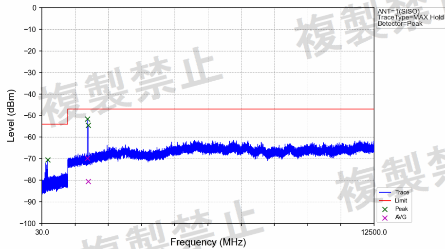
GFSK_DH5_2480MHz_Ant1_NTHV
