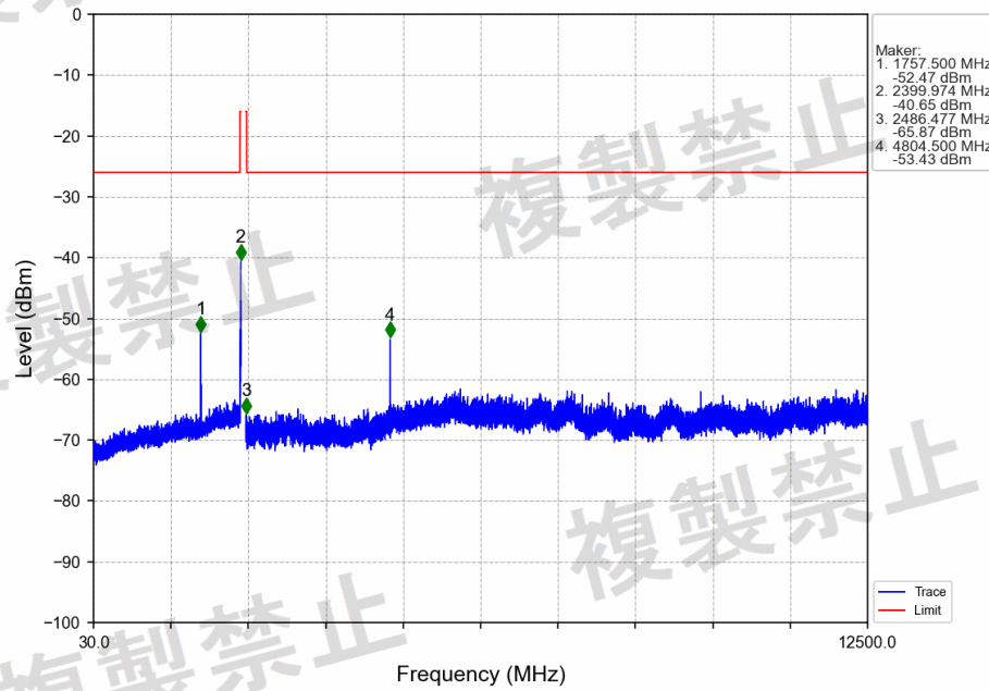
8DPSK_3DH5_2402MHz_Ant1_NTHV
