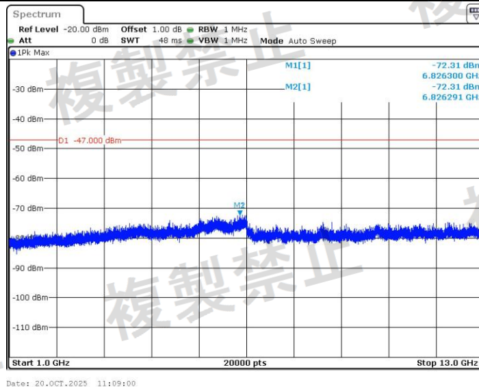
11AX20SISO_Ant1_5240_1000~13000
