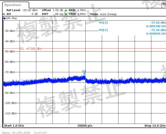
11AC20SISO_Ant1_5240_1000~13000
