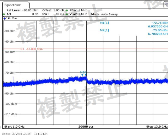
11AX40SISO_Ant2_5190_1000~13000
