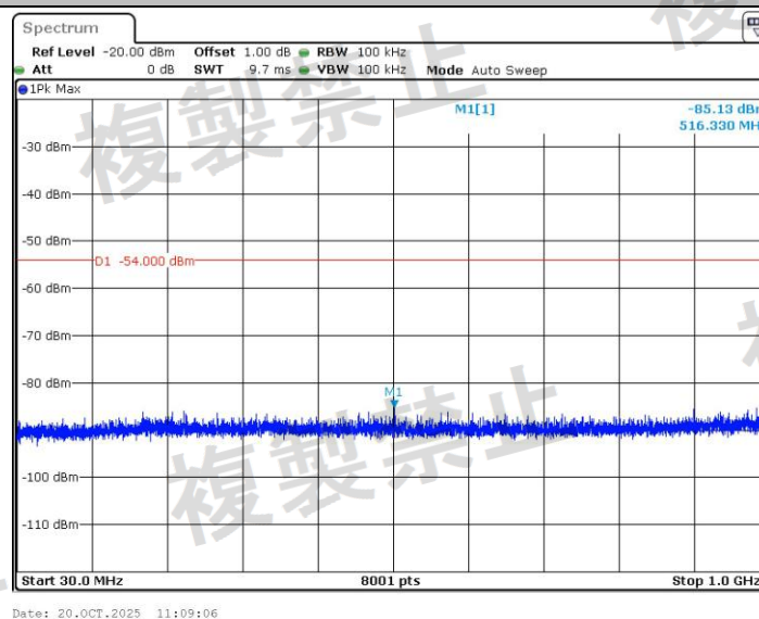
11AX40SISO_Ant1_5190_30~1000
