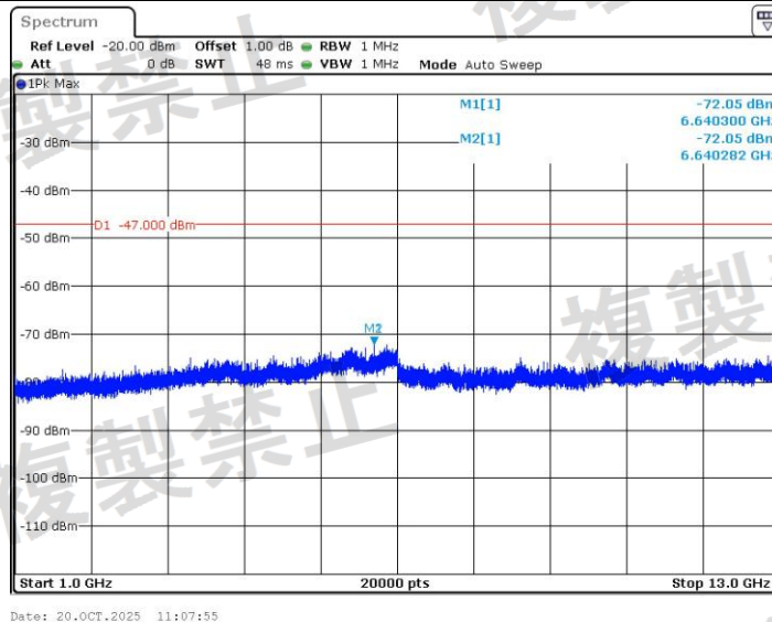
11AC40SISO_Ant1_5230_1000~13000
