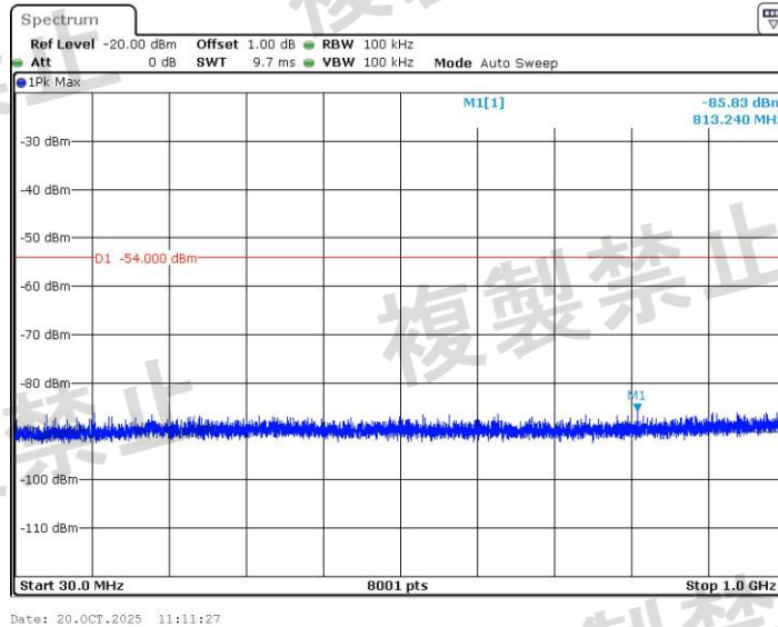
11N40SISO_Ant2_5230_30~1000
