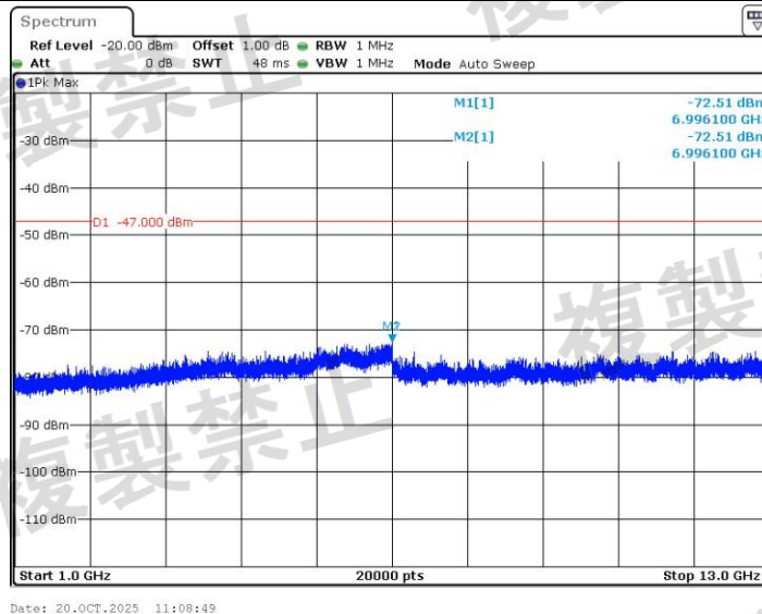
11AX20SISO_Ant1_5200_1000~13000
