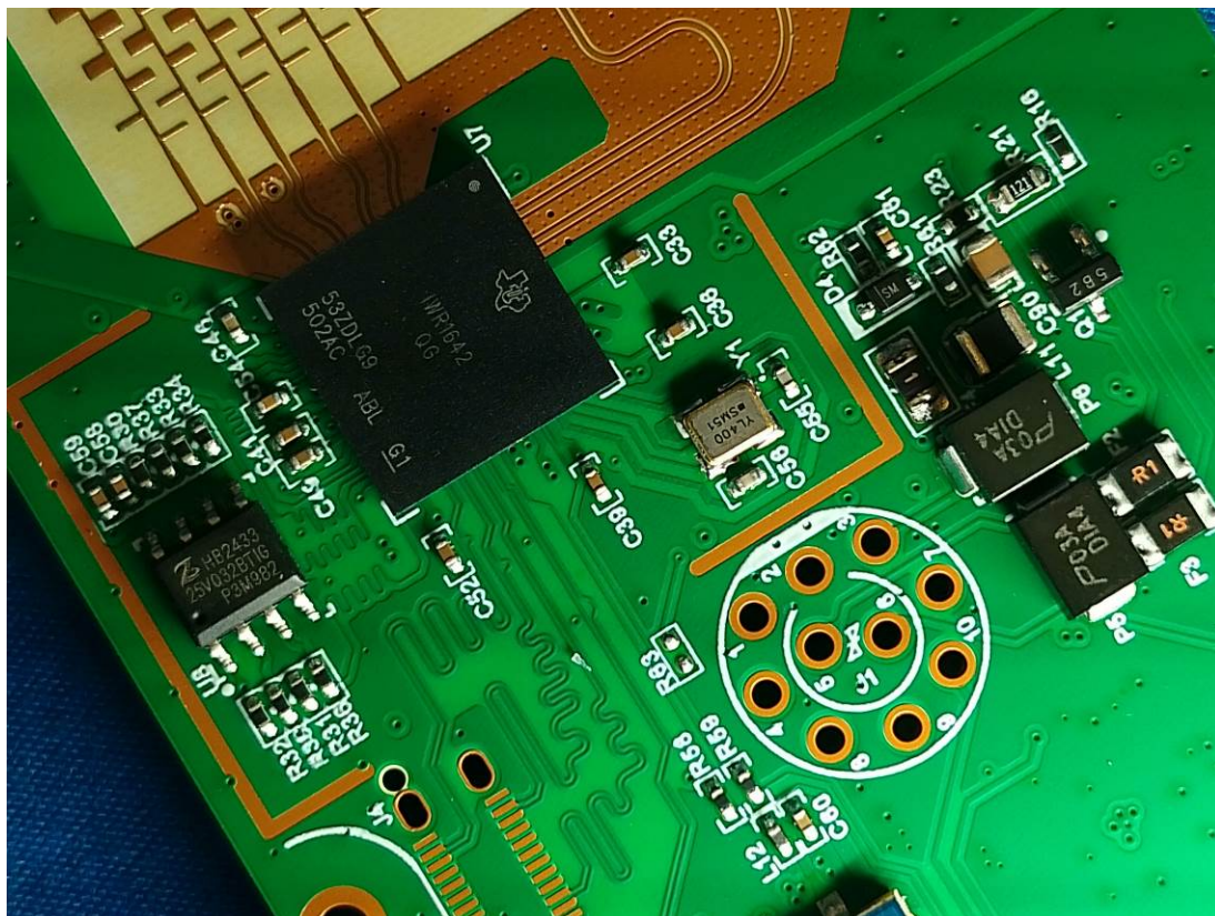
Radar Antenna (2TX4RX)
