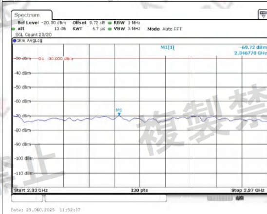
2330.0-2370.0_new Band 3 5MHz/1747.5/Mid QPSK 1@0
