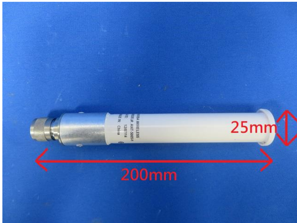
(9) EUT Photo (ANT-2X2-5005-Hpol)
