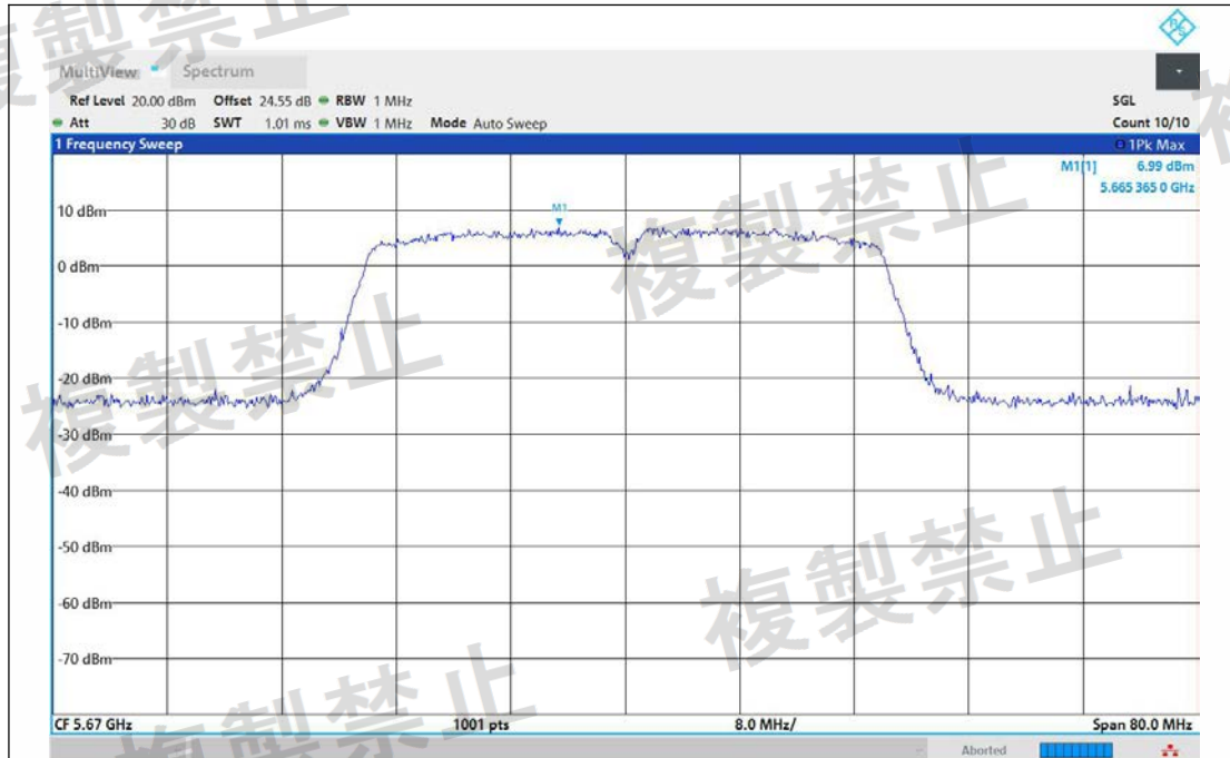
NTNV-11AC40MIMO-Ant1-5670-TPC_H-PASS
