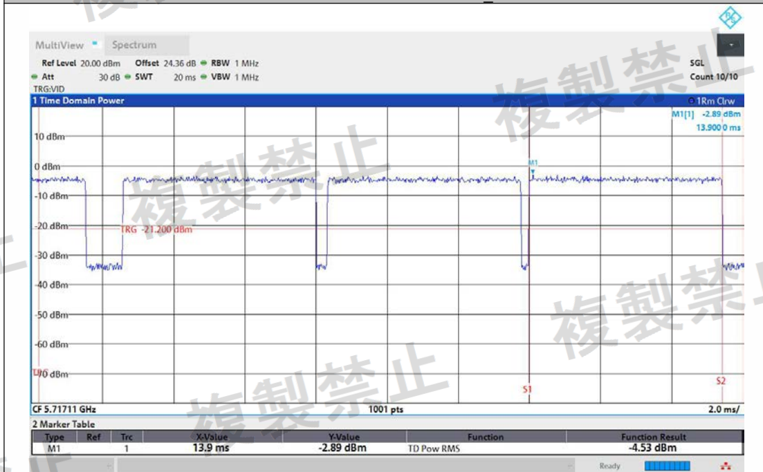
NTNV-11N40MIMO-Ant2-5710-TPC_H-PASS
