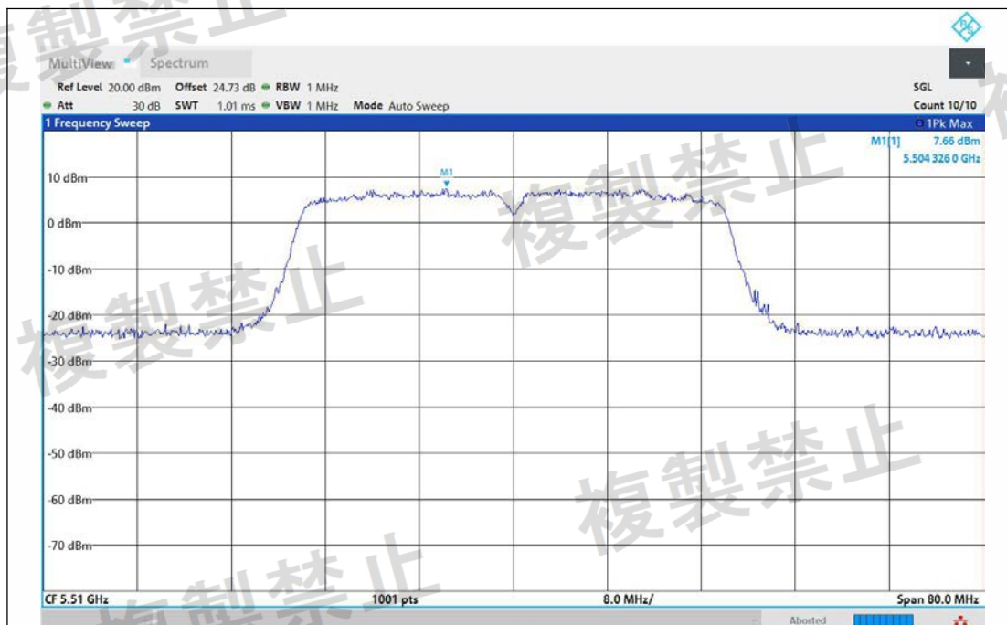
NTNV-11AC40MIMO-Ant2-5510-TPC_H-PASS
