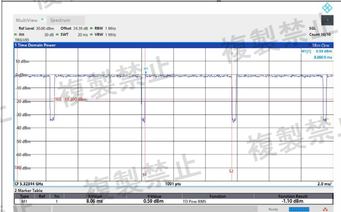
NTNV-11N20MIMO-Ant1-5320-TPC_H-PASS
