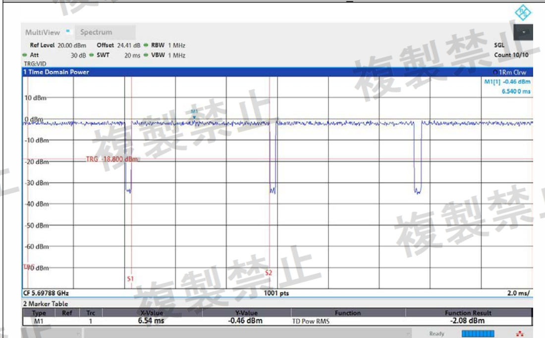
NTNV-11N20MIMO-Ant2-5700-TPC_H-PASS
