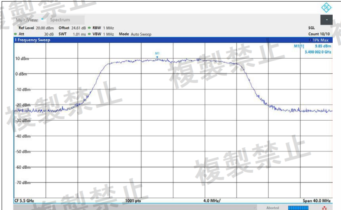
NTNV-11AC20MIMO-Ant2-5500-TPC_H-PASS
