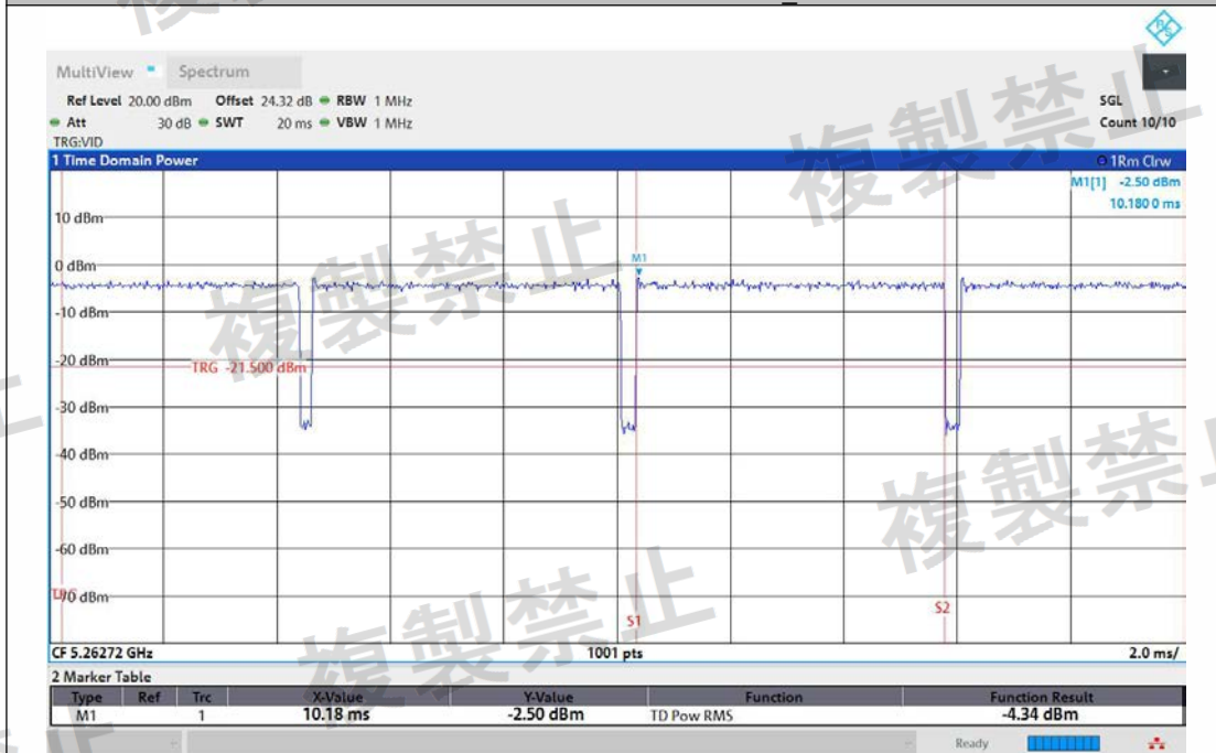
NTNV-11AC20MIMO-Ant1-5260-TPC_L-PASS
