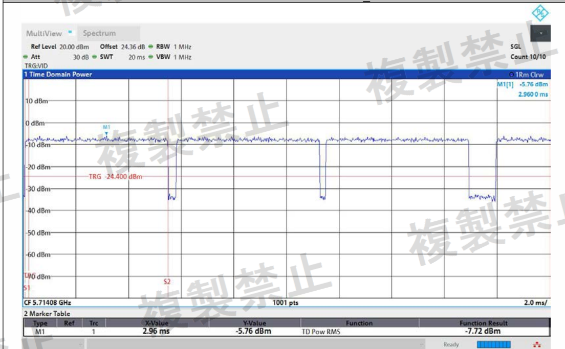
NTNV-11AC40MIMO-Ant2-5710-TPC_L-PASS
