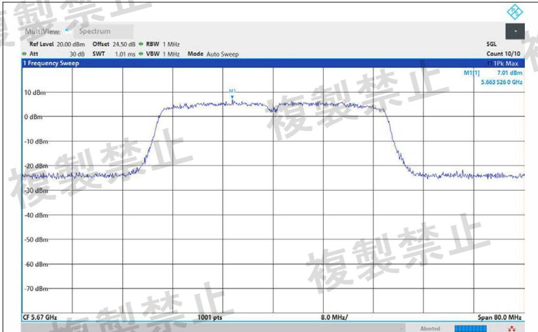
NTNV-11AC40MIMO-Ant2-5670-TPC_H-PASS
