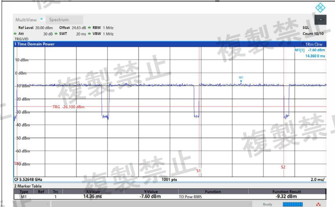
NTNV-11AC80MIMO-Ant2-5530-TPC_L-PASS
