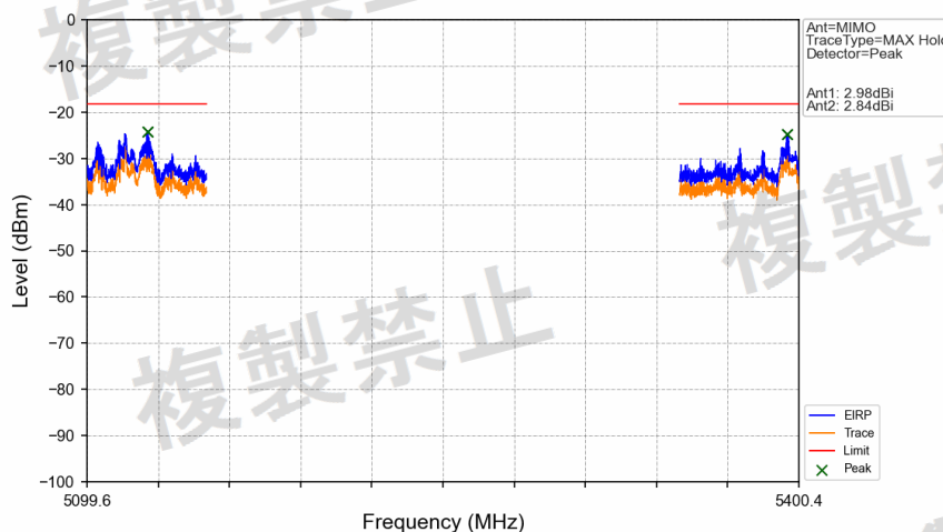
802.11ac(VHT160)_MCH_5250MHz_MIMO_NTNV
