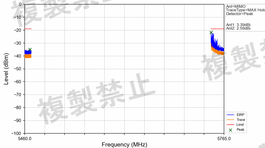
802.11ax(HEW20)_HHCH_5720MHz_RU242_Left_MIMO_NTNV
