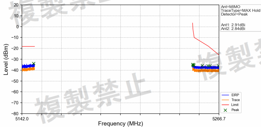
802.11ax(HEW20)_LCH_5180MHz_RU242_Left_MIMO_NTNV
