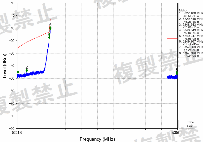
802.11ac(VHT40)_LCH_5270MHz_MIMO_NTNV
