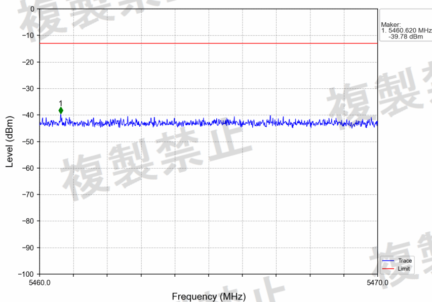
802.11ax(HEW40)_HCH_5670MHz_RU484_Left_Ant2_NTNV
