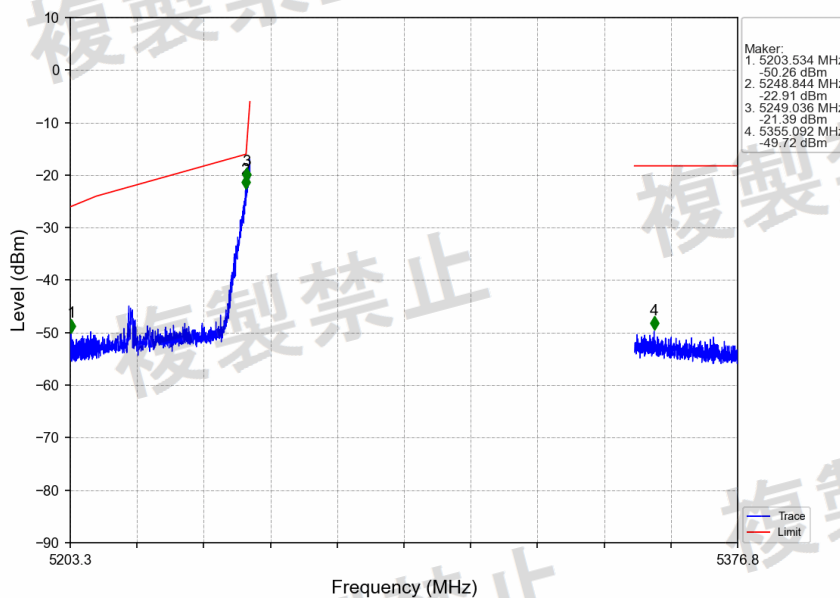
802.11ac(VHT80)_MCH_5290MHz_Ant2_NTNV
