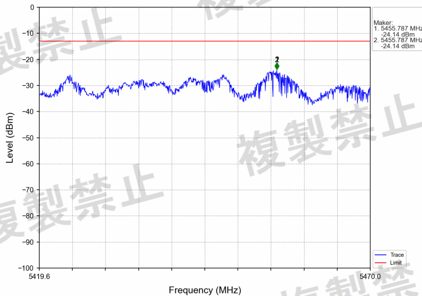
802.11ac(VHT160)_MCH_5570MHz_MIMO_NTNV
