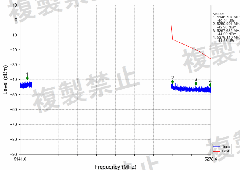
802.11ac(VHT40)_LCH_5190MHz_Ant2_NTNV
