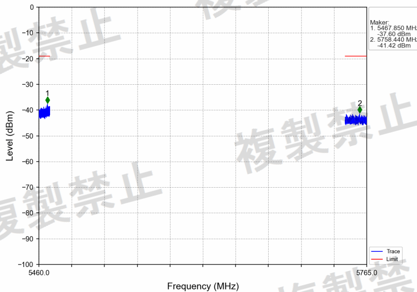
802.11ac(VHT20)_LCH_5500MHz_Ant2_NTNV
