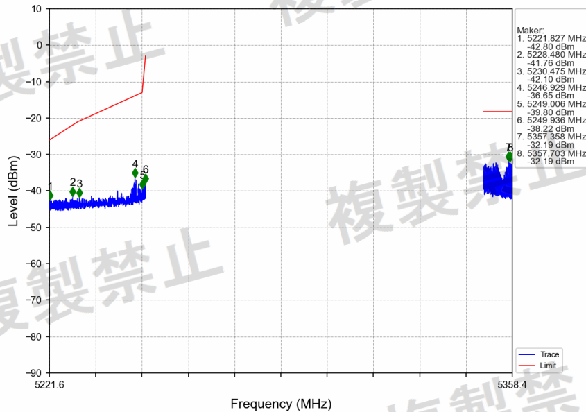
802.11ax(HEW40)_HCH_5310MHz_RU484_Left_MIMO_NTNV
