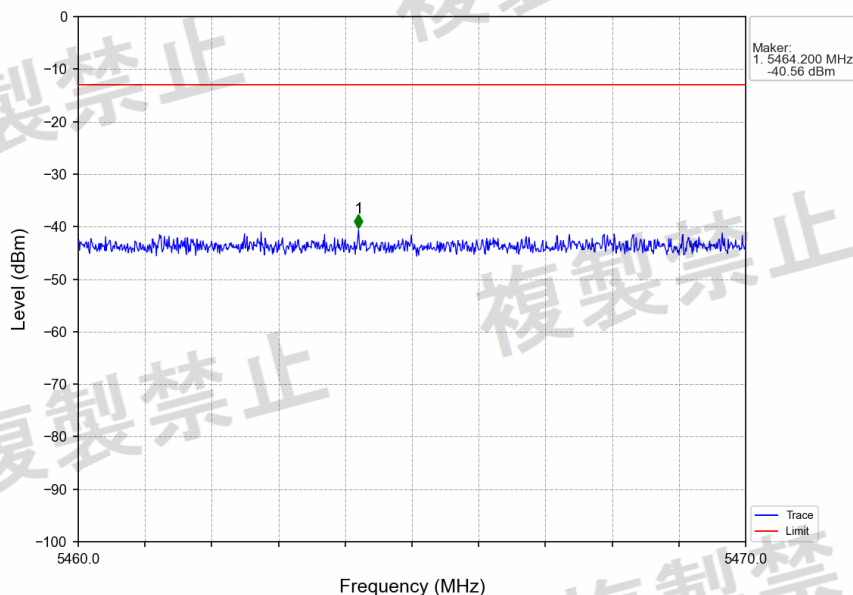
802.11ax(HEW40)_HHCH_5710MHz_RU484_Left_Ant2_NTNV
