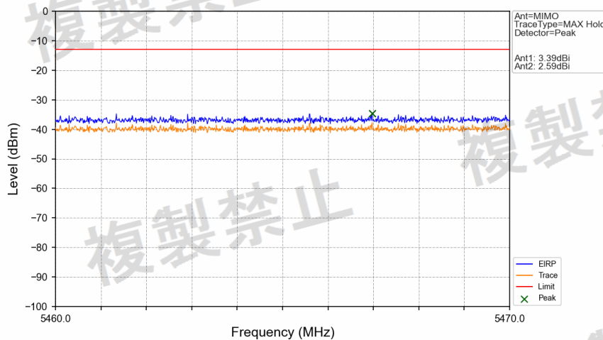
802.11n(HT40)_MCH_5590MHz_MIMO_NTNV
