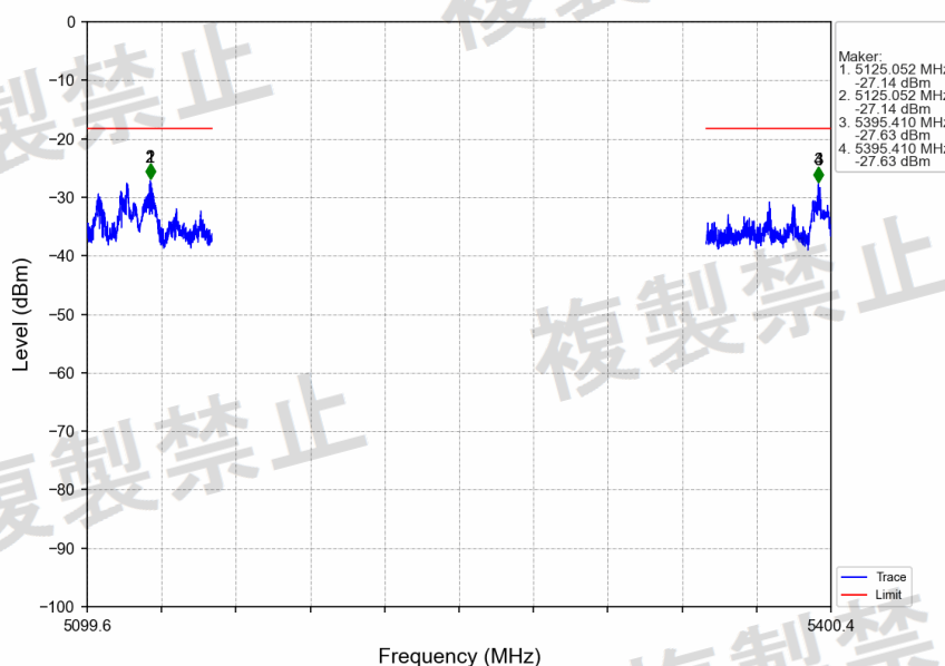
802.11ac(VHT160)_MCH_5250MHz_MIMO_NTNV
