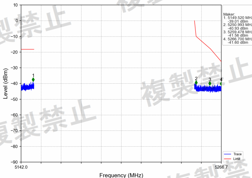
802.11ac(VHT20)_LCH_5180MHz_Ant2_NTNV
