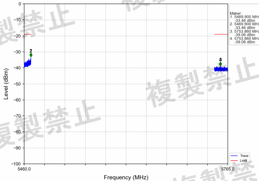
802.11ax(HEW20)_LCH_5500MHz_RU242_Left_MIMO_NTNV
