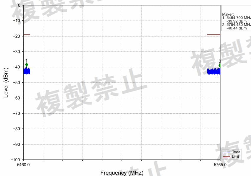
802.11ac(VHT20)_MCH_5600MHz_Ant2_NTNV
