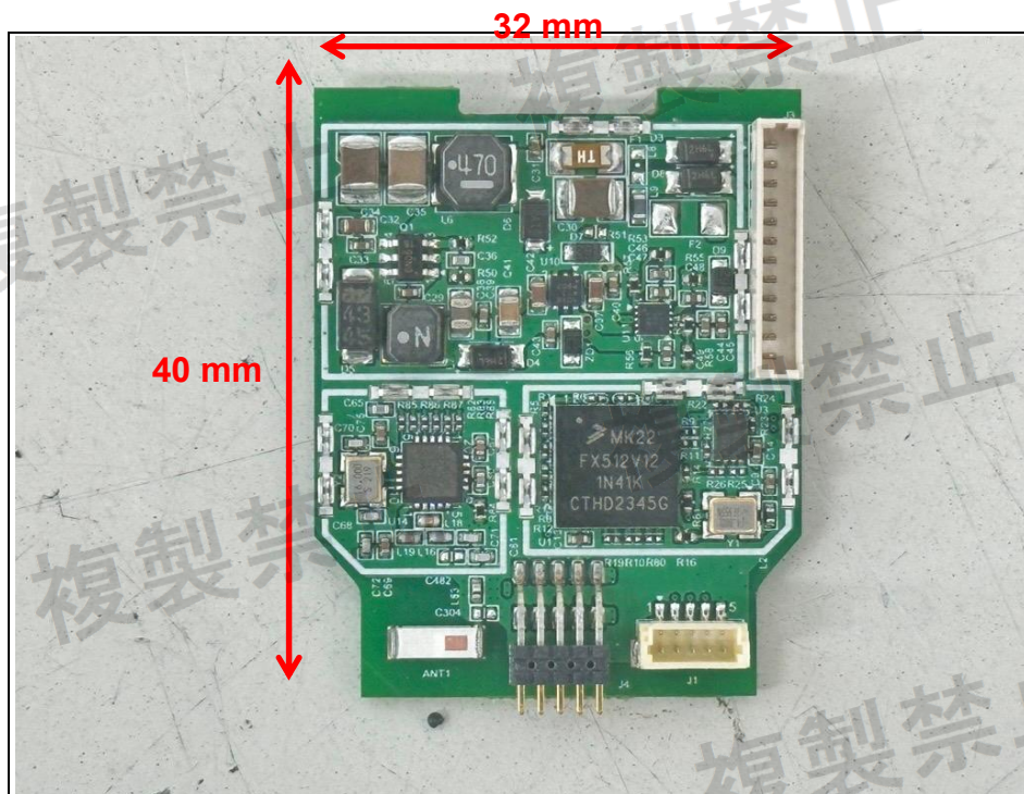
Top view of Main PCB
