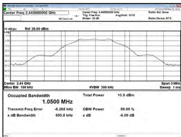
Modulation Type: GFSK(1Mbps) CH19
