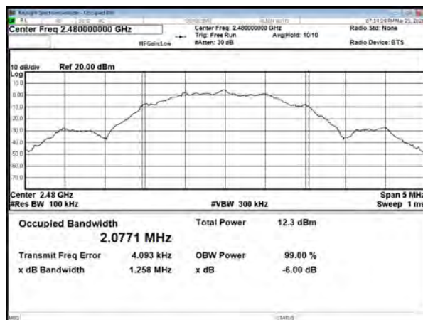
Modulation Type: GFSK(2Mbps) CH39
