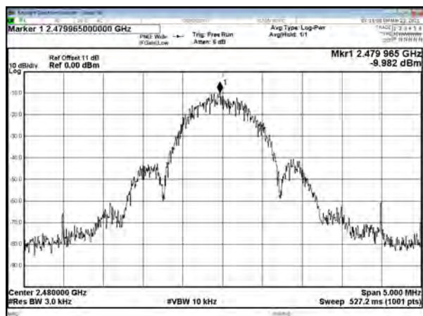
Modulation Type: GFSK(1Mbps) CH39
