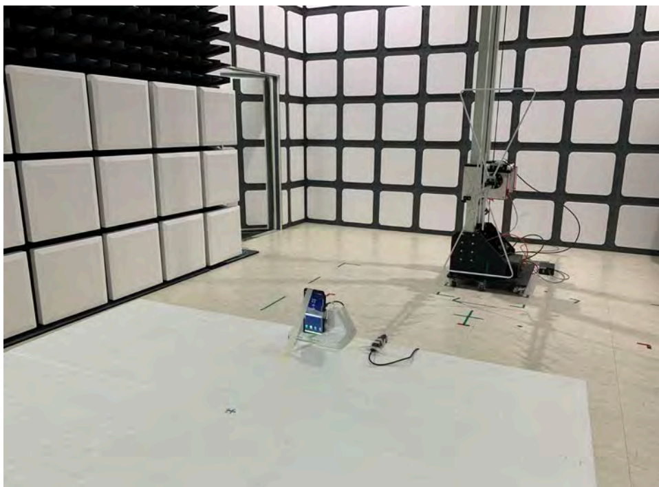
30 MHz ~ 1 GHz _ Rear View
