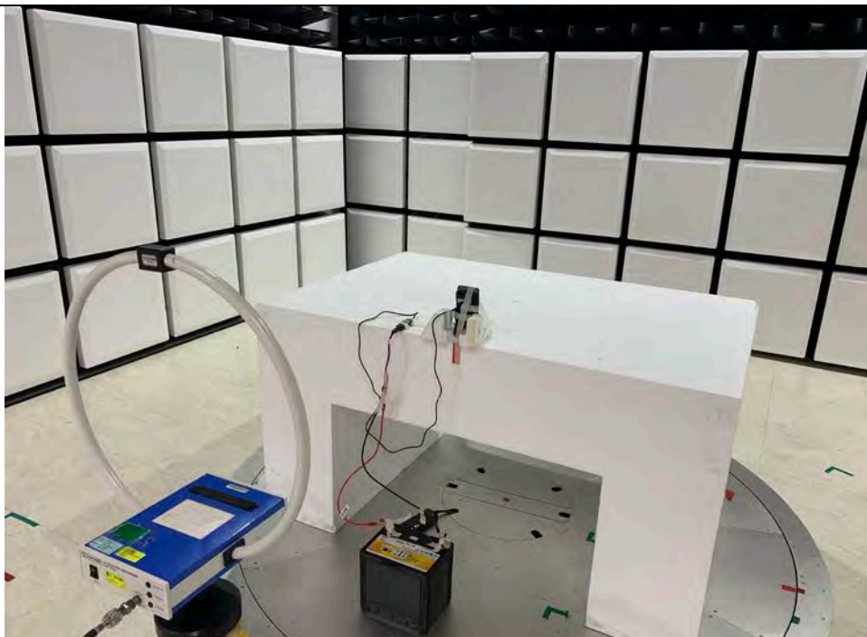
9 kHz ~ 30 MHz _ Rear View
