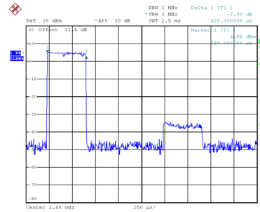
CH78-2DH1
