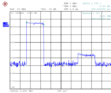
CH39-2DH1
