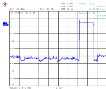
CH39-2DH5
