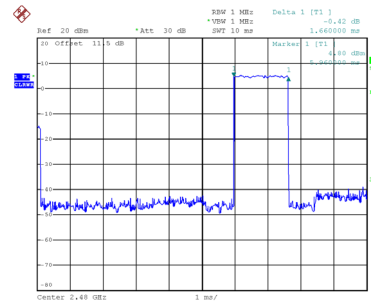
CH78-2DH3
