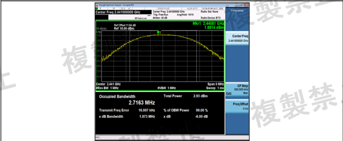
NTNV-2DH5-Ant1-2441-PASS
