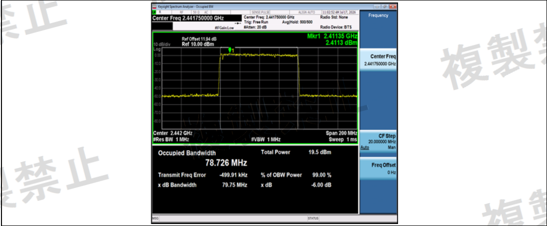
NTNV-3DH5-Ant1-Hop-PASS
