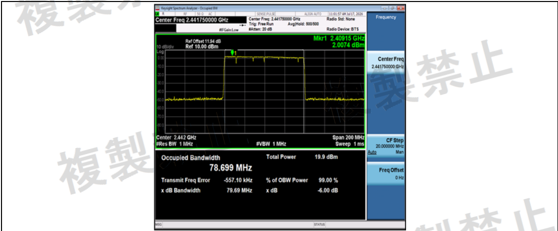
NTNV-DH5-Ant1-Hop-PASS
