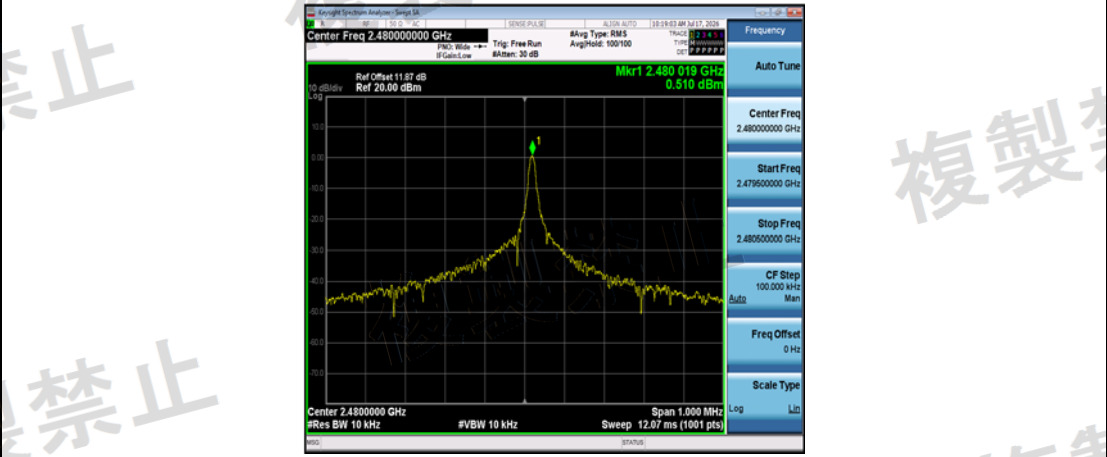
NTNV-2DH5-Ant1-2480-PASS
