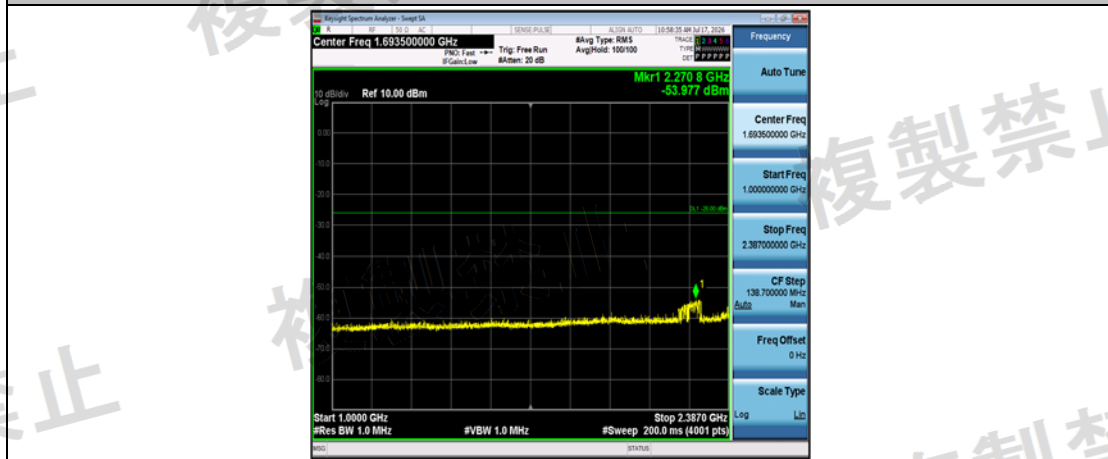
NTNV-3DH5-Ant1-Hop-1000~2387-PASS
