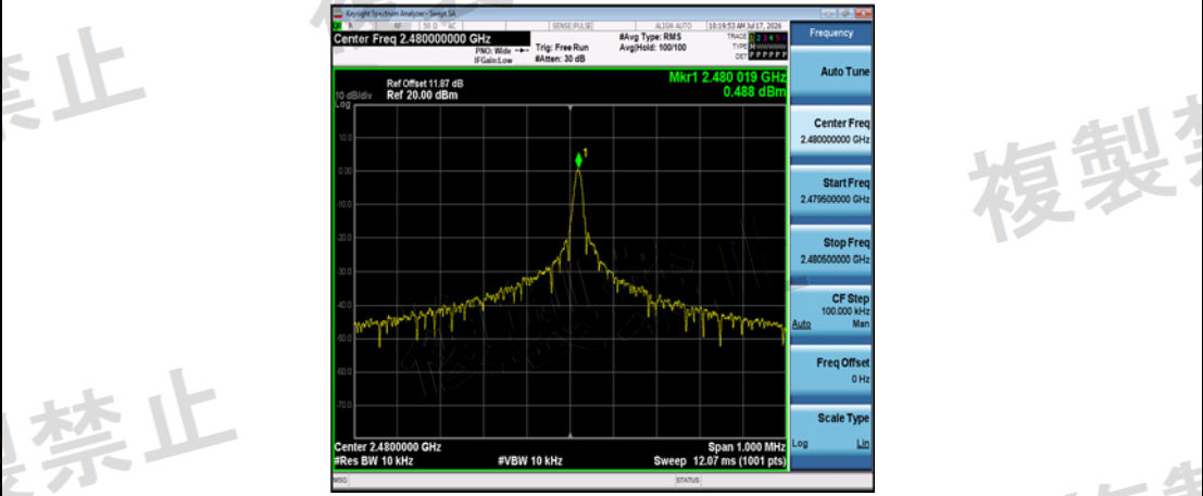
NTNV-3DH5-Ant1-2480-PASS
