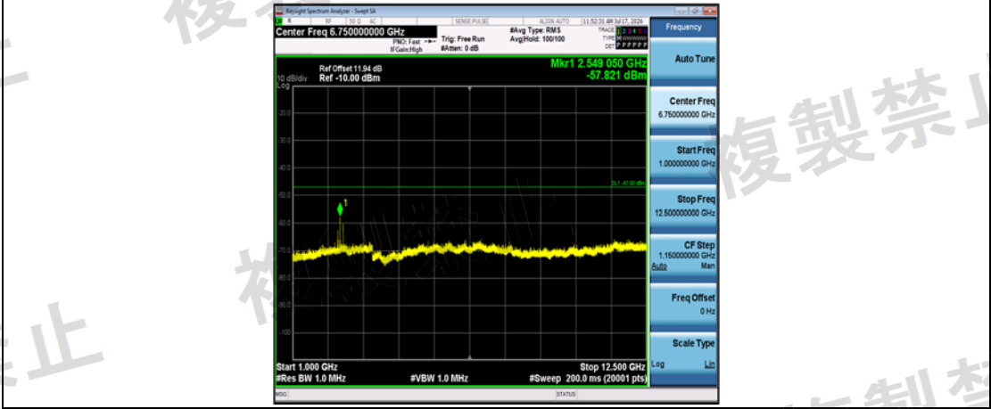
NTVN-3DH5-Ant1-2441-1000~12500-PASS
