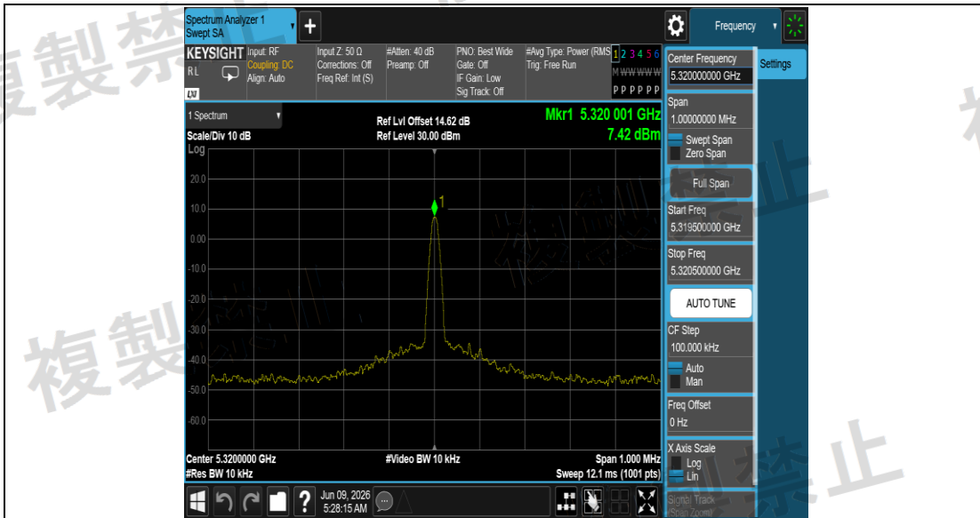
NTNV_11N20SISO_Ant1_5320
