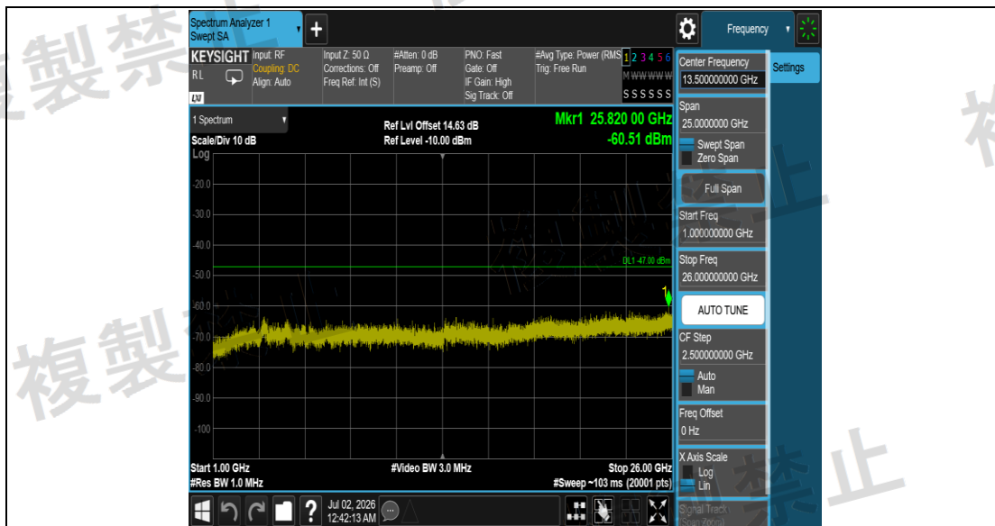
NTNV_11A_Ant1_5700_1000~26000
