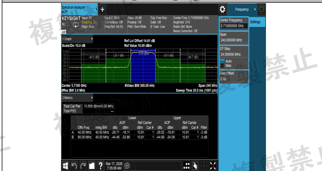
NTNV_11N40SISO_Ant1_5710
