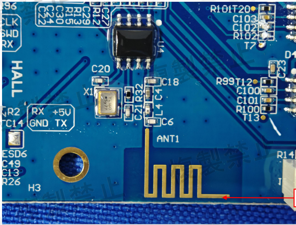
SRD 2.4G Antenna
