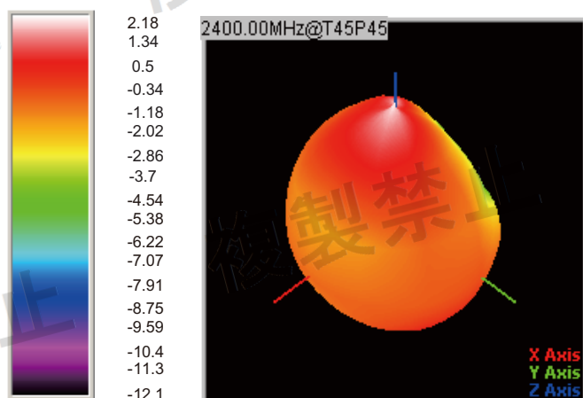
◎ 3D Gain Pattern (2400.0 MHz)
