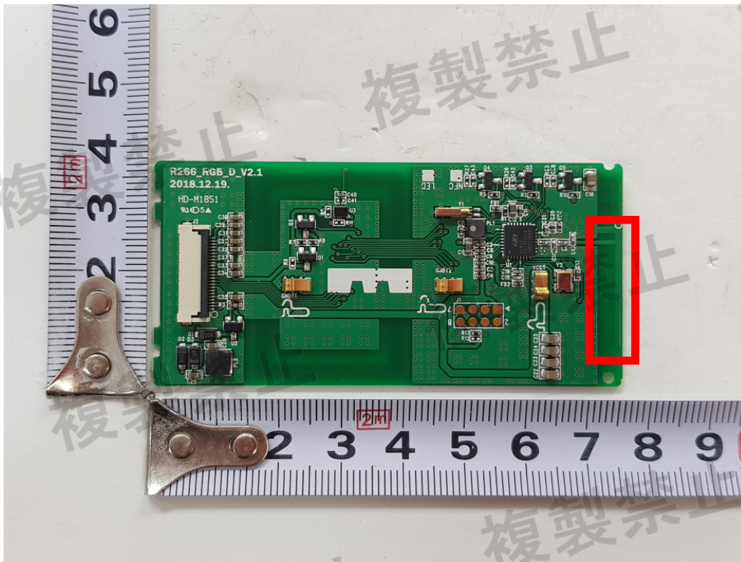
Zigbee Antenna
