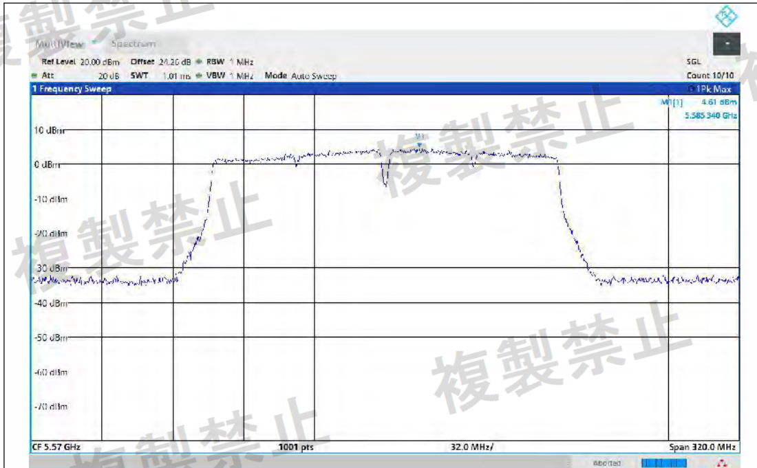
NTNV-11AC160MIMO-Ant2-5570-TPC_H-PASS
