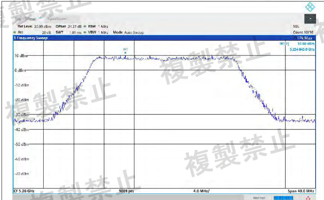
NTNV-11BE20MIMO-Ant2-5260-TPC_H-PASS
