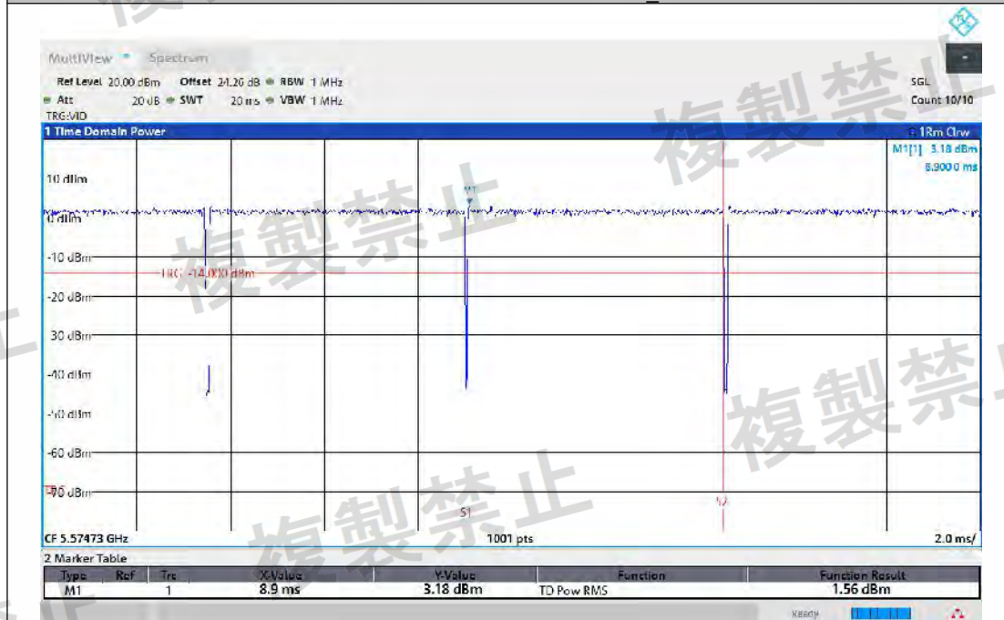
NTNV-11AX20MIMO-Ant1-5580-TPC_H-PASS
