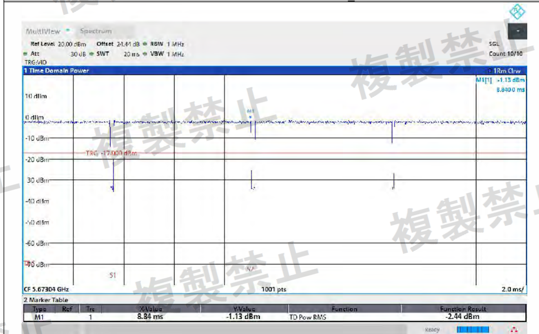
NTNV-11BE40MIMO-Ant1-5670-TPC_L-PASS
