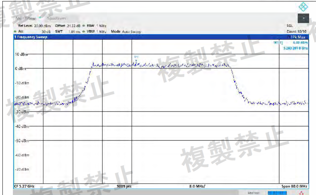
NTNV-11AX40MIMO-Ant1-5270-TPC_L-PASS
