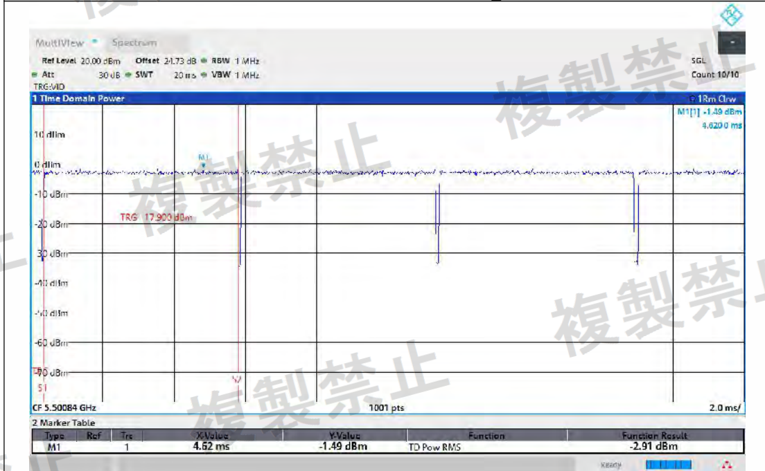
NTNV-11BE20MIMO-Ant2-5500-TPC_L-PASS
