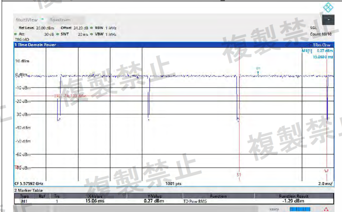
NTNV-11BE20MIMO-Ant2-5580-TPC_L-PASS
