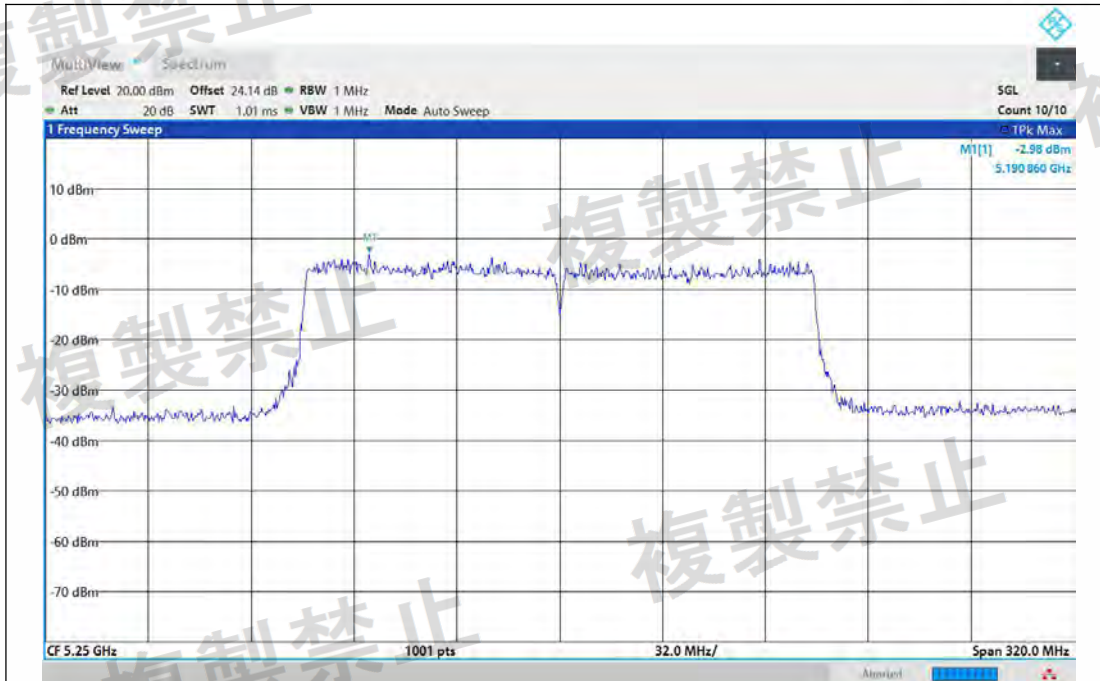
NTNV-11AX160MIMO-Ant2-5250-TPC_L-PASS
