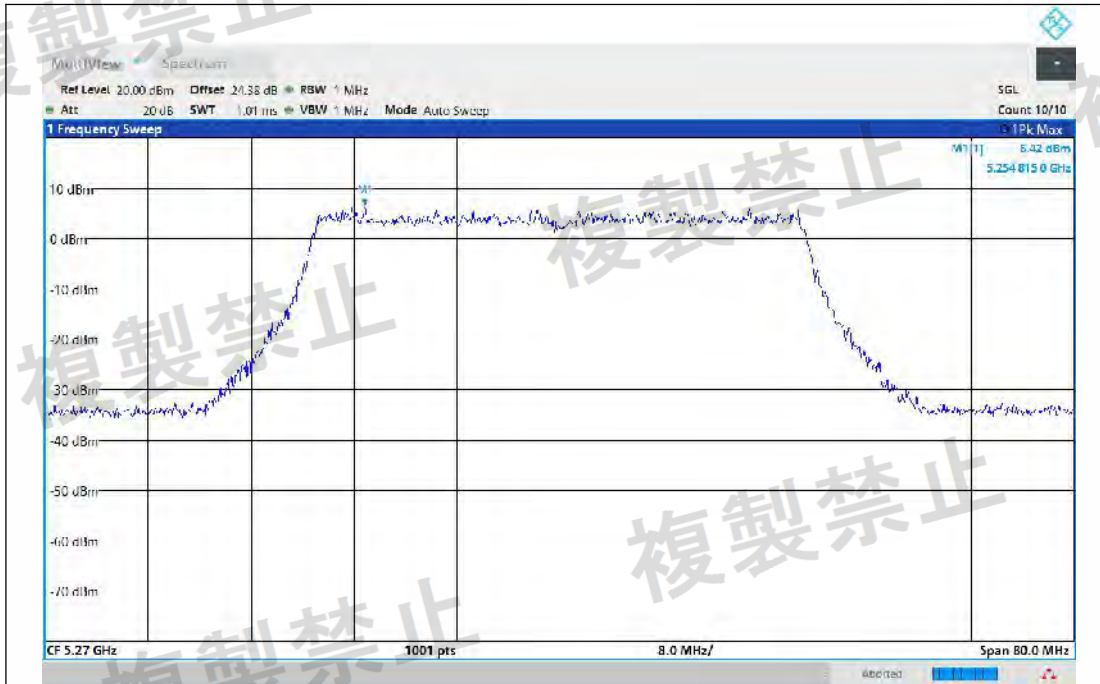
NTNV-11BE40MIMO-Ant2-5270-TPC_H-PASS
