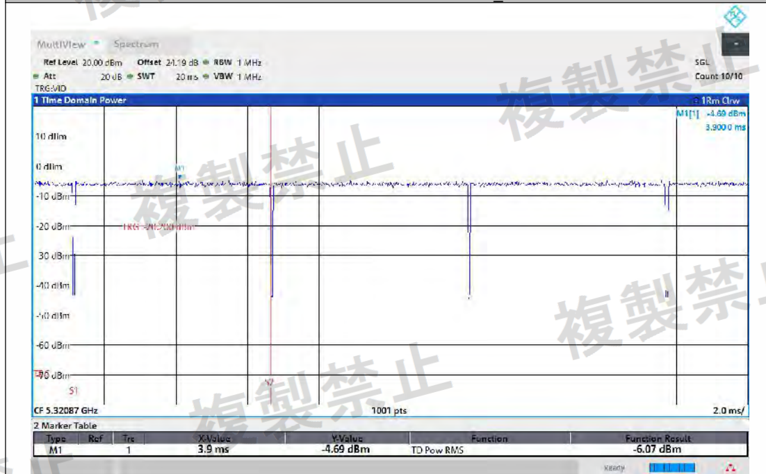
NTNV-11AC40MIMO-Ant2-5310-TPC_H-PASS
