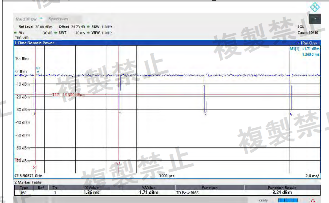
NTNV-11AX20MIMO-Ant2-5500-TPC_L-PASS
