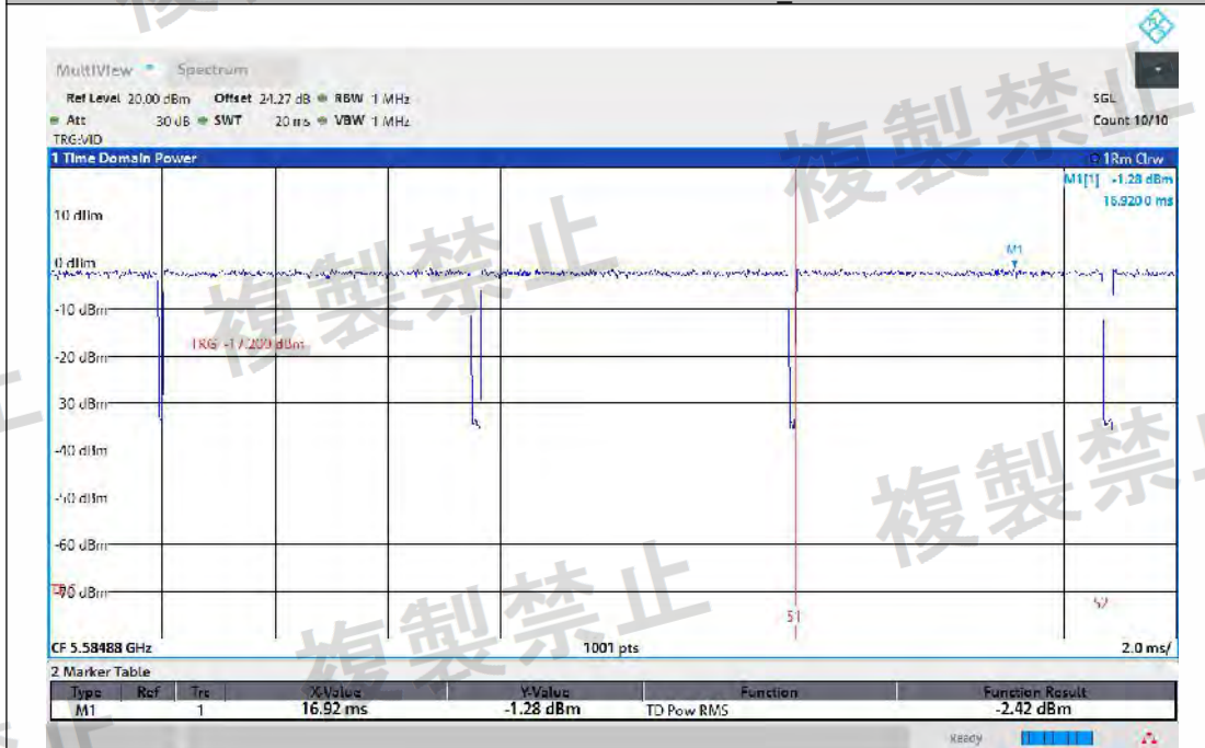
NTNV-11AX20MIMO-Ant1-5580-TPC_L-PASS
