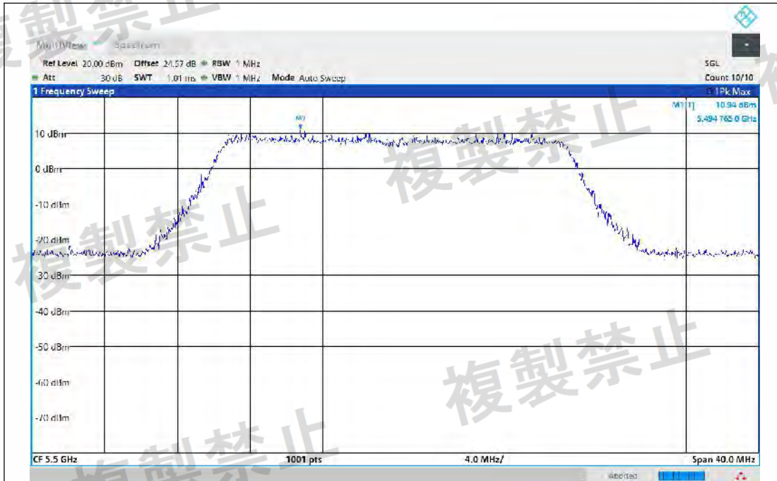
NTNV-11BE20MIMO-Ant1-5500-TPC_L-PASS
