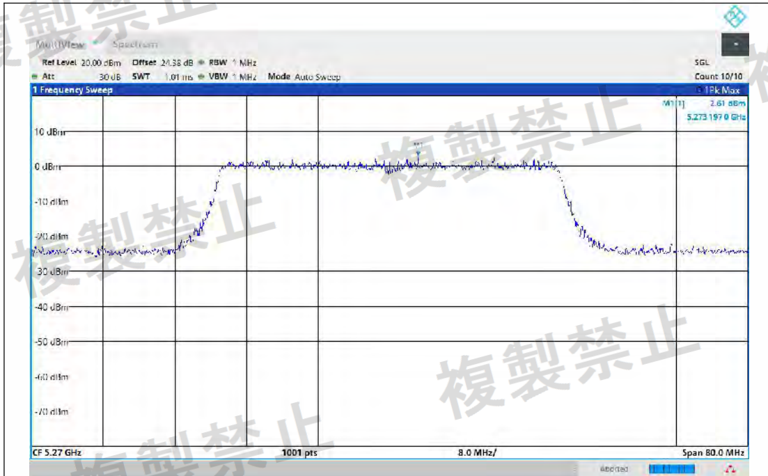
NTNV-11AX40MIMO-Ant2-5270-TPC_L-PASS
