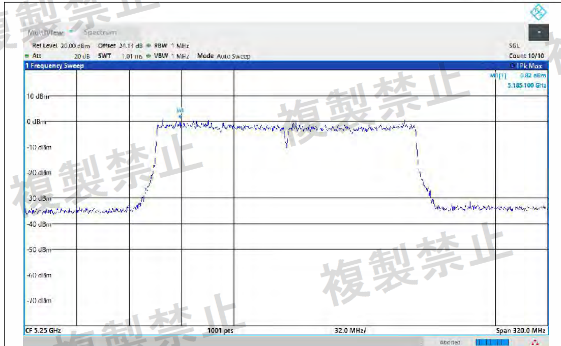
NTNV-11BE160MIMO-Ant2-5250-TPC_H-PASS
