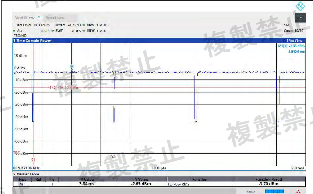
NTNV-11AX40MIMO-Ant1-5270-TPC_H-PASS
