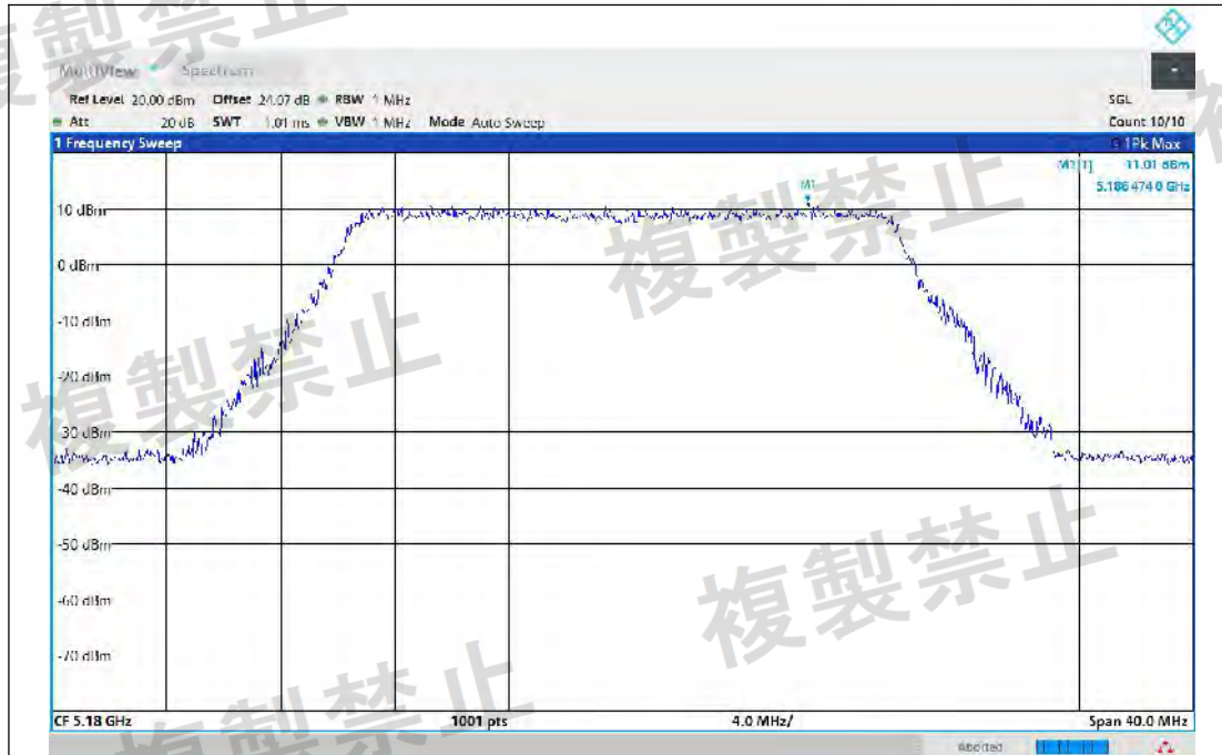
NTNV-11BE20MIMO-Ant1-5180-PASS
