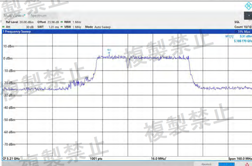
NTNV-11BE80MIMO-Ant2-5210-484+242_OFDMA-1-PASS
