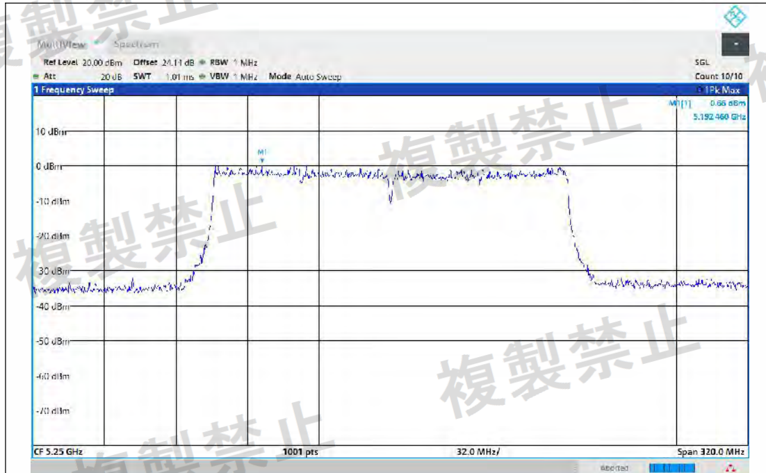
NTNV-11AX160MIMO-Ant2-5250-TPC_H-PASS
