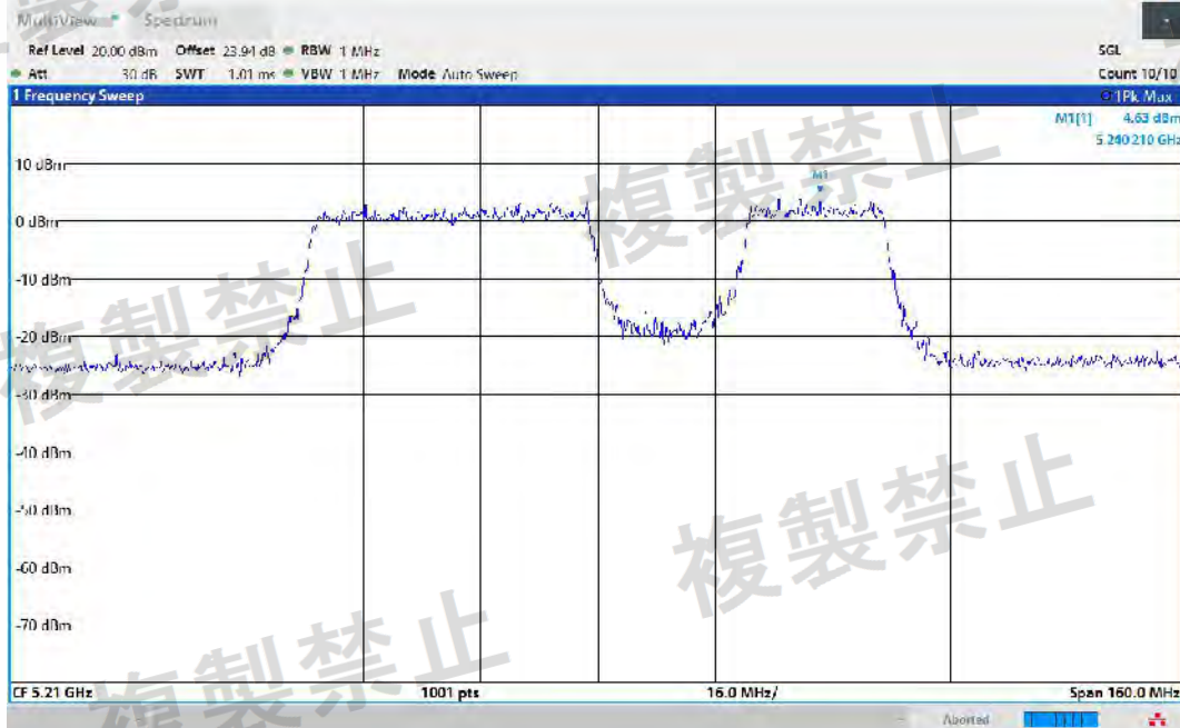
NTNV-11BE80MIMO-Ant1-5210-484+242_OFDMA-3-PASS
