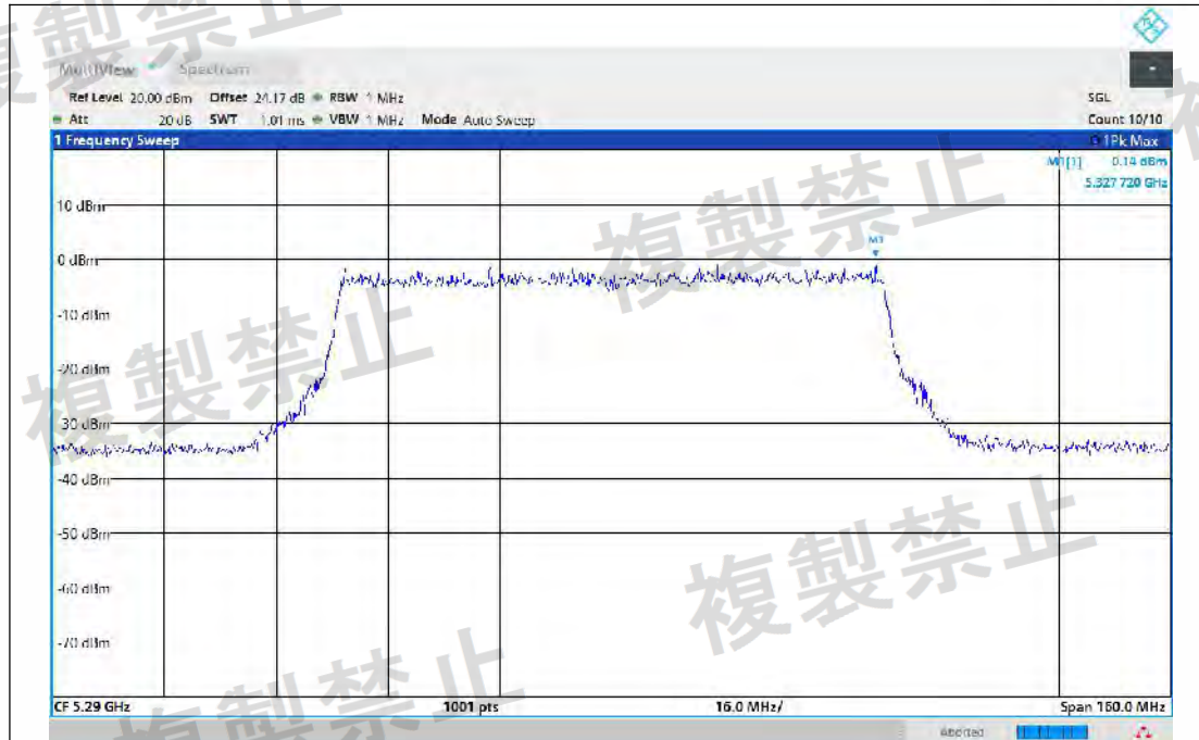
NTNV-11AX80MIMO-Ant2-5290-TPC_L-PASS
