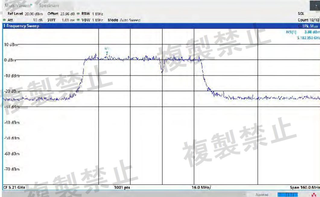
NTNV-11BE80MIMO-Ant2-5210-484+242_OFDMA-4-PASS
