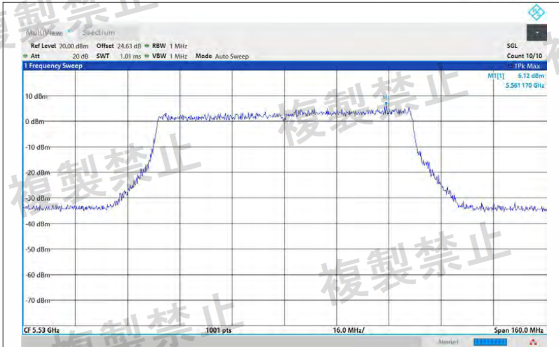
NTNV-11AX80MIMO-Ant2-5530-TPC_L-PASS
