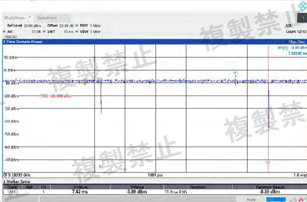
NTNV-11BE80MIMO-Ant2-5210-484+242_OFDMA-4-PASS
