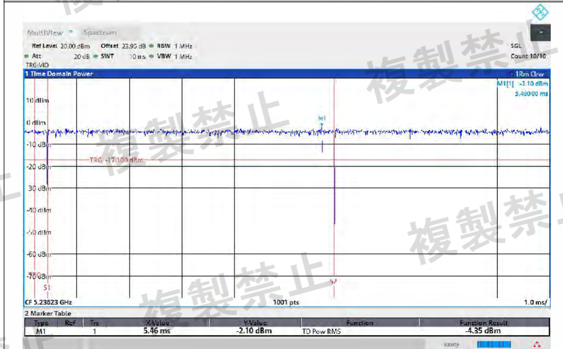
NTNV-11AC40MIMO-Ant1-5230-PASS
