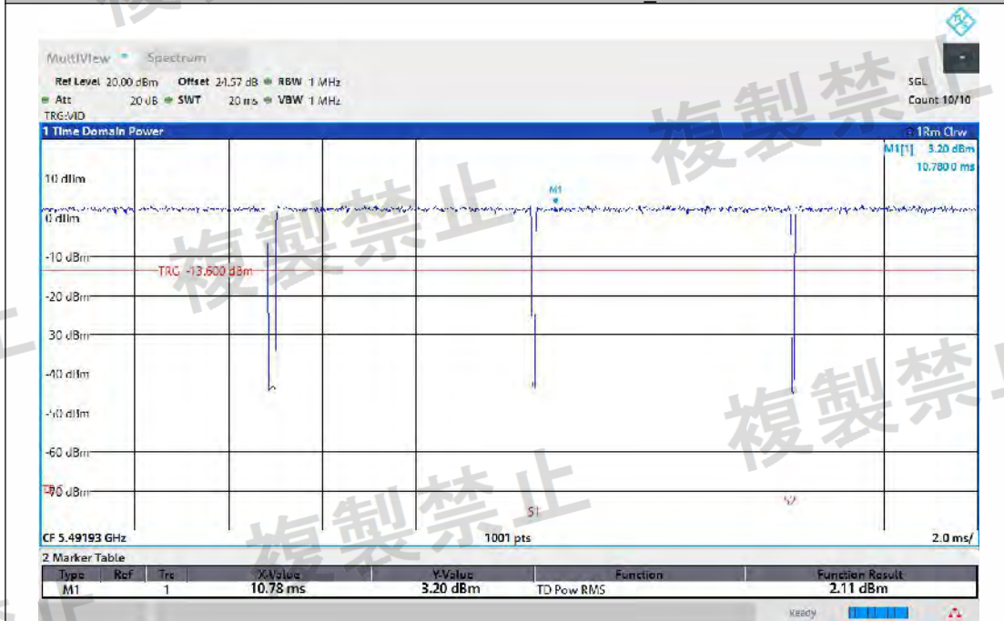
NTNV-11AX20MIMO-Ant1-5500-TPC_H-PASS
